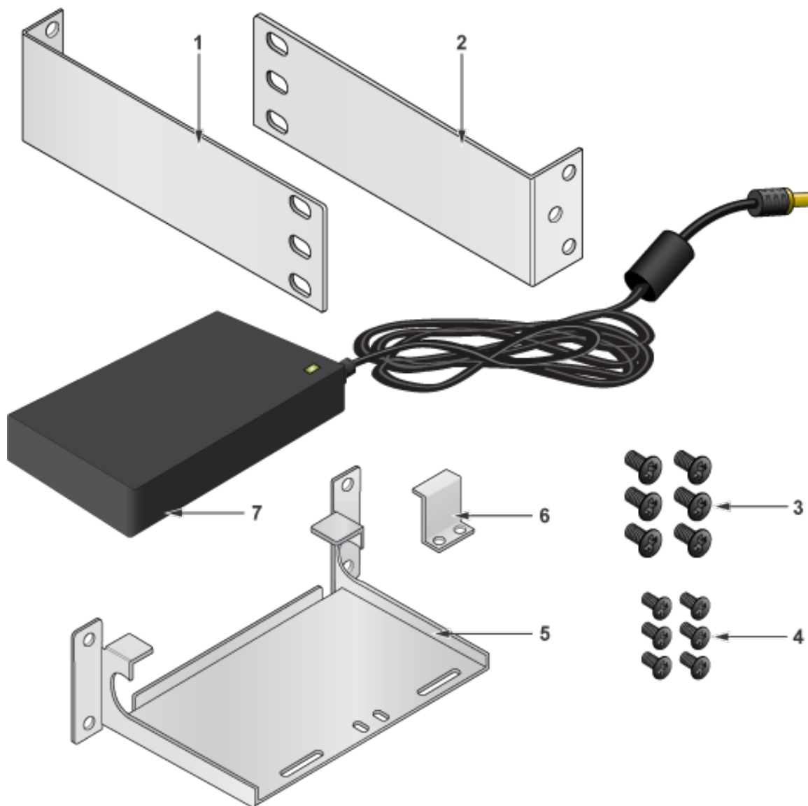
Figure 1: CCA-ETM-Q6EWL Mounting Parts Kit
