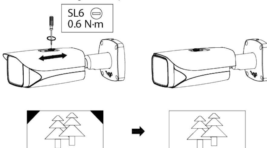
Figure 3-7 Adjust sunshield
