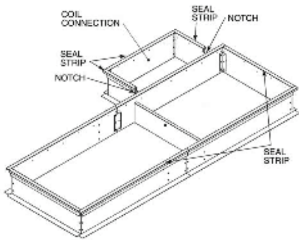
Fig. 62 — Installing Seal Strip
