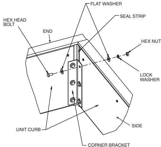
Fig. 21 — Corner Bracket
