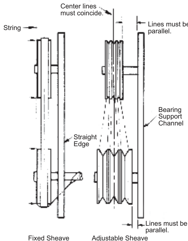
Fig. 55 — Determining Sheave-Shaft Alignment
