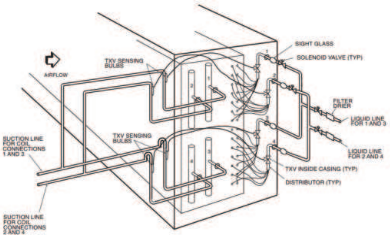
Fig. 111 — Row-Split Coil Manifolding (Typical)
