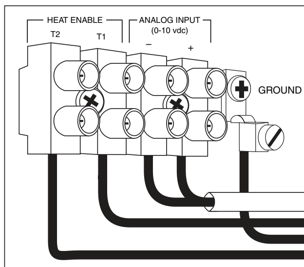
Fig. 148 — Gas-Fired Duct System Furnace Typical Wiring Diagram
