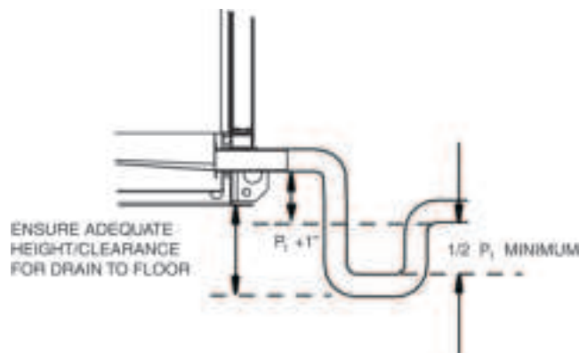
Fig. 113 — Condensate Drain, Draw-Thru Trapping (All Sizes)
