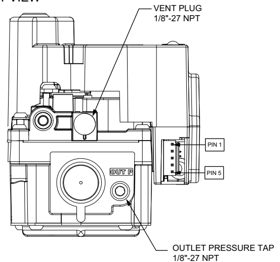
RIGHT VIEW
