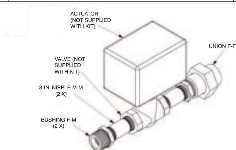
Fig. 87 — Valve Fitting Kits
