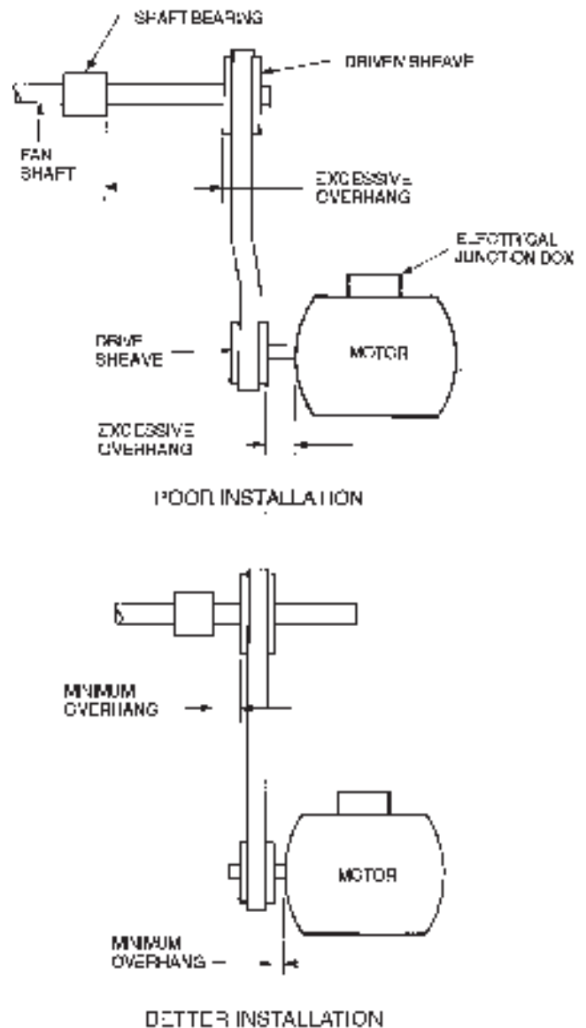
Fig. 54 — Determining Sheave-Shaft Overhang
