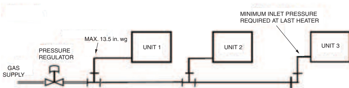
Fig. 154 — Inlet Pressure for Multiple Heaters
