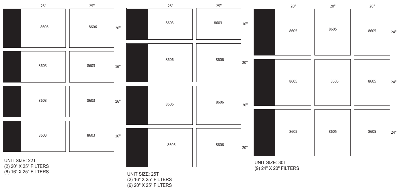
Fig. 213 — Flat Filter Arrangement — 2-in. or 4-in. (cont)
