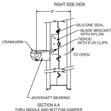
Fig. 44 — Face and Bypass Section Detail
