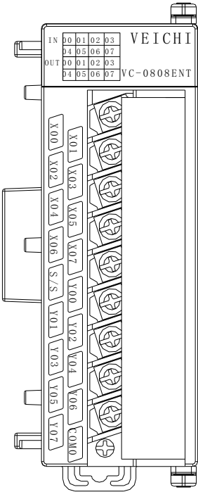
Figure 1-4 VC-0808ENT appearance and terminal diagram
