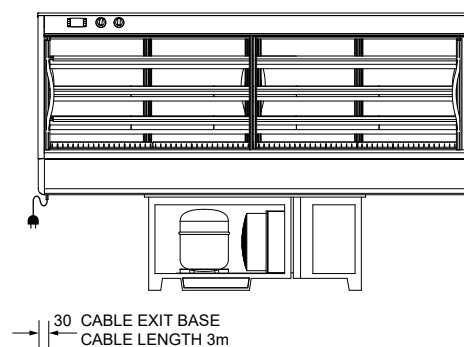
REAR ELEVATION
