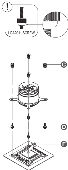
Intel LGA 2011/2066
