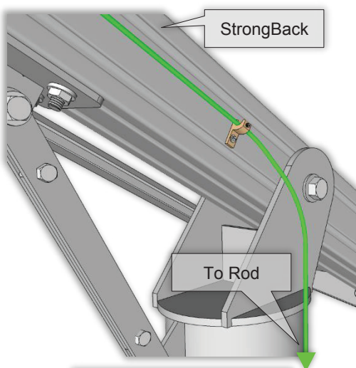
StrongBack Ground Lug
