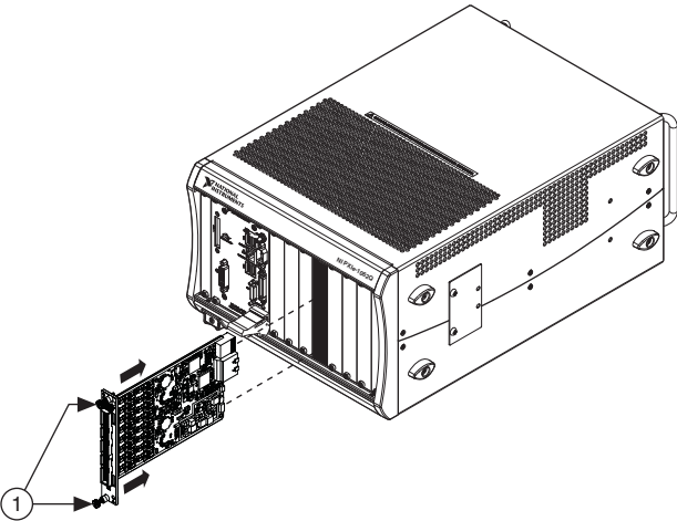
Figure 2. Installing PXIe-4302/4303 Modules
