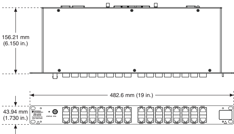
Figure 10. RM-4302 Dimensions
