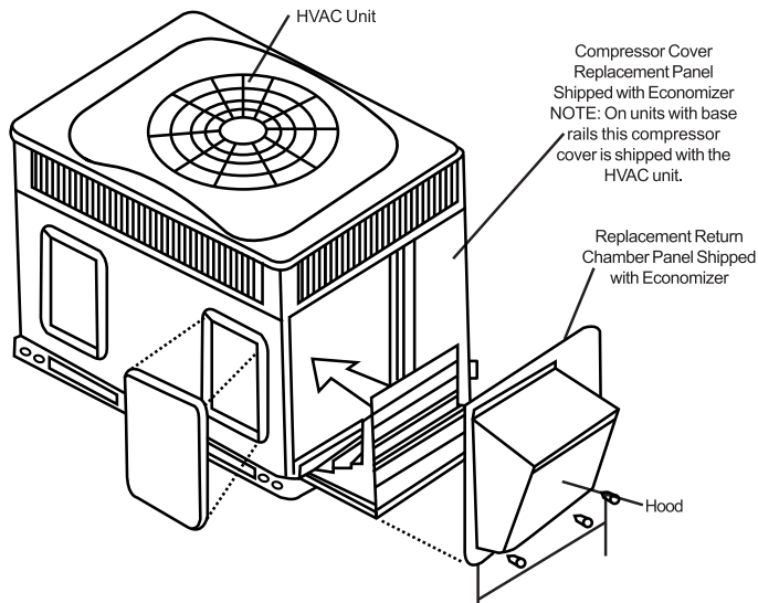
Vertical Economizer
