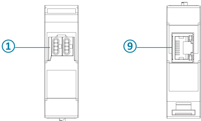
DIN-KXI Top and Bottom View
