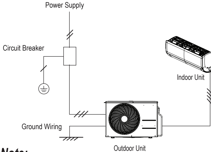
Figure 22: LS090HSV5 and LS120HSV5 General Power / Communications System Schematic.
