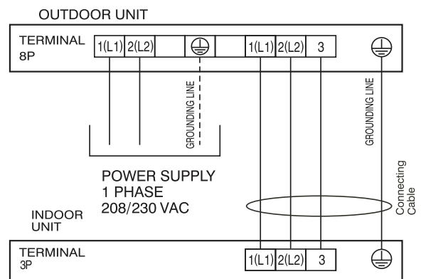
Figure 25: LS181HSV5 System Electrical Connections.
