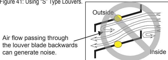
Figure 41: Using “S” Type Louvers.
