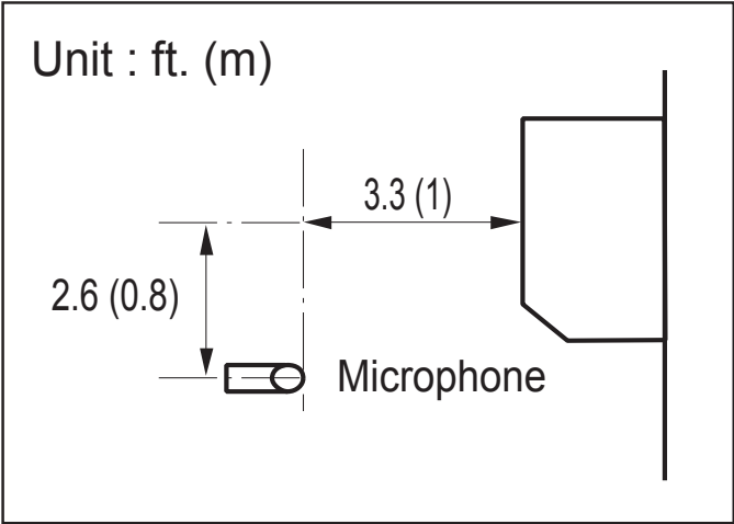
Figure 9: High Efficiency Indoor Unit Sound Level Measurement.
