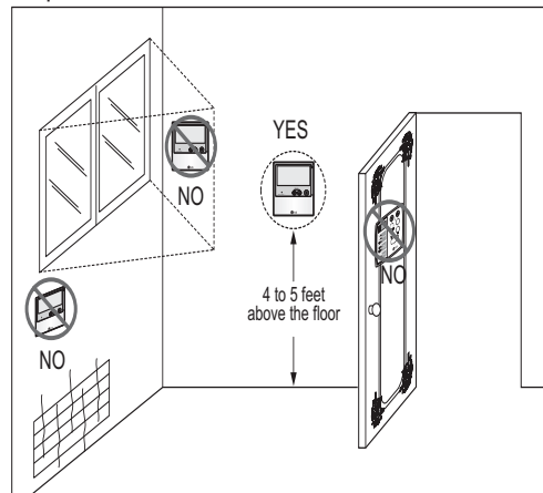
Figure 29: Proper Location for the Wired Controller.
