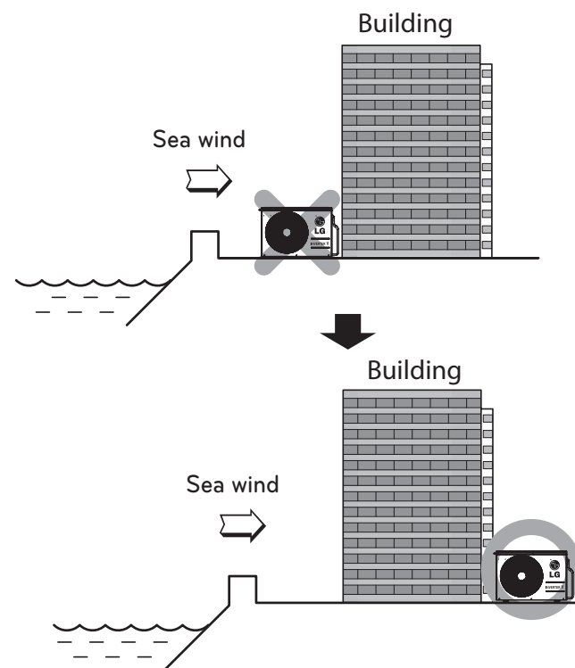
Figure 38: Placement Using Building as Shield.
