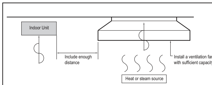
Figure 34: Installing Near a Heat or Steam Source.
