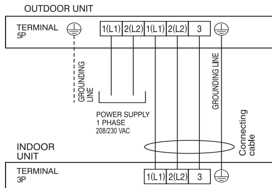
Figure 24: LS090-120HSV5 System Electrical Connections.
