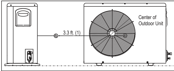
Figure 12: High Efficiency Outdoor Unit Sound Level Measurement.
