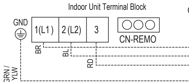
Figure 27: Wired Controller Connection on the Indoor Unit Terminal Block.
