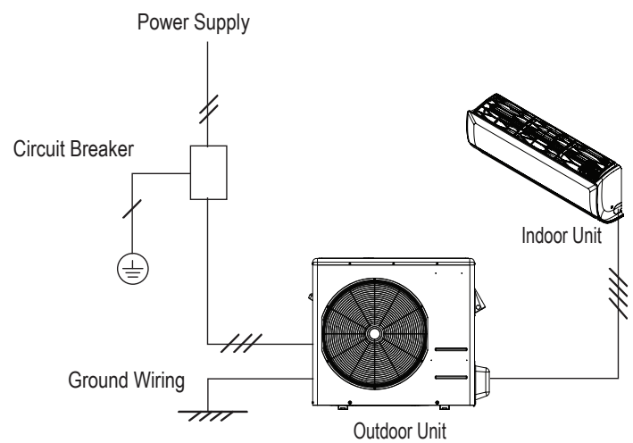
Figure 23: LS181HSV5 General Power / Communications System Schematic.
