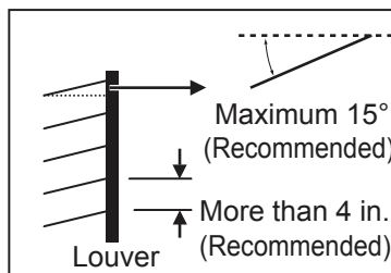
Figure 40: Louver Recommendations.
