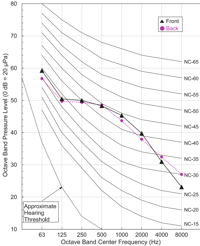
Figure 15: LSU181HSV5 Cooling Sound Pressure Level Diagram.
