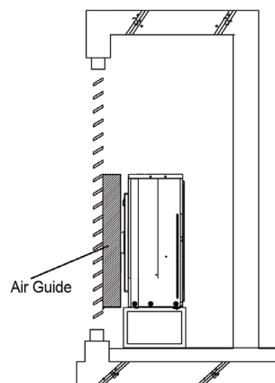
Figure 43: Example of Installing Outdoor Unit Indoors.
