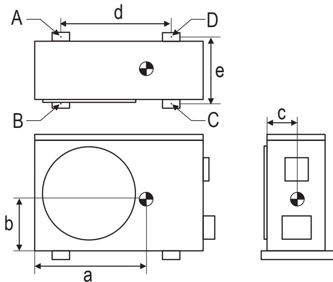
Figure 6: LSU090-120-181HSV5 Outdoor Unit Corner Weight and Center of Gravity Dimensions.
