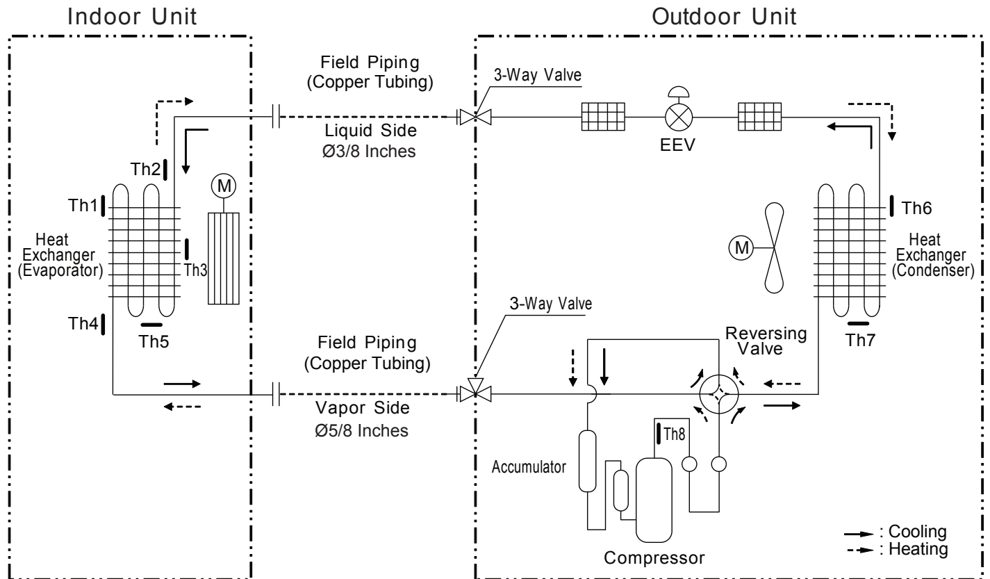
Figure 18: Refrigerant Flow Diagram for LSN / LSU181HSV5 units.
