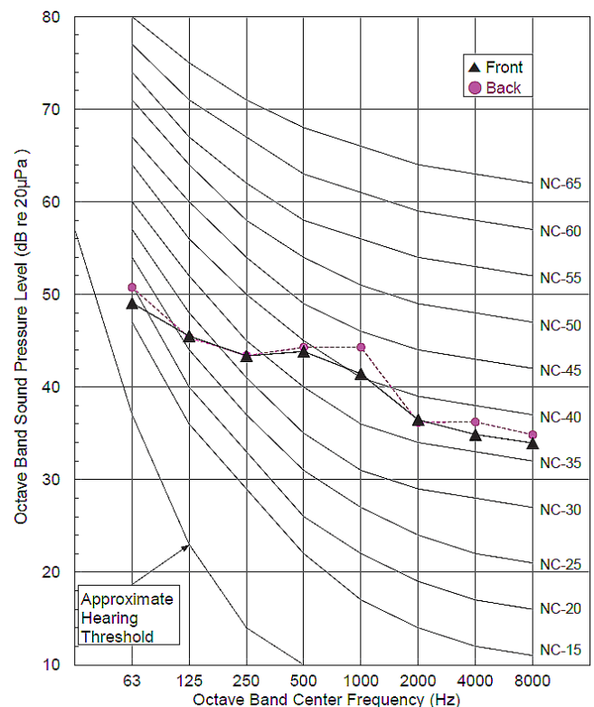
Figure 14: LSU090/120HSV5 Heating Sound Pressure Level Diagram.
