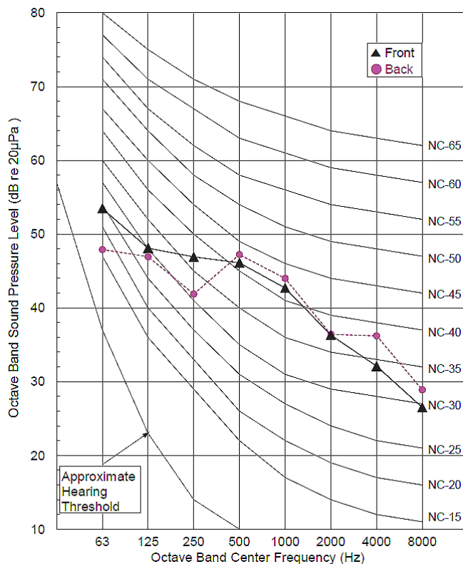
Figure 13: LSU090/120HSV5 Cooling Sound Pressure Level Diagram.
