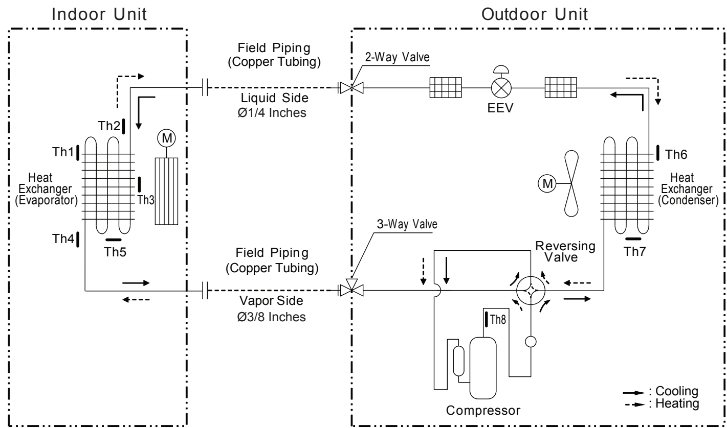
Figure 17: Refrigerant Flow Diagram for LSN / LSU090-120HSV5 units.
