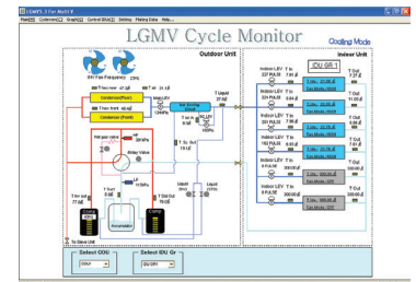
Figure 30: Sample Cycleview.
