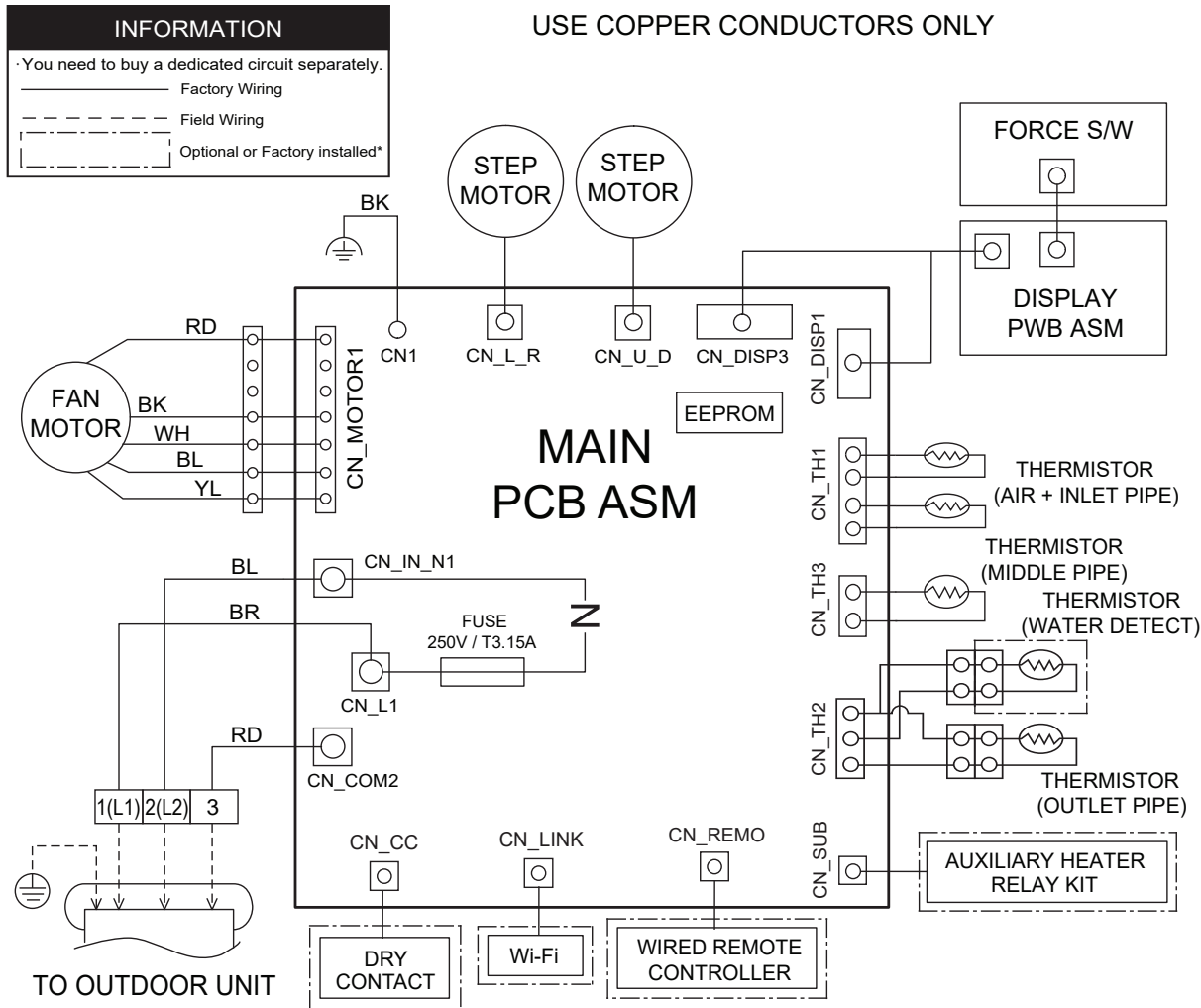
Figure 19: Wiring Diagram for LSN090HSV5, LSN120HSV5, LSN181HSV5 units.
