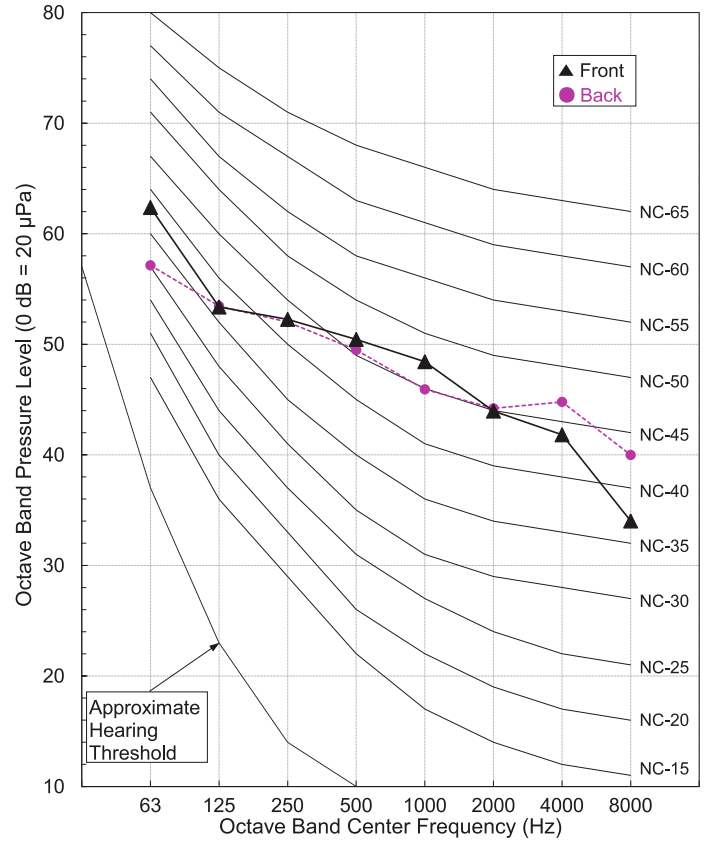
Figure 16: LSU181HSV5 Heating Sound Pressure Level Diagram.
