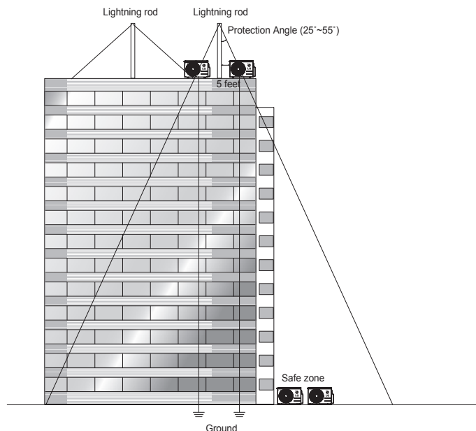
Figure 36: Lightning Protection Diagram.
