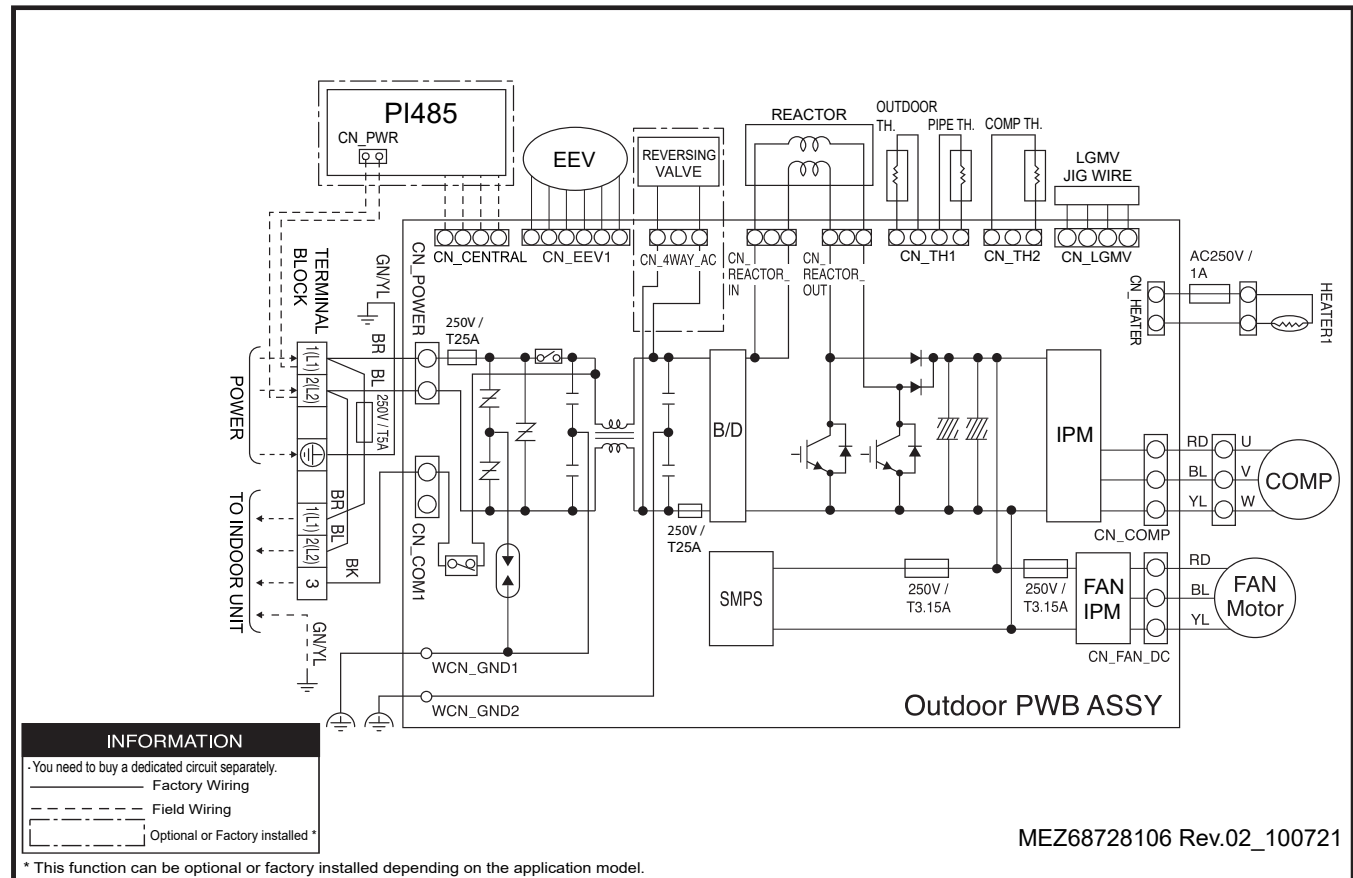
Figure 21: Wiring Diagram for LSU181HSV5 units.
