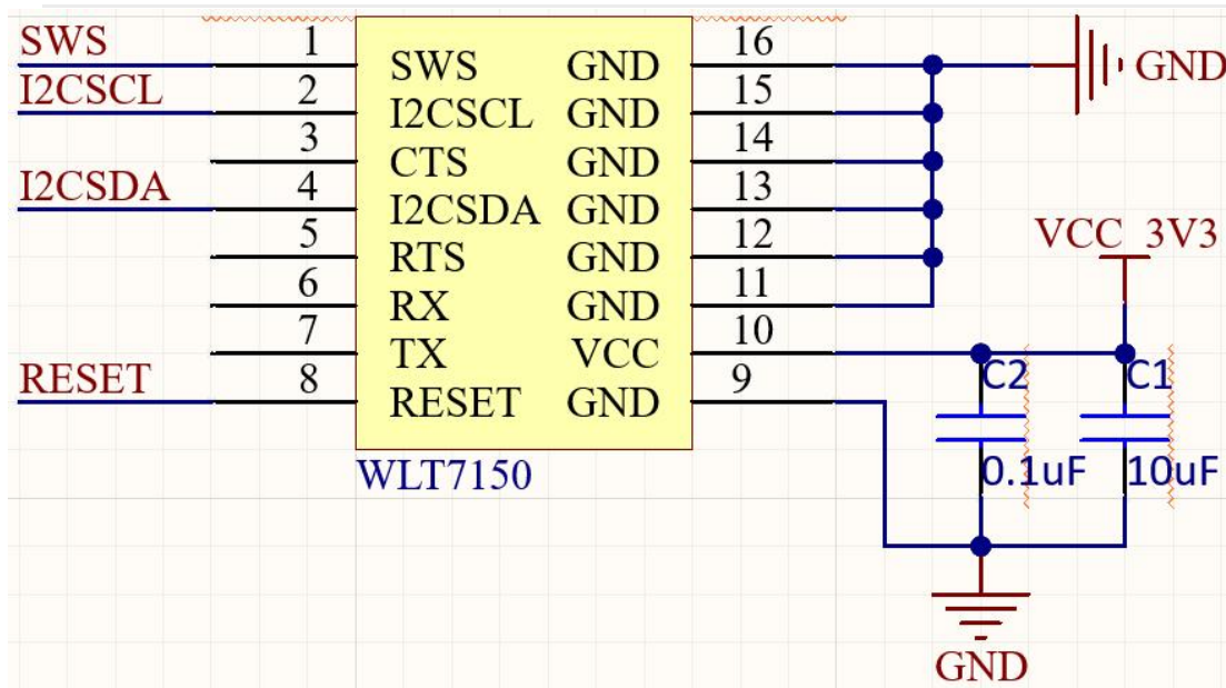
Figure 4-1: Reference schematic
