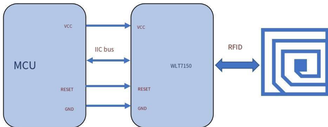
Figure 3-2: I2C communication
