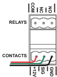
Figure 4. Contact Port for Voltage Source (e.g., Motion Sensor)
