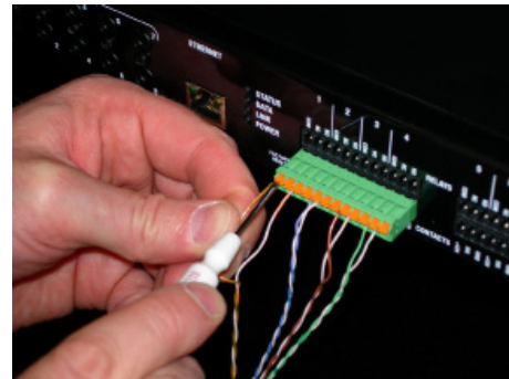
Figure 3. Connect to Terminal Block
