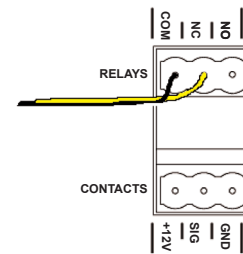
Figure 8. Relay Port, Normally Closed
