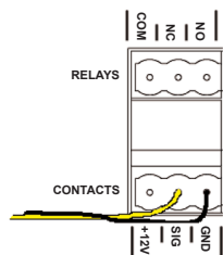
Figure 6. Contact for Self-Powered Voltage Source Device
