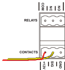
Figure 6. Contact for Self-Powered Voltage Source Device
