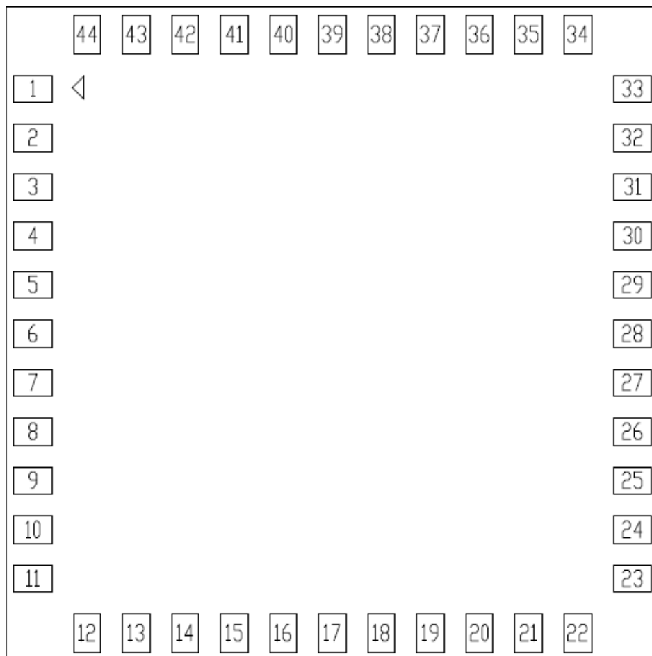
AW-HM610 Pin Map (Top View)
