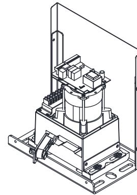
Releasing arm in torsion, wriggle 90 degrees gate operator will be in releasing state
