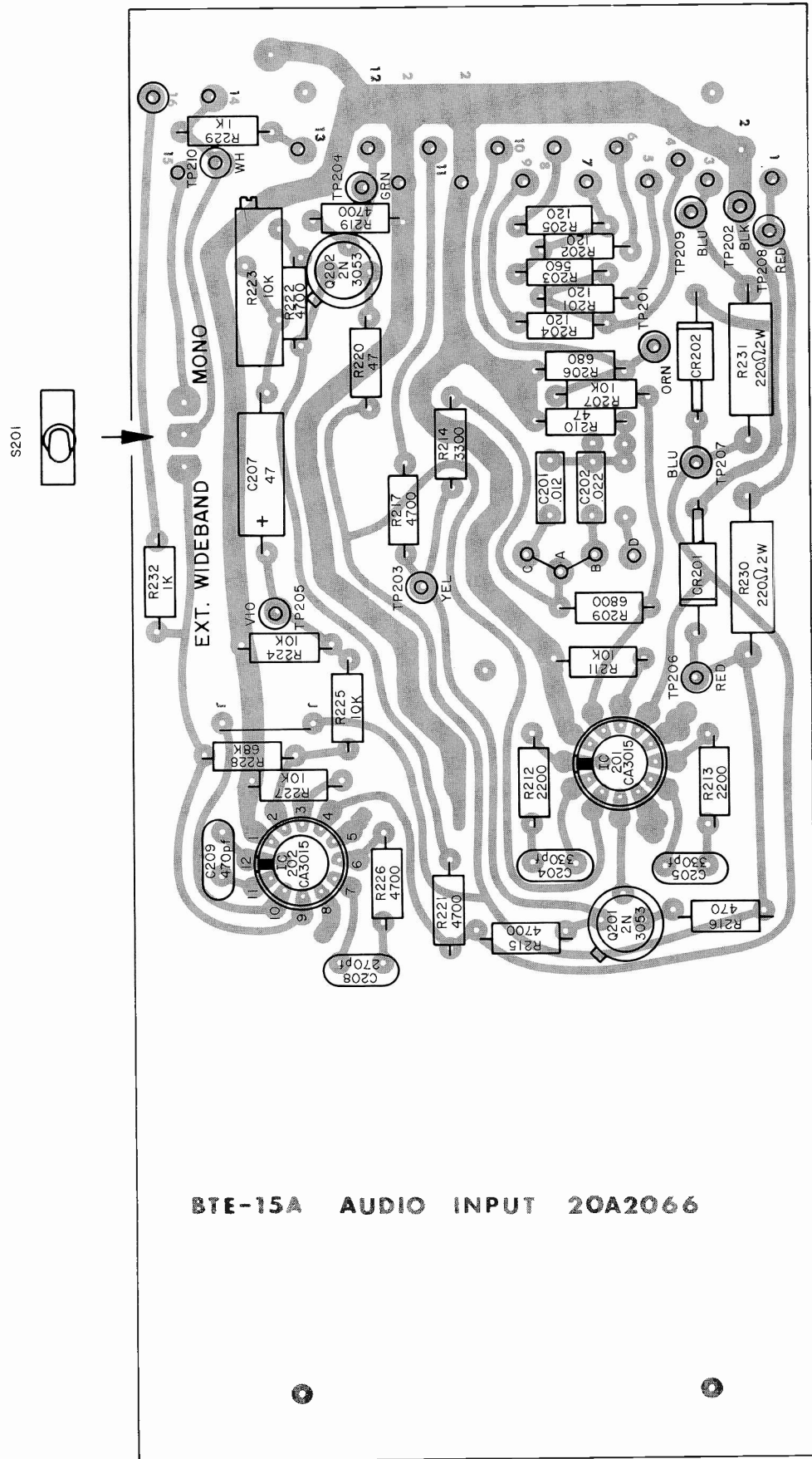
Figure 39. Monaural Audio Board, Parts Overlay, Bottom
