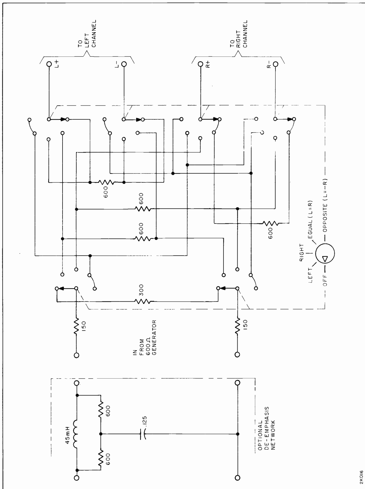
Figure 56. Test Fixture
