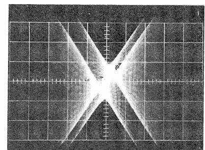
TP411 (white); Composite Output .1 V/cm, 50 \mu sec/cm Sync: Ext. audio generator Photo to left expanded to show waveform when pilot phase is misadjusted.
