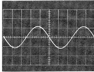
*TP409 (yellow); 17 kHz Filter Input 1 V/cm, .5 ms/cm Sync: Ext. audio generator
