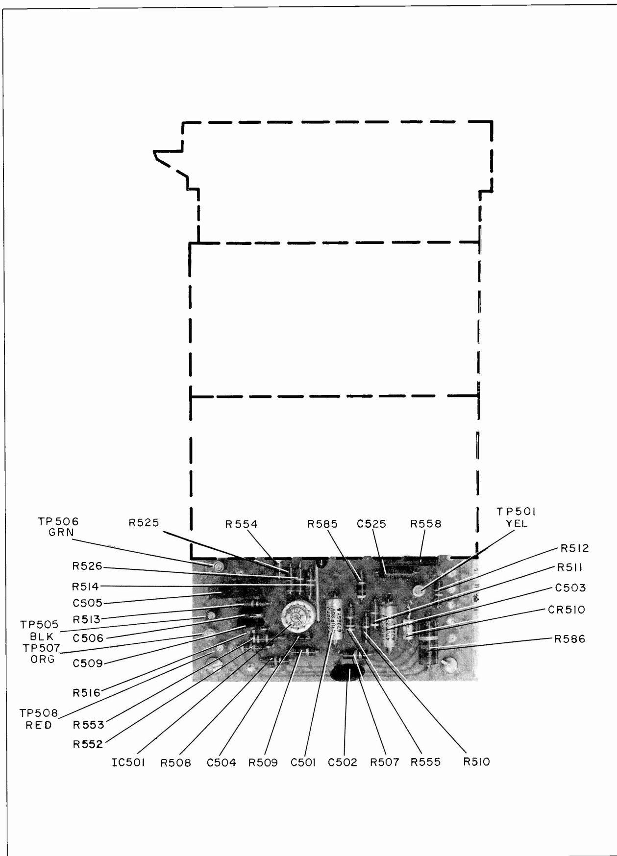
Figure 43. SCA Generator Board, Parts Location, Ser. No. 1 through 999
