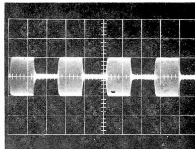
TP312 (blue); Switch .5 V/cm, 10 \mu sec/cm Sync: Ext. from TP304
