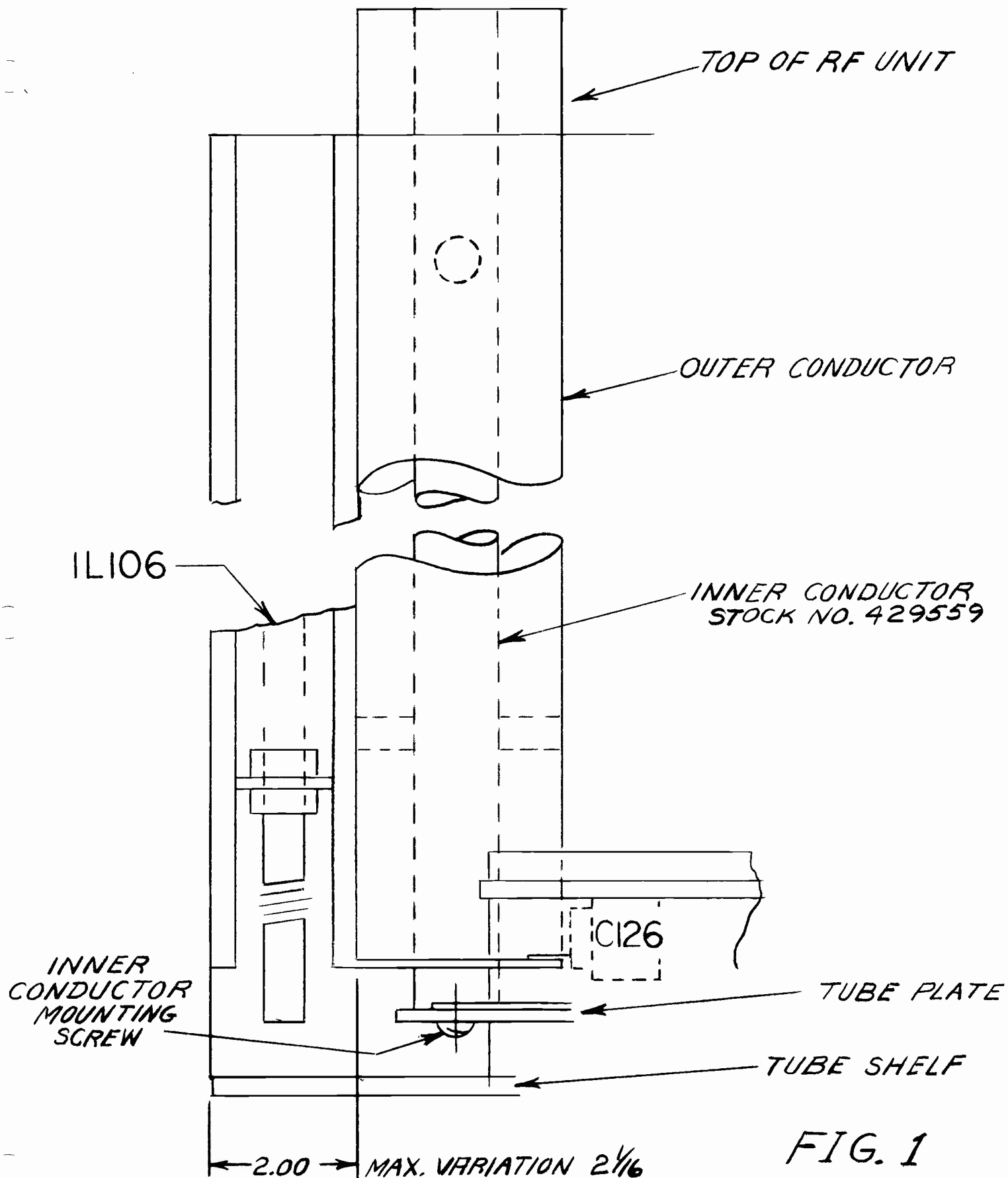
FRONT VIEW OF RF COMPARTMENT
