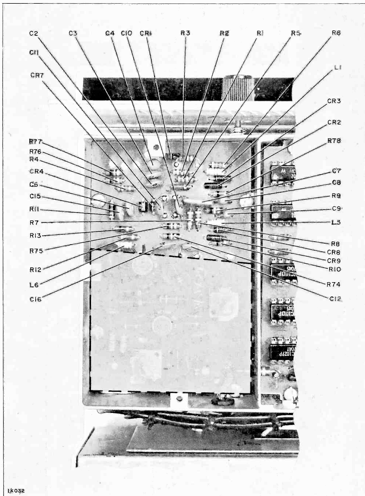
Figure 19. Exciter, Modulated Oscillator Board, Parts Location
