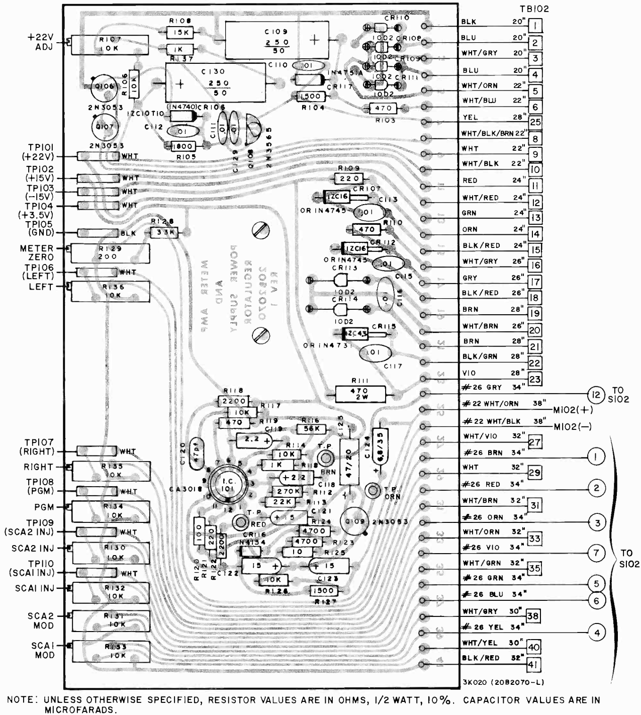
Figure 16. Main Frame Metering Amplifier Board, Parts Overlay, Top
