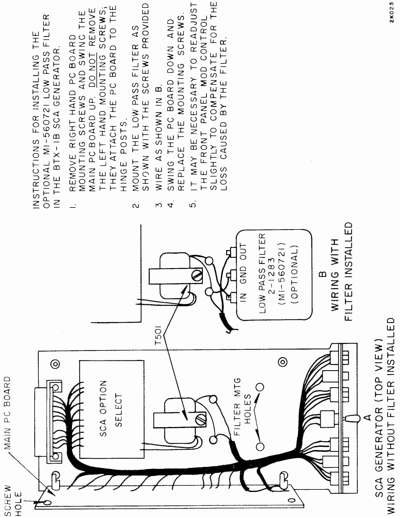
Figure 57. BTX-1B Low Pass Filter Installation
