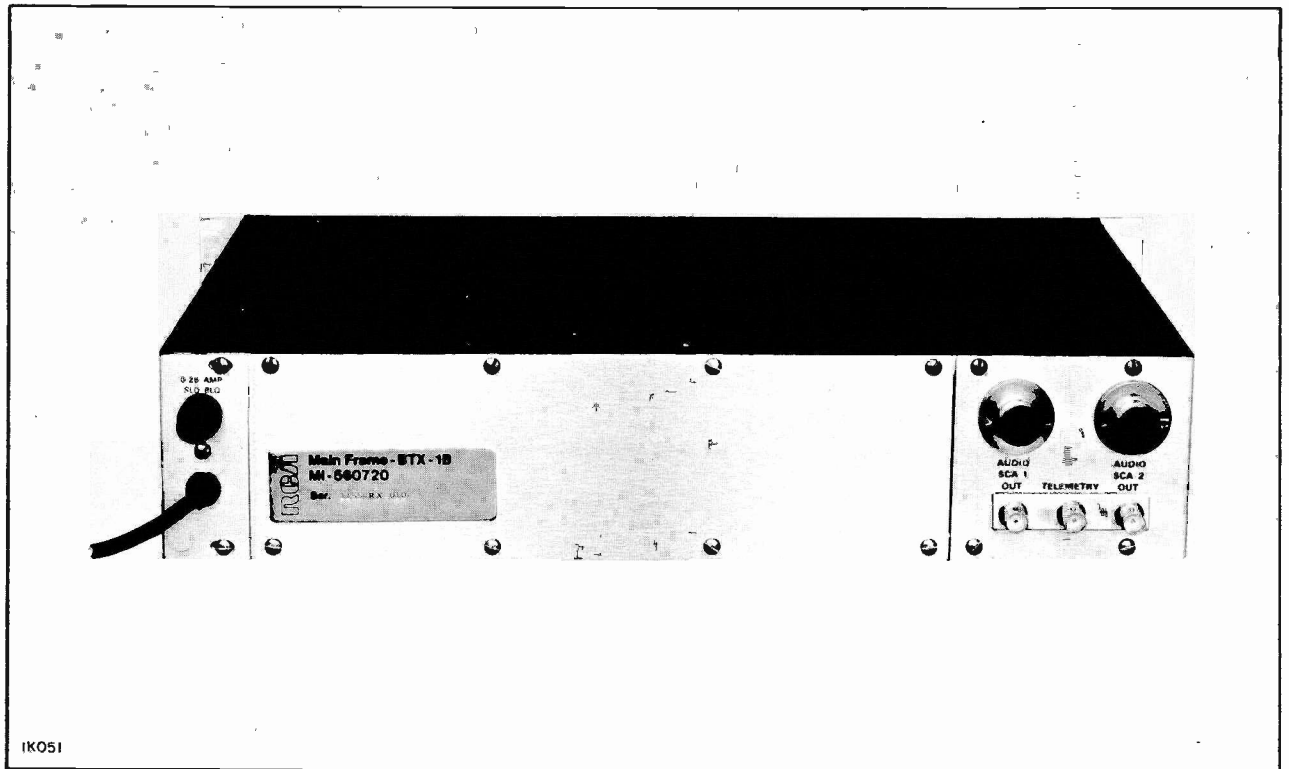
Figure 75. BTX-1B SCA Generator, Rear View
