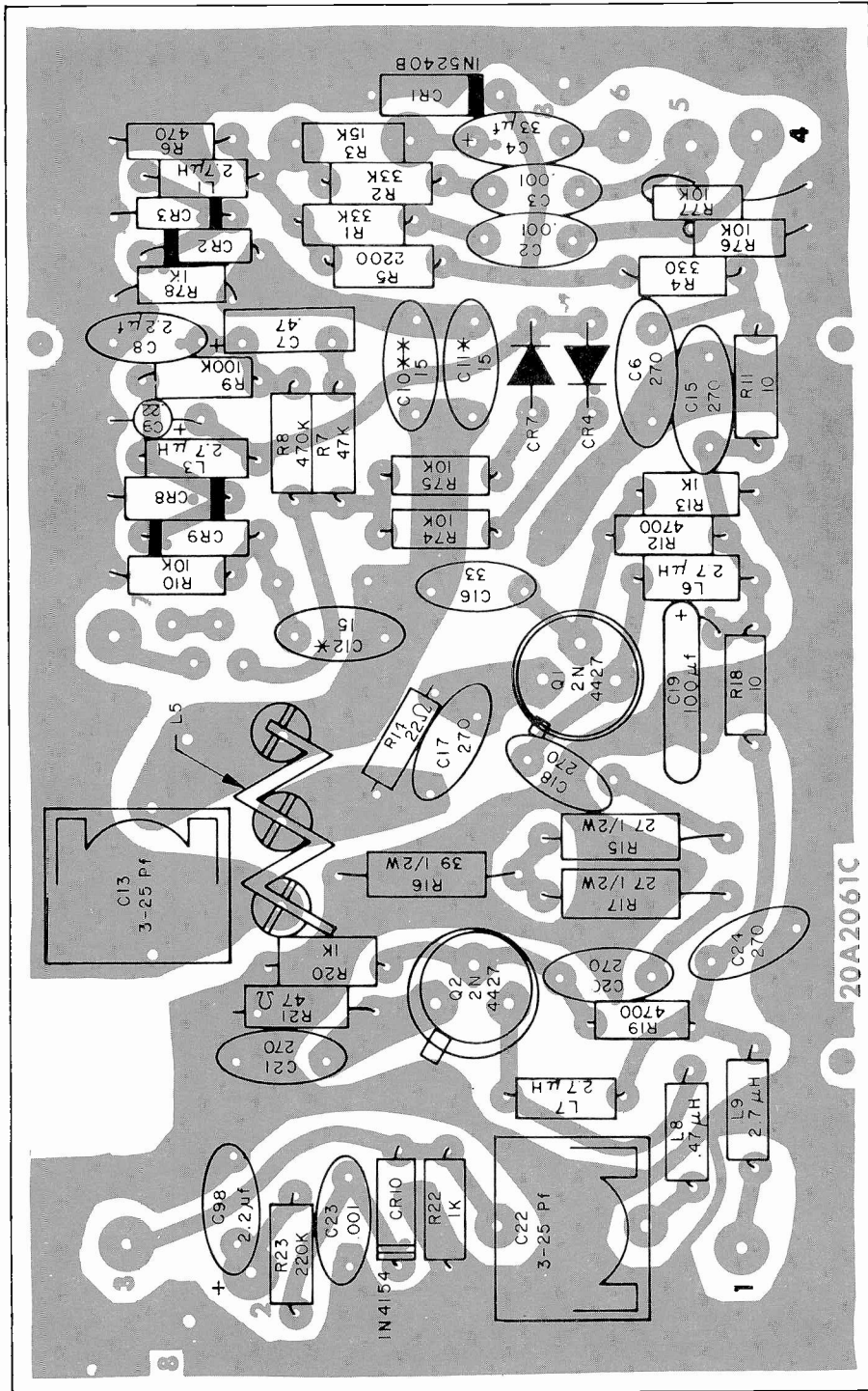
Figure 25. Exciter, Modulated Oscillator Board, Parts Overlay, Bottom
