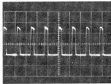
TP301 (yellow); 76 kHz 2 V/cm, 10 \mu\text{sec}/\text{cm} Sync: Ext. from TP304
