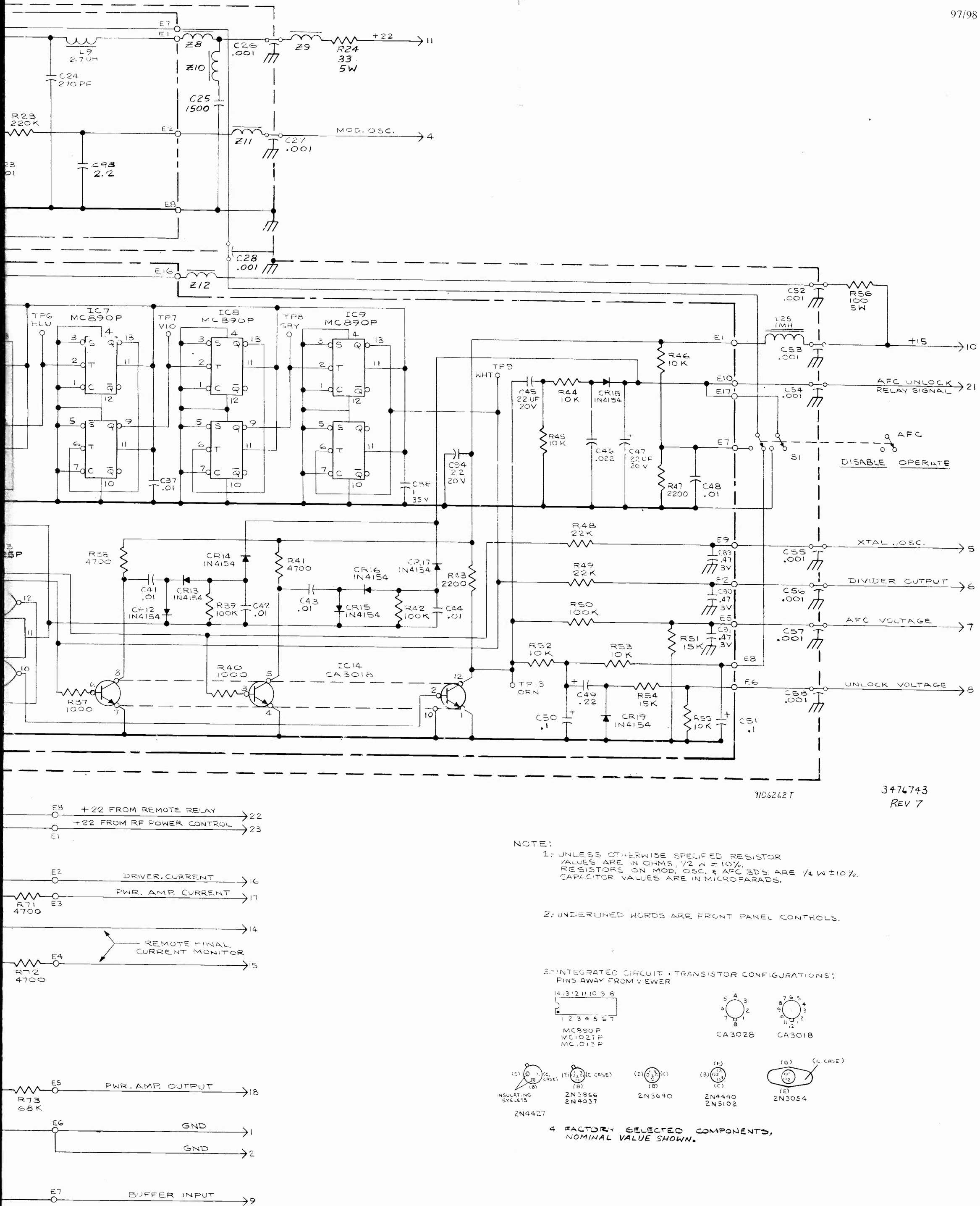
Figure 51. BTE-15A FM Exciter, Schematic Diagram
