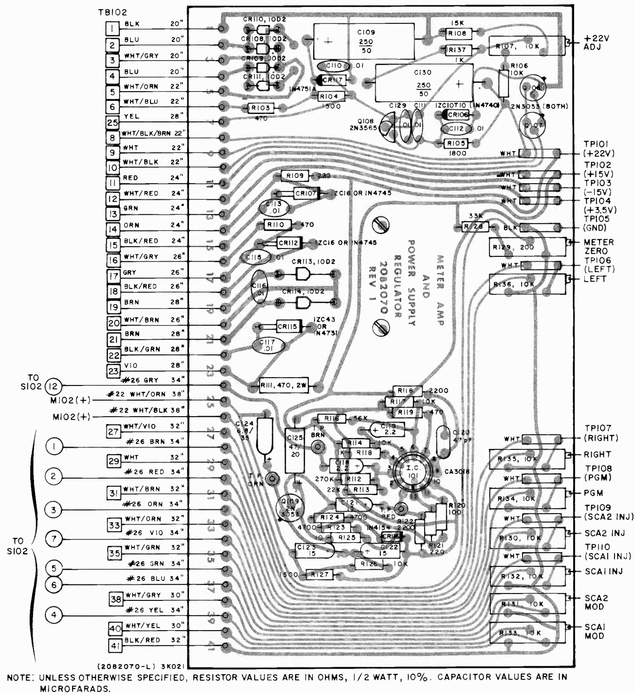
Figure 17. Main Frame Metering Amplifier Board, Parts Overlay, Bottom
