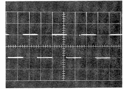
TP302 (green); 38 kHz #1 2 V/cm, 10 \mu\text{sec}/\text{cm} Sync: Ext. from TP304
