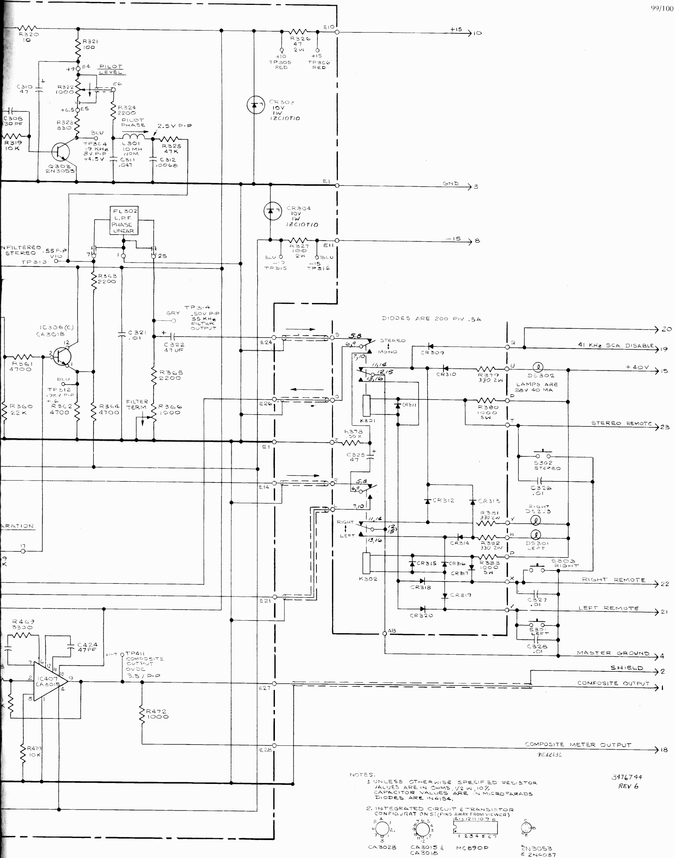
Figure 52. BTS-1B Stereo Generator, Schematic Diagram
