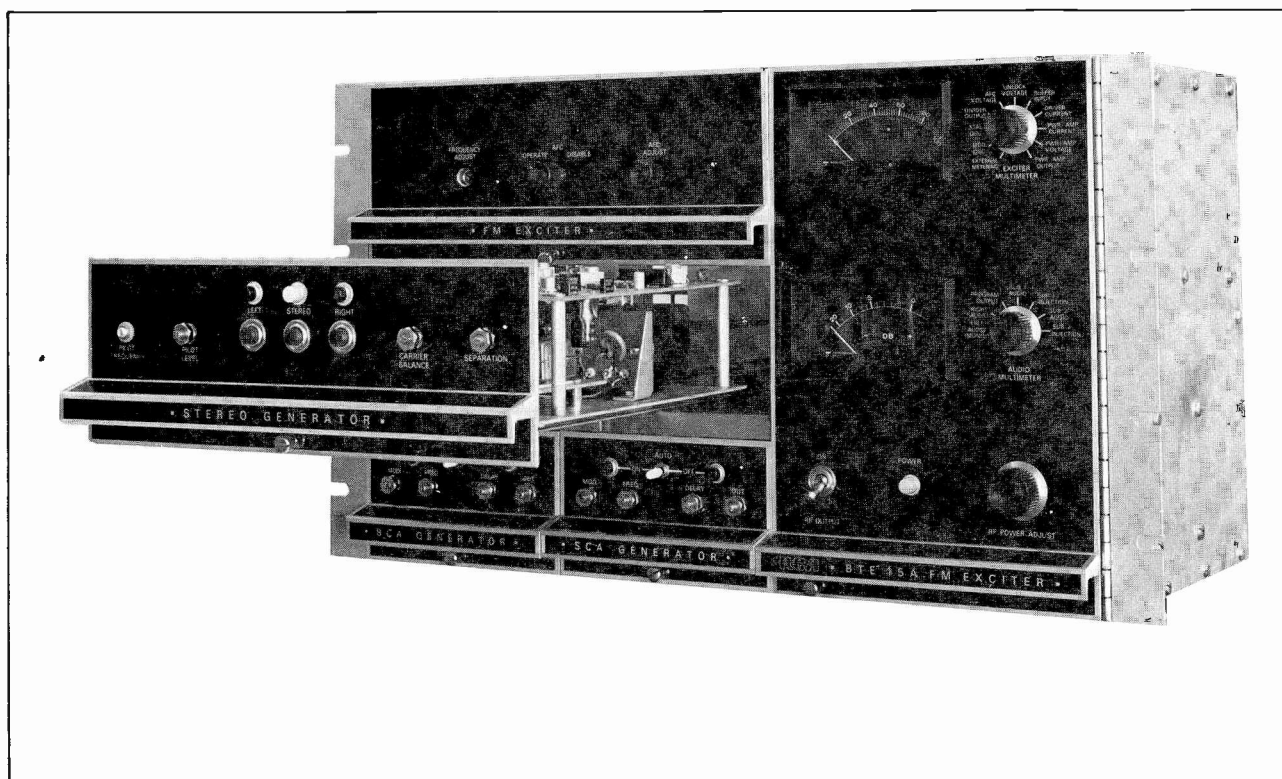
Figure 8. BTE-15A System, Module Extender Installed
