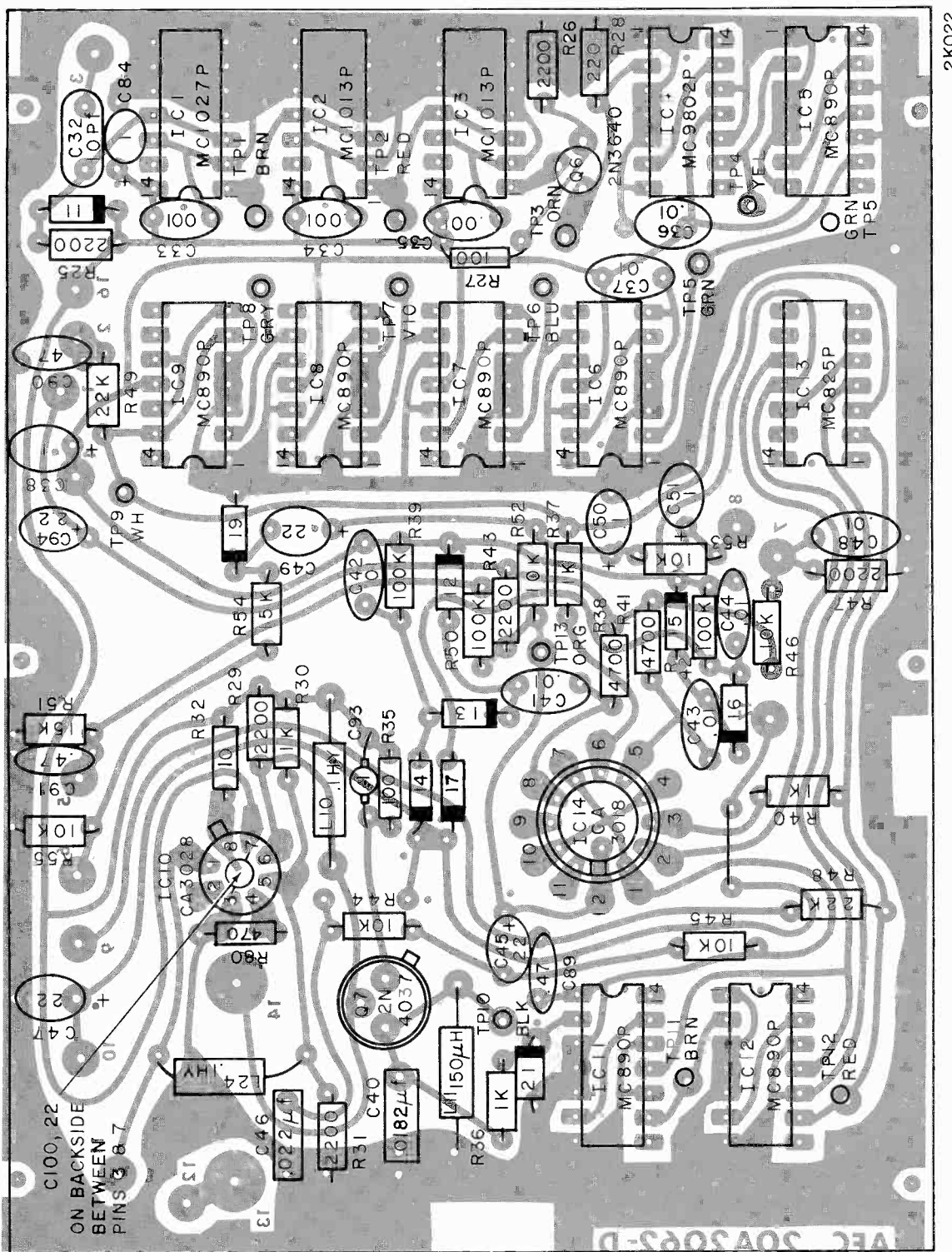
Figure 26. Exciter, AFC Board, Parts Overlay, Top
