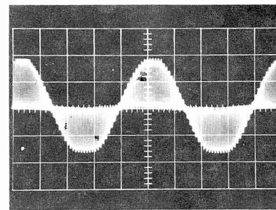
TP411 (white); Composite Output 1 V/cm, .5 ms/cm Sync: Ext. audio generator Waveform showing effect of extreme overmodulation; input level increased to give more than 200% modulation.
