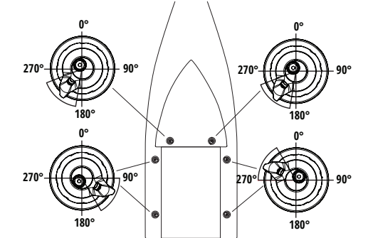
ARM ORIENTATION The image above can be used as a guide to the orientation of the self-tailing arm in typical locations on the deck.
