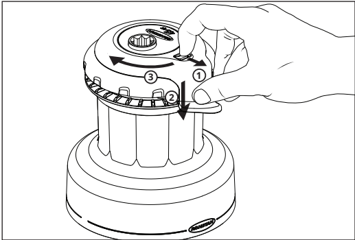
STEP 3 Reassemble the winch as per instructions above.
