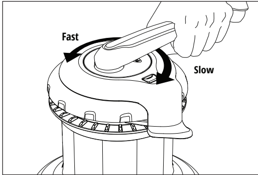
STEP 3 Two speed operation, overdrive button (RA6503 only) not engaged. Check that the drum turns smoothly when rotated by hand in a clockwise direction, and is not able to turn in an anti-clockwise direction. Insert a winch handle in the socket of the central drive shaft. Turning the handle in an clockwise direction should drive the drum in it's slowest speed; turning the handle in an anti-clockwise direction should drive it in the faster speed. For a three-speed winch, after pushing the button on top of the winch turning the handle clockwise should drive the winch in the fastest (overdrive) gear.
