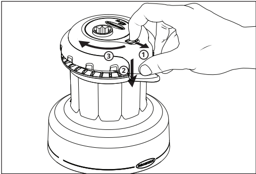
STEP 2 Rotate the self-tailing arm to its desired position, ensuring that the rope splitter is in position. Pull back the spring-loaded release latch on the self-tailing arm with a fingertip (1), then rotate the arm slightly in a clockwise direction (3), and listen for the audible "click" indicating it is locked in position (2).
