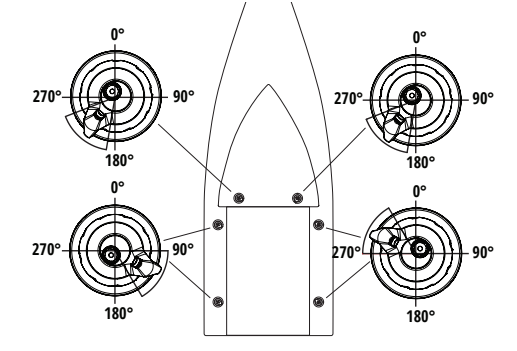
ARM ORIENTATION The image above can be used as a guide to the orientation of the self-tailing arm in typical locations on the deck.
