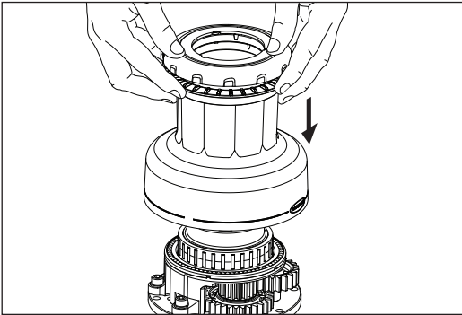
STEP 1 Lift the drum assembly over the centre stem, then slide it fully down into position.
