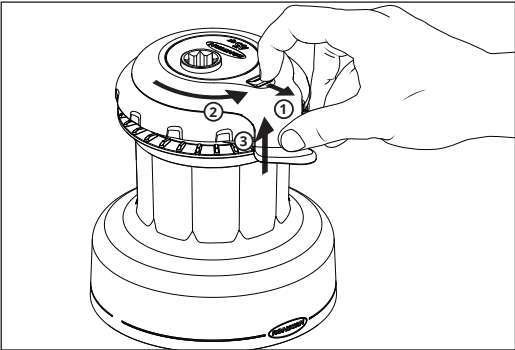
STEP 1 Remove the self-tailer arm and the closing washer and set aside for now.
