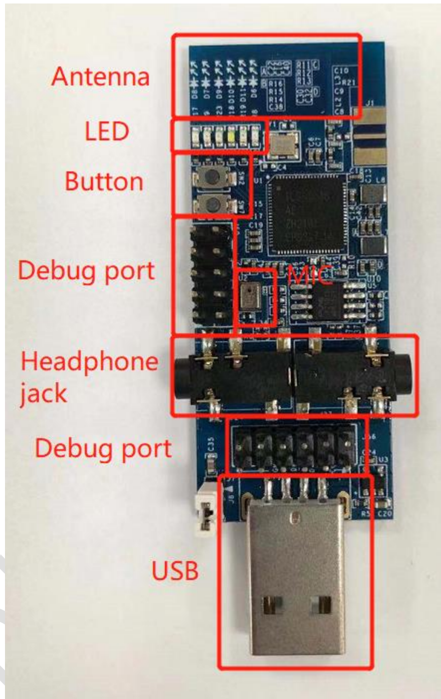
Figure 2-3 Function modules on the board
