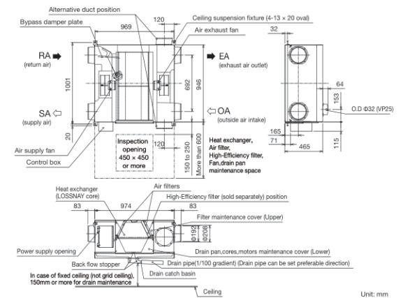
Outline drawings
