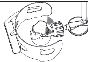
Regulator/Cylinder Connection
