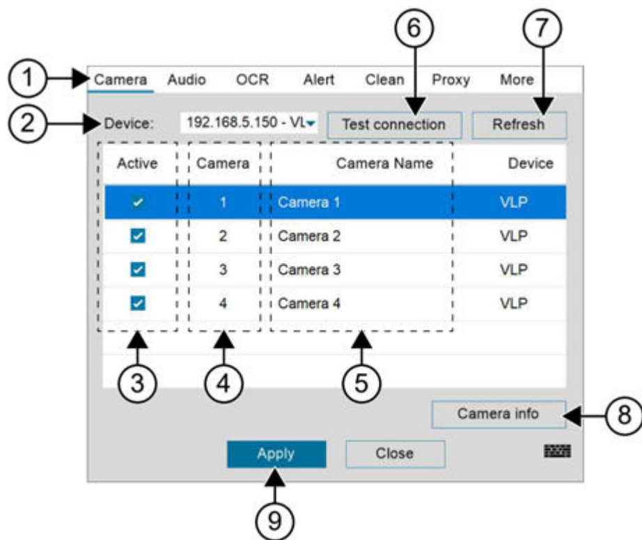
Figure 36: VLP Camera Tab
