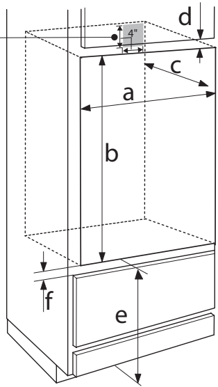
Double Oven - Installed in Cabinet
