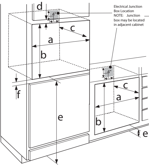
Single Oven - Installed in Cabinet and Installed Undercounter
