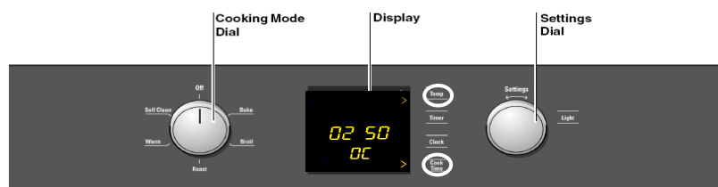
Figure 20 HBL3/HBN3 User interface
