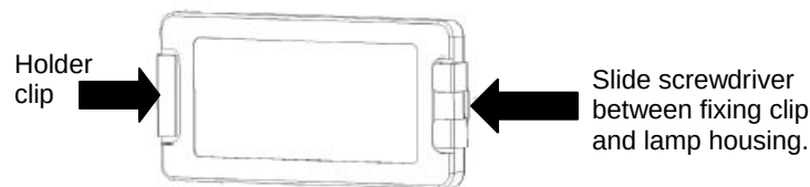
Figure 10 Horizontal-style side lamp
