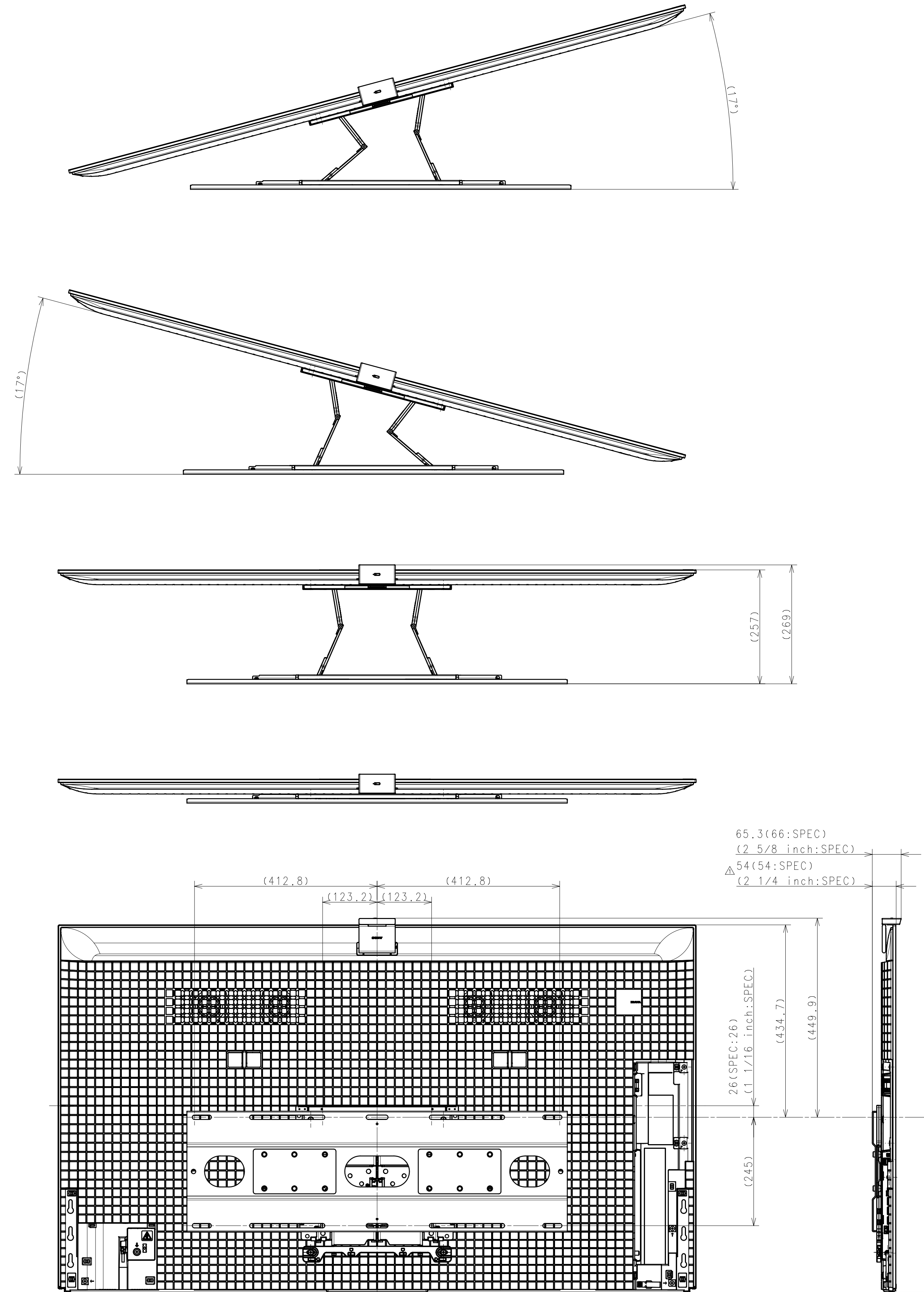
SU-WL855 with LATERAL SHAFT BRACKET
