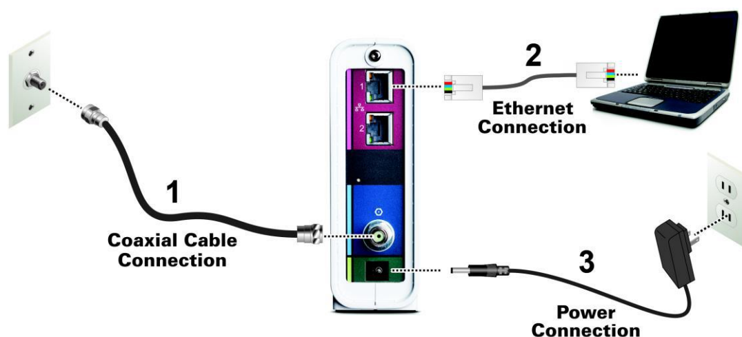
Figure 4: SB8200 Connection Diagram
