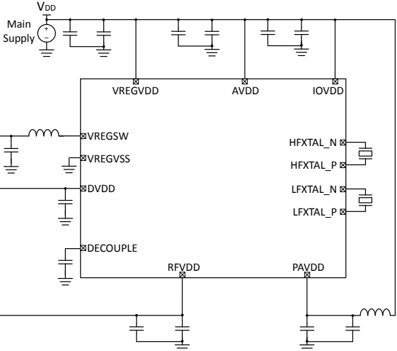
Figure 5.3. EFR32BG1 Typical Application Circuit: Configuration with DC-DC converter (PAVDD from VDD)
