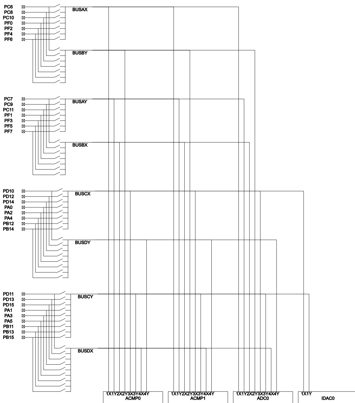
Figure 6.4. EFR32BG1 APORT
