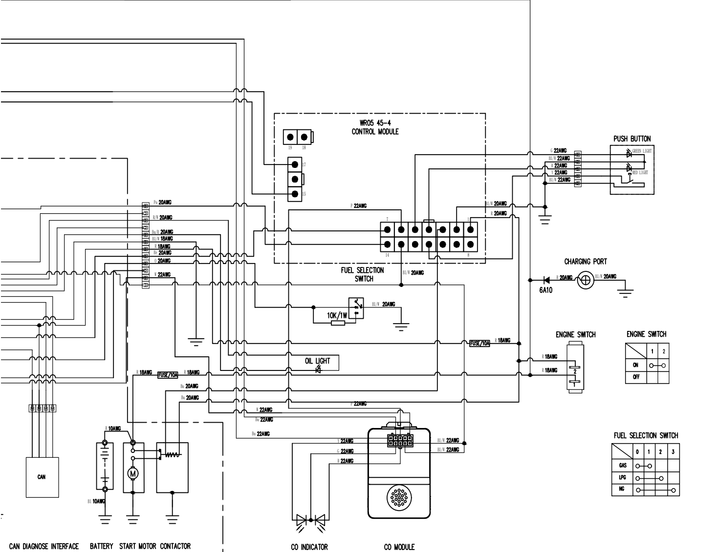
WIRING DIAGRAM OF XP15000HXT GENERATOR SET
