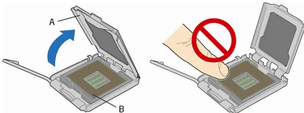
Figure 7. Lift the Load Plate
