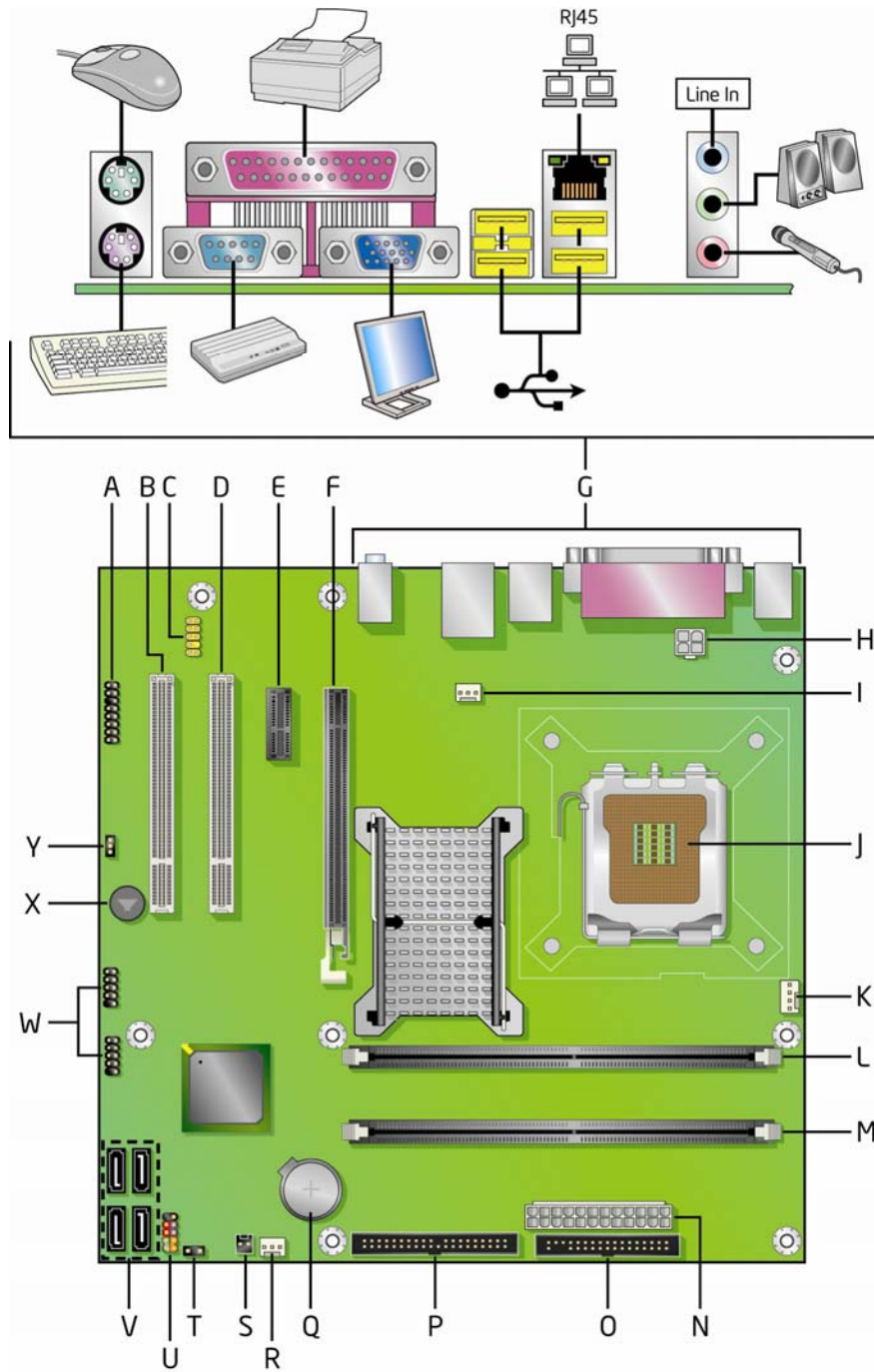
Figure 1. Desktop Board D946GZAB Components
