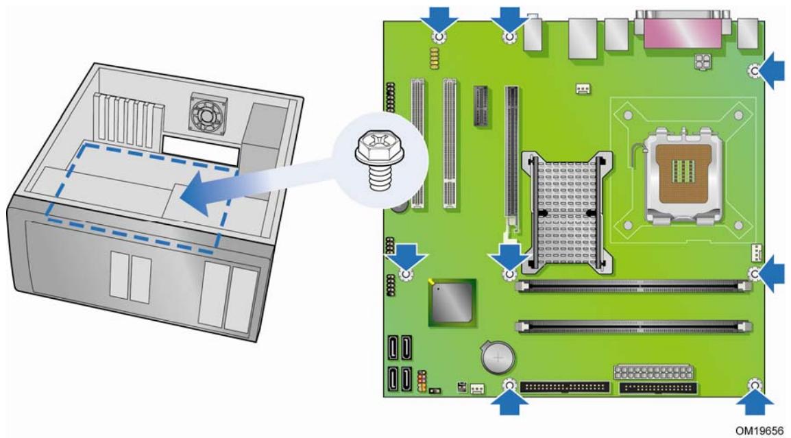
Figure 5. Desktop Board D946GZAB Mounting Screw Hole Locations
