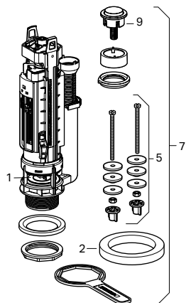
Flushing Valve Type 290 Single-flush
