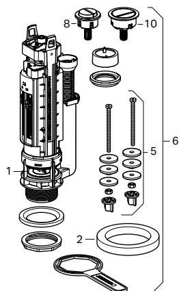
Flushing Valve Type 290 Dual-flush
