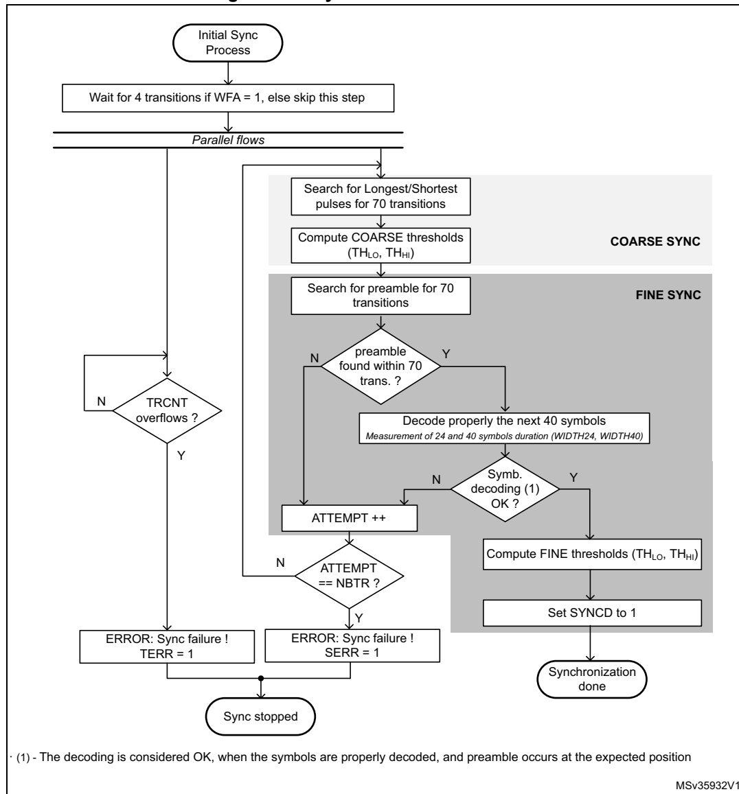
Figure 345. Synchronization flowchart
