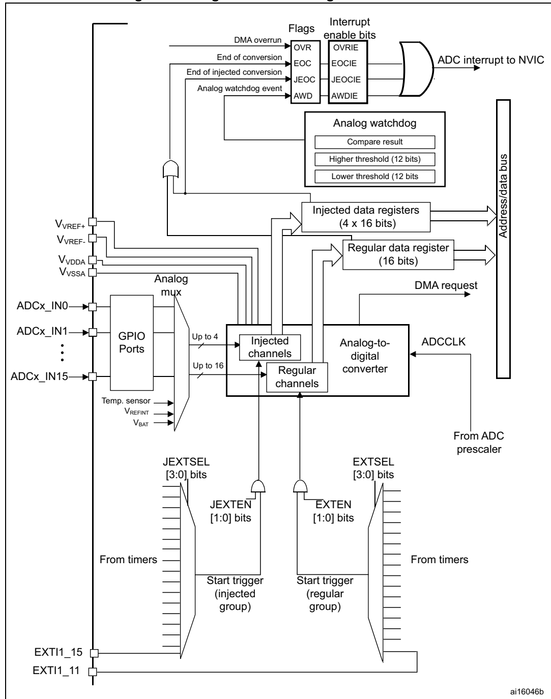
Figure 69. Single ADC block diagram
