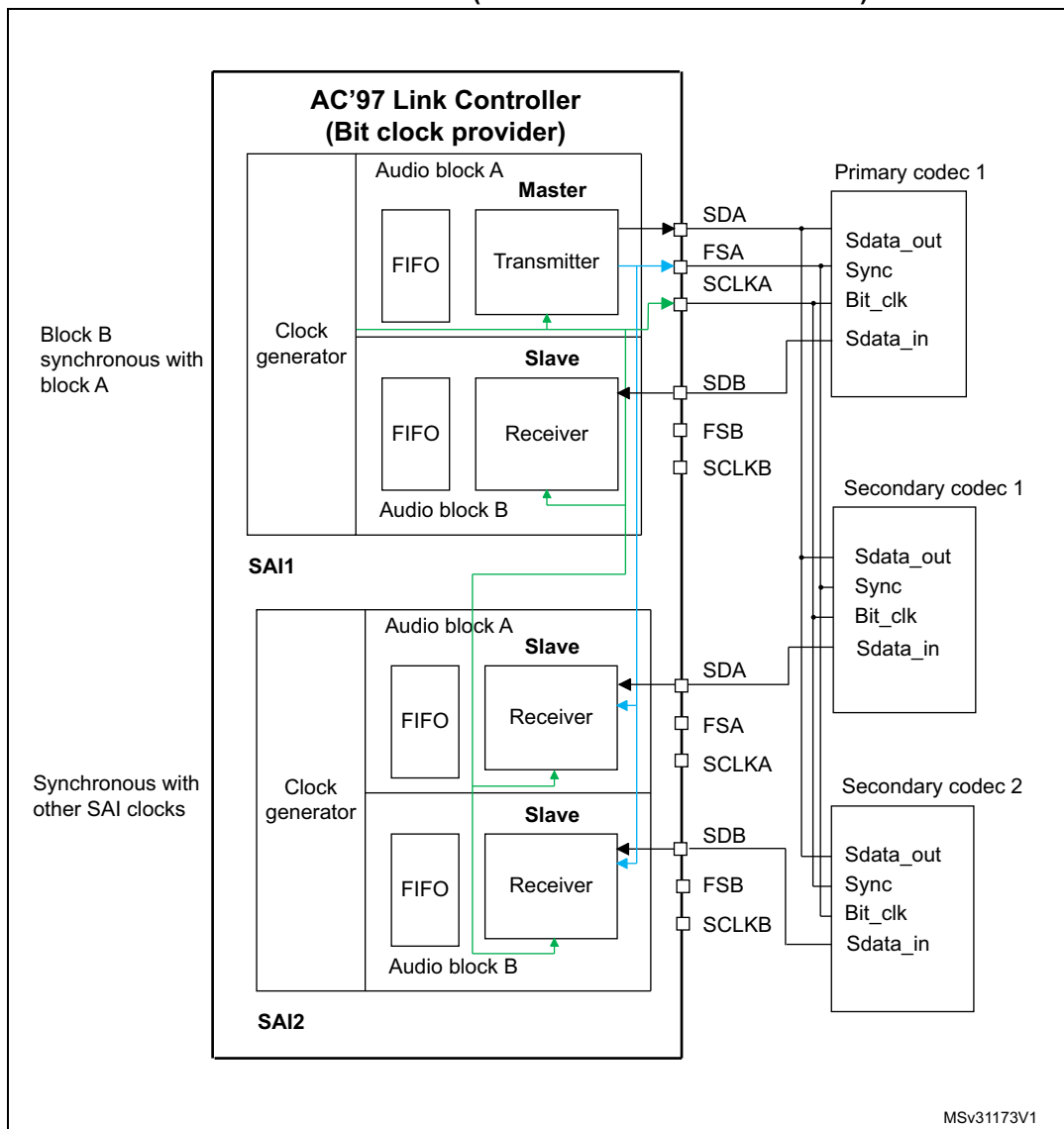
Figure 361. Example of typical AC'97 configuration on devices featuring at least two embedded SAIs (three external AC'97 decoders)
