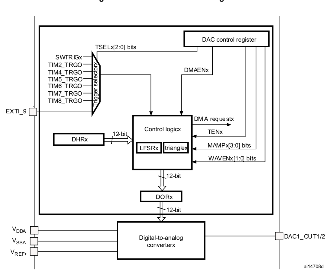
Figure 92. DAC channel block diagram
