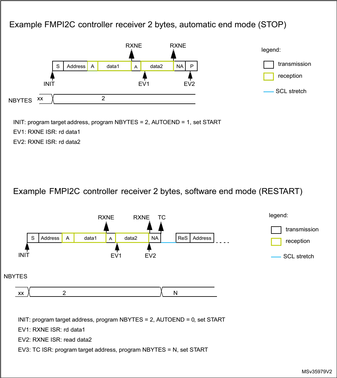
Figure 263. Transfer bus diagrams for FMPI2C controller receiver (mandatory events only)
