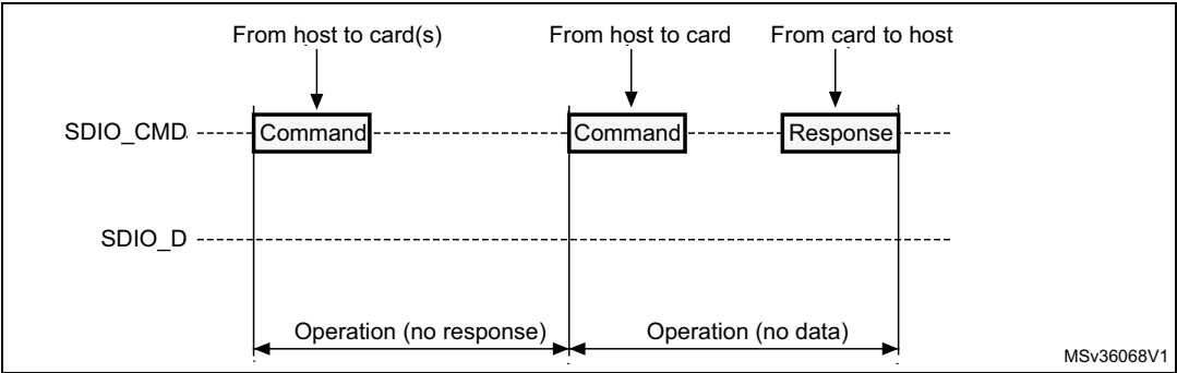
Figure 369. “No response” and “no data” operations
