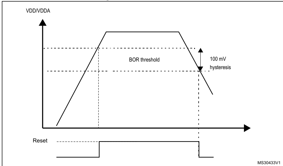
Figure 11. BOR thresholds
