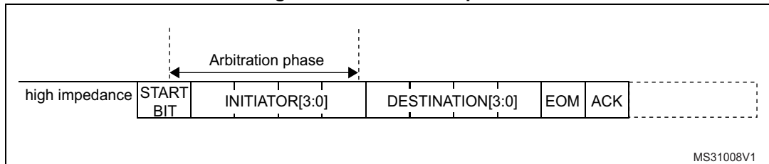
Figure 436. Arbitration phase
