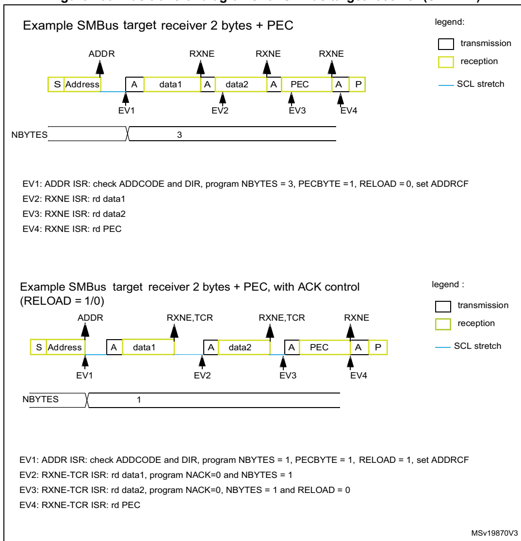
Figure 268. Bus transfer diagrams for SMBus target receiver (SBC = 1)
