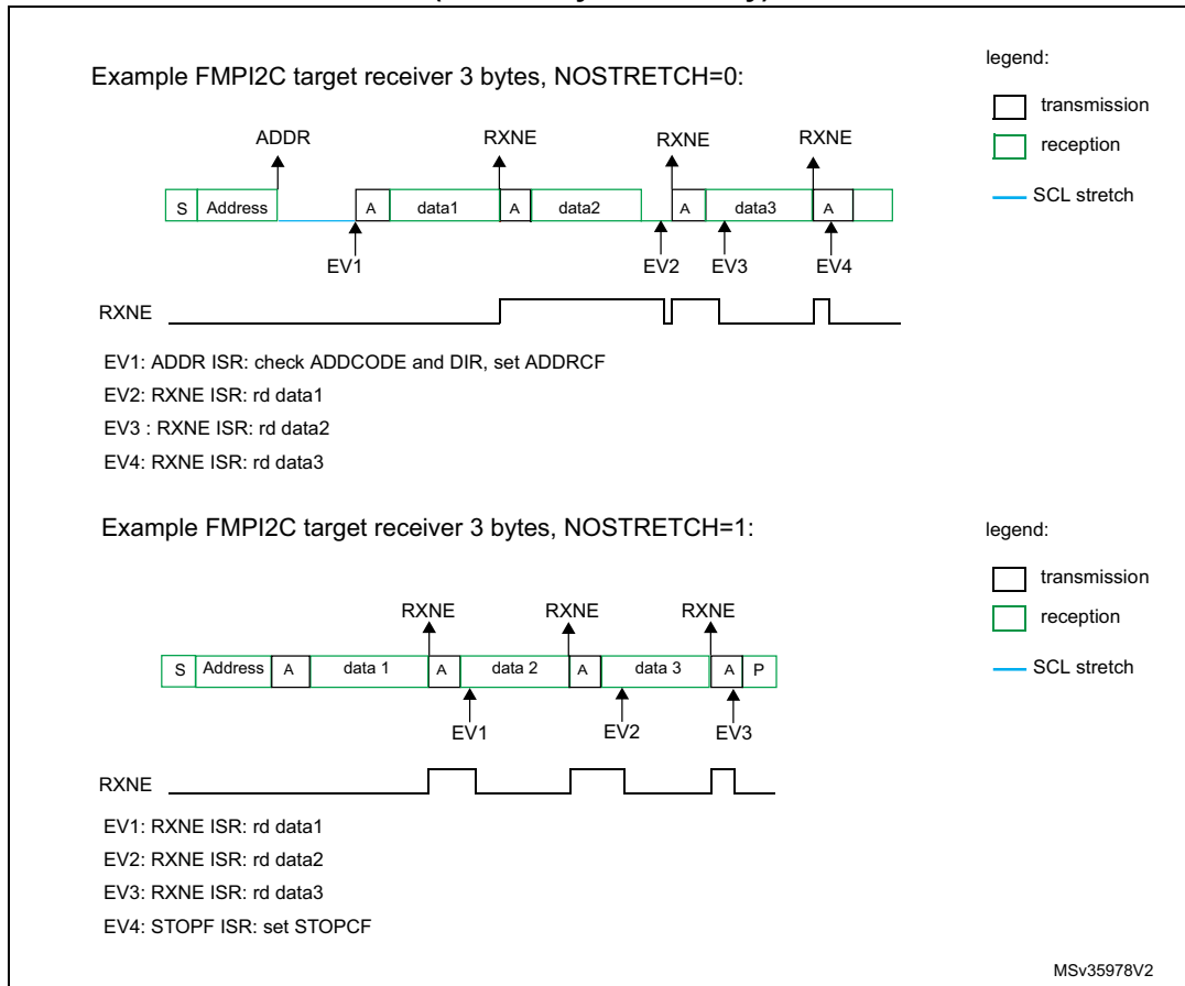
Figure 253. Transfer bus diagrams for FMPI2C target receiver (mandatory events only)
