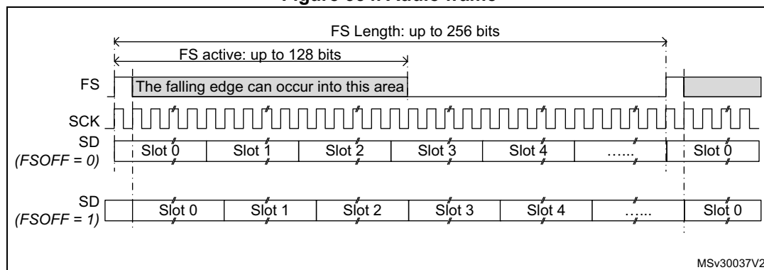
Figure 354. Audio frame
