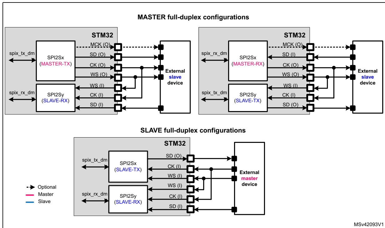
Figure 317. Full-duplex communication
