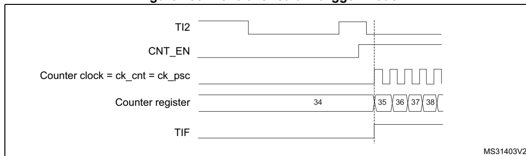
Figure 156. Control circuit in trigger mode
