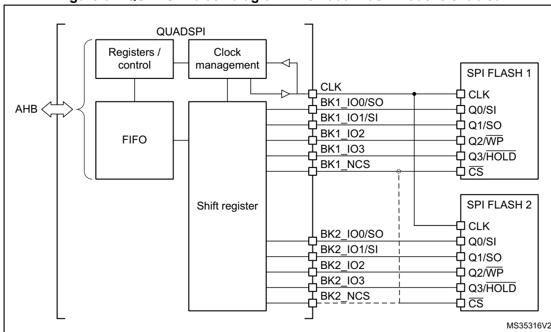
Figure 62. QUADSPI block diagram when dual-flash mode is enabled
