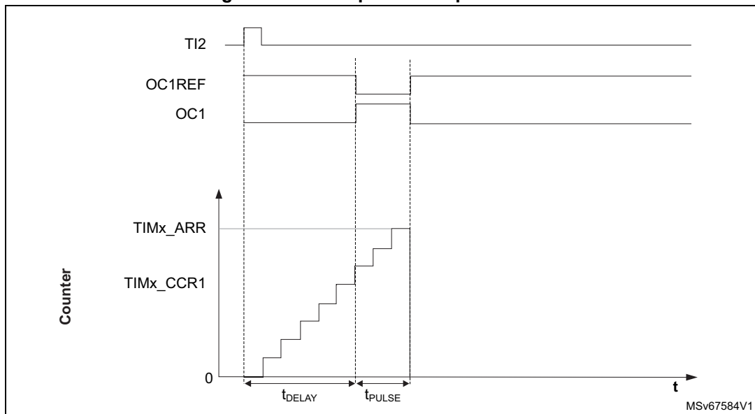
Figure 223. Example of One-pulse mode
