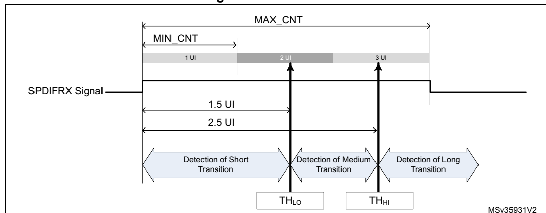
Figure 344. Thresholds
