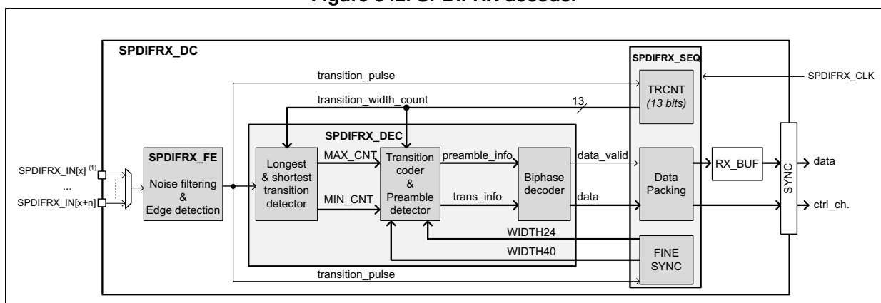
Figure 342. SPDIFRX decoder
