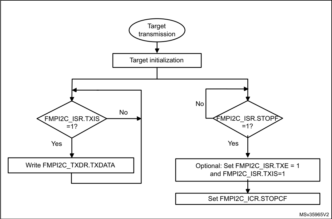
Figure 249. Transfer sequence flow for FMPI2C target transmitter, NOSTRETCH = 1
