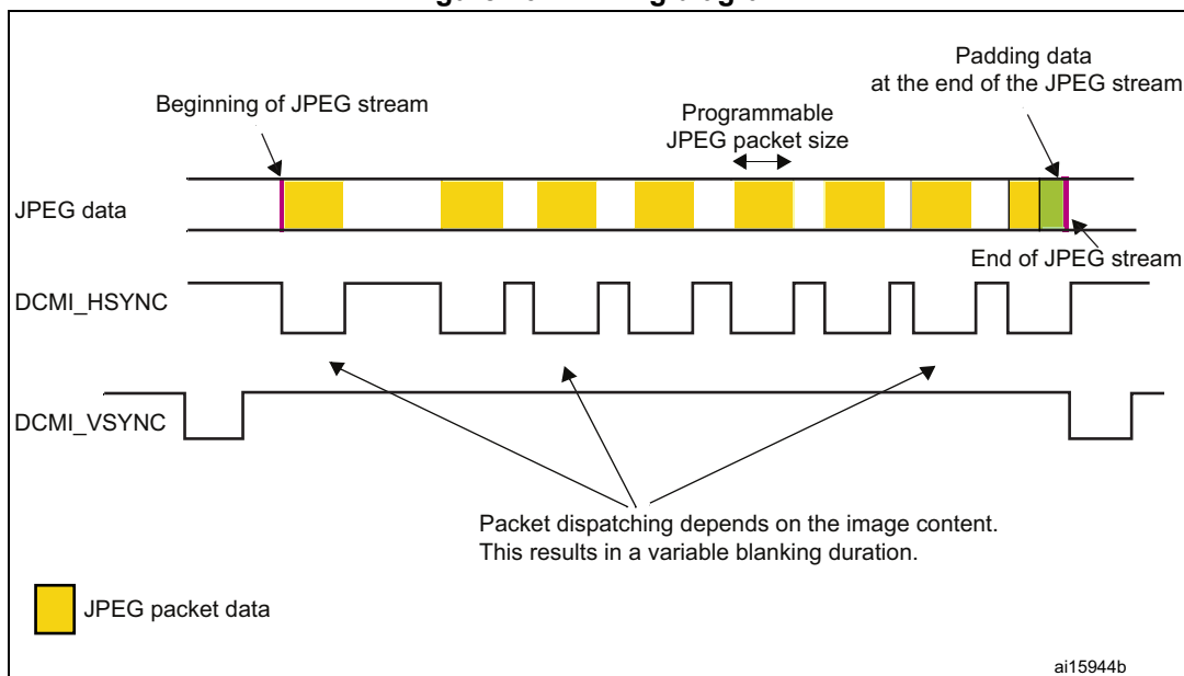
Figure 104. Timing diagram
