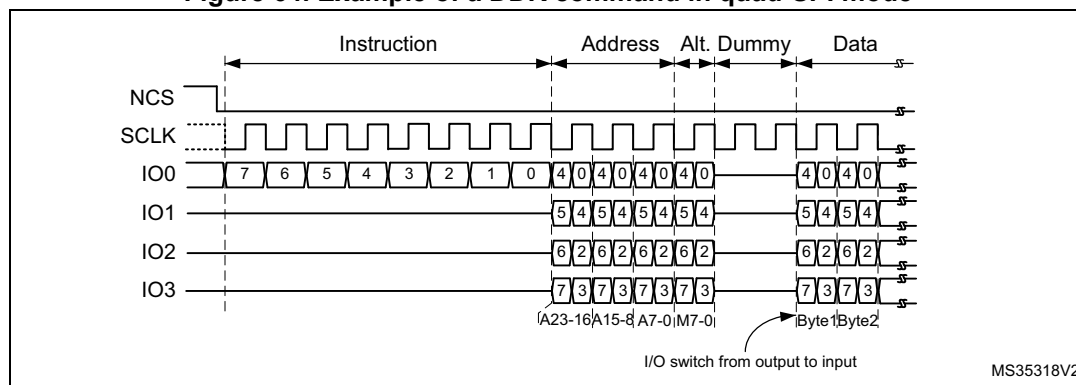
Figure 64. Example of a DDR command in quad-SPI mode
