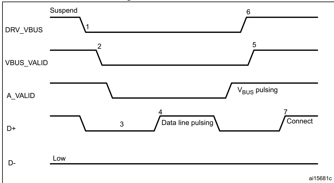
Figure 427. A-device SRP
