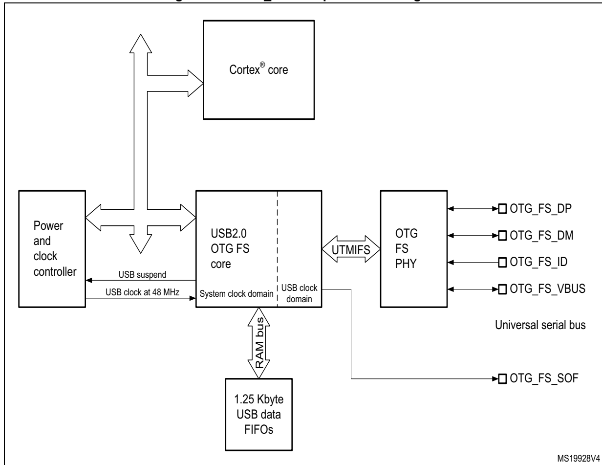
Figure 399. OTG_FS full-speed block diagram
