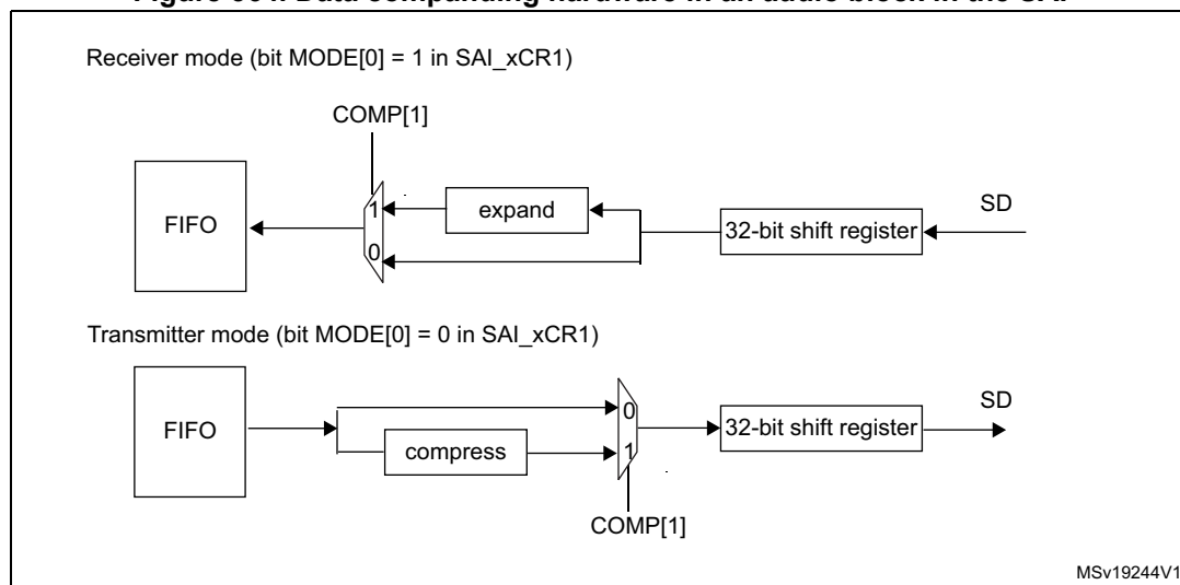
Figure 364. Data companding hardware in an audio block in the SAI
