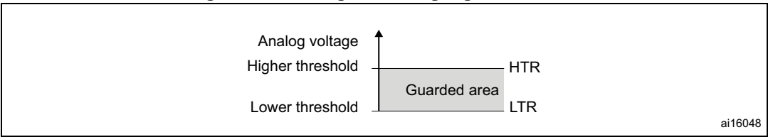
Figure 74. Analog watchdog's guarded area
