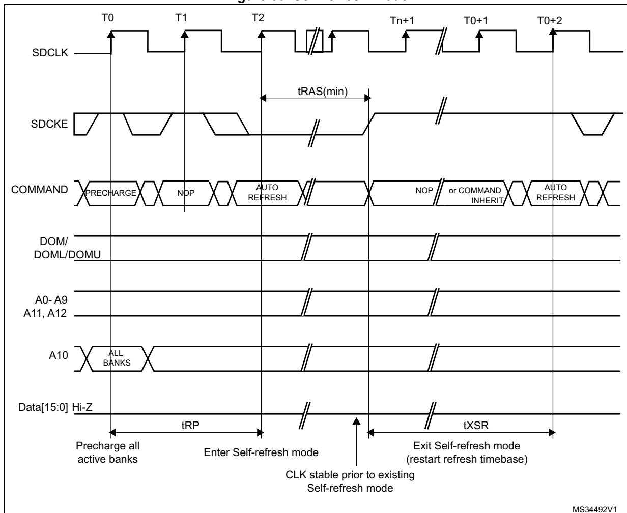
Figure 59. Self-refresh mode
