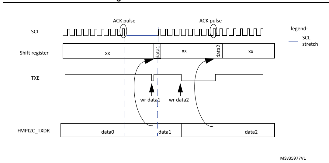
Figure 246. Data transmission
