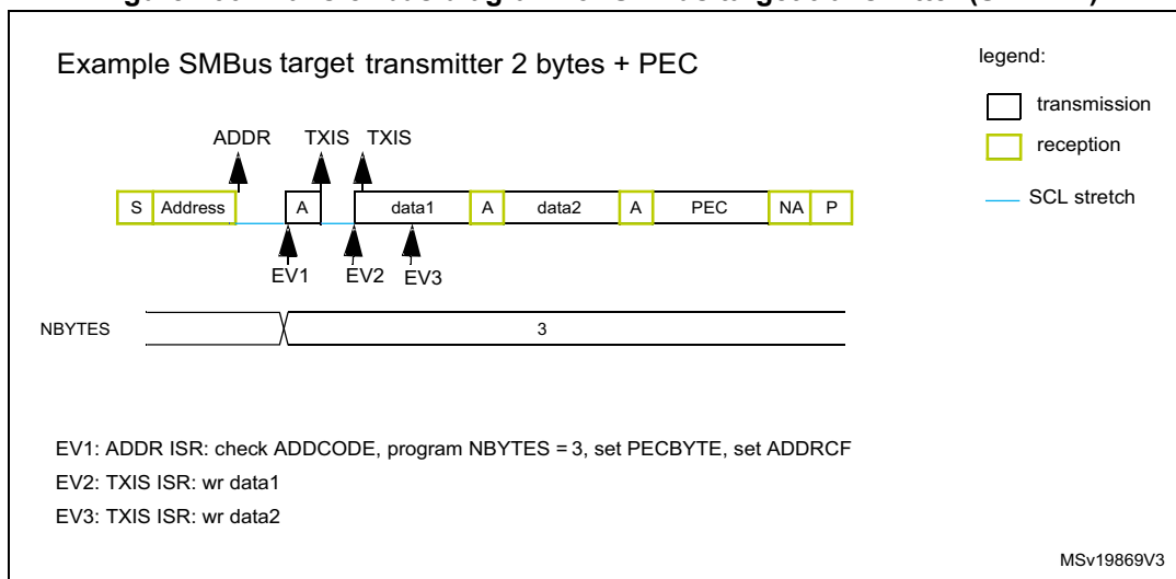
Figure 266. Transfer bus diagram for SMBus target transmitter (SBC = 1)
