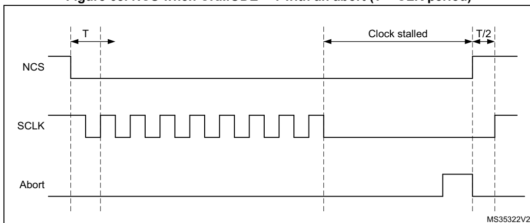
Figure 68. NCS when CKMODE = 1 with an abort ( T = \text{CLK period} )
