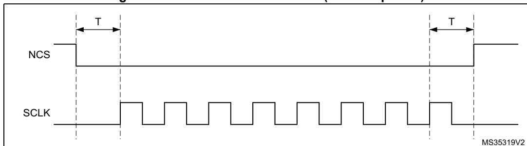
Figure 65. NCS when CKMODE = 0 (T = CLK period)
