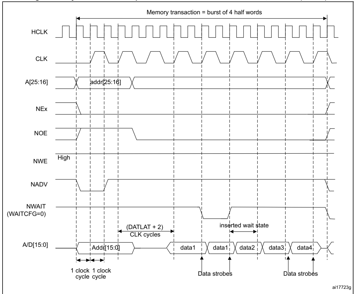
Figure 50. Synchronous multiplexed read mode waveforms - NOR, PSRAM (CRAM)
