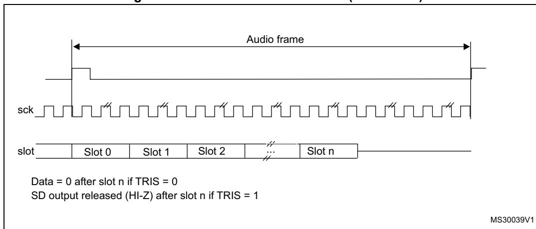
Figure 356. FS role is start of frame (FSDEF = 0)
