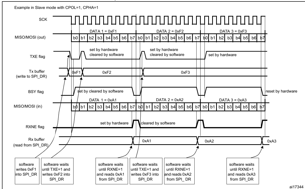
Figure 312. TXE/RXNE/BSY behavior in slave / full-duplex mode (BIDIMODE=0, RXONLY=0) in the case of continuous transfers
