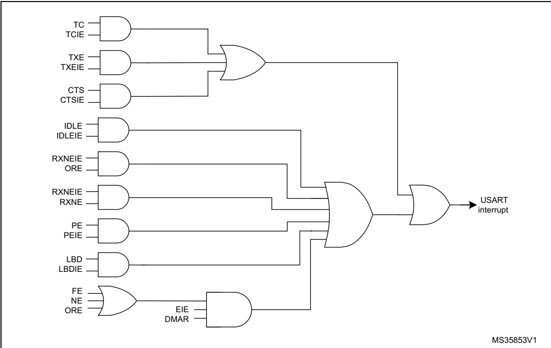
Figure 302. USART interrupt mapping diagram
