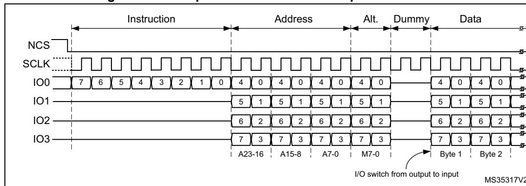
Figure 63. Example of read command in quad-SPI mode
