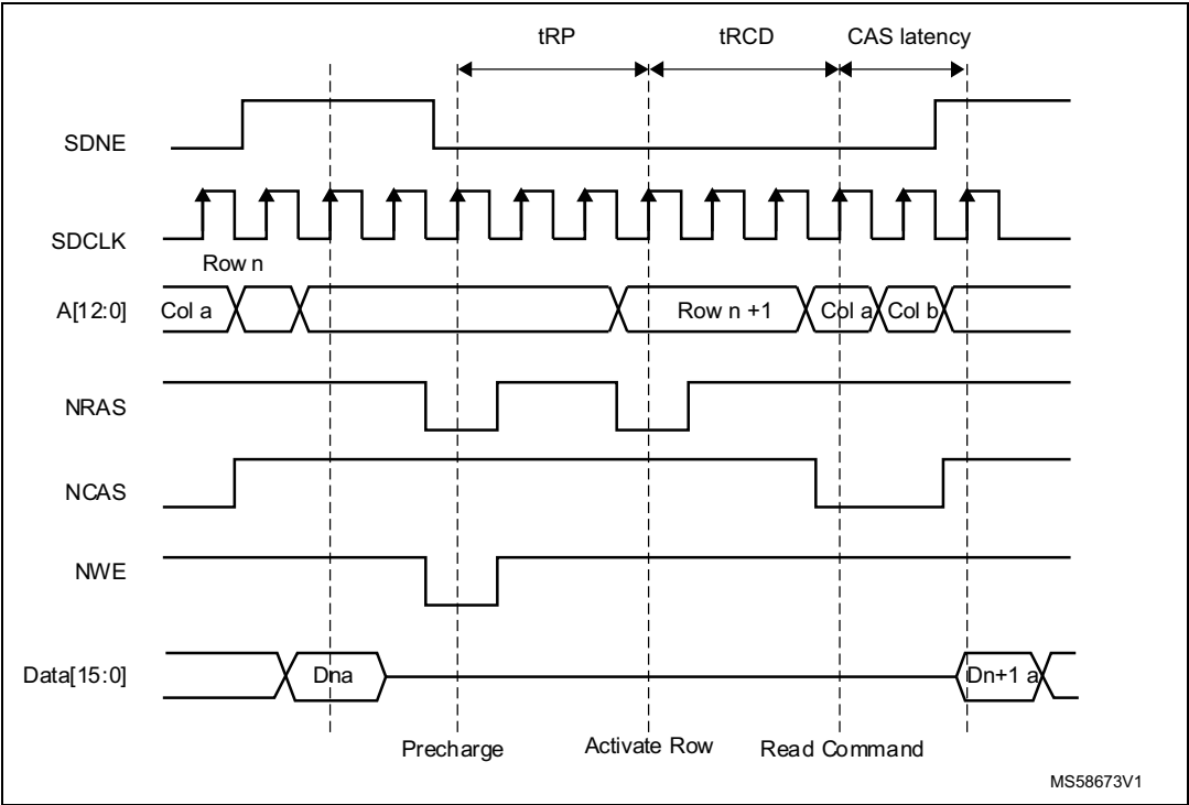
Figure 57. Read access crossing row boundary
