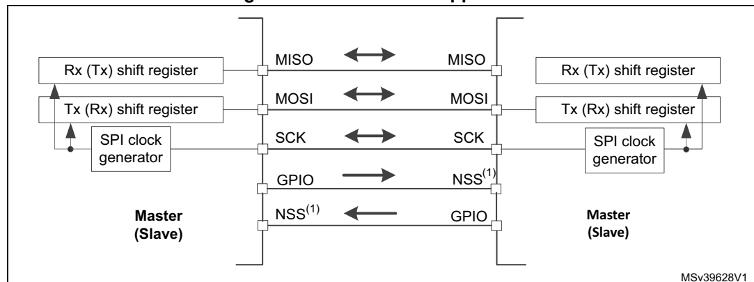
Figure 308. Multimaster application
