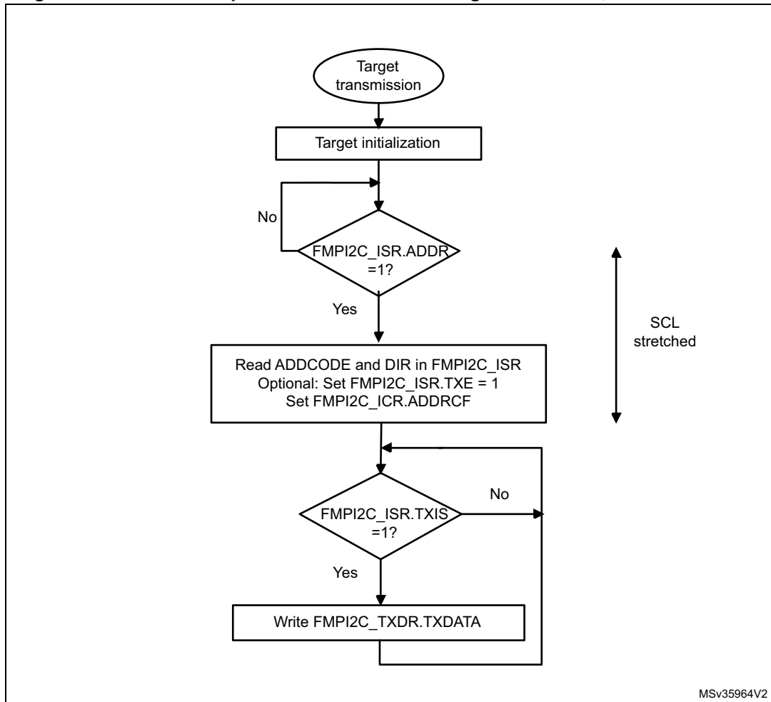
Figure 248. Transfer sequence flow for FMPI2C target transmitter, NOSTRETCH = 0
