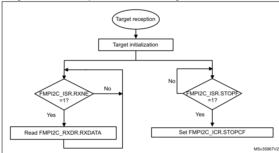
Figure 252. Transfer sequence flow for FMPI2C target receiver, NOSTRETCH = 1
