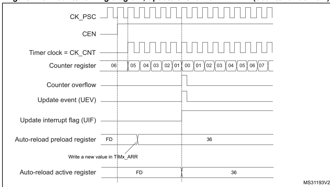
Figure 128. Counter timing diagram, update event with ARPE=1 (counter underflow)
