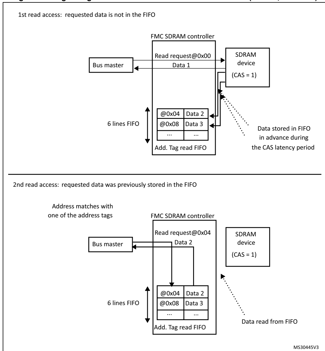
Figure 56. Logic diagram of Read access with RBURST bit set (CAS=1, RPIPE=0)
