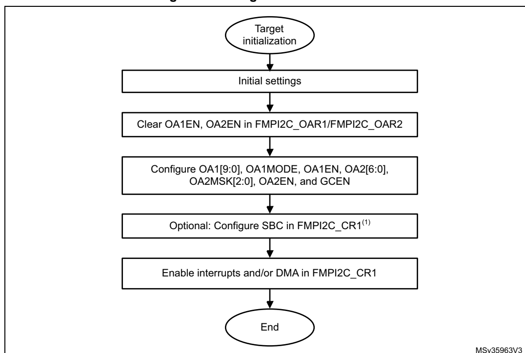
Figure 247. Target initialization flow
