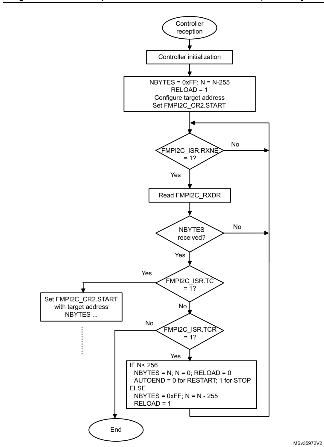
Figure 262. Transfer sequence flow for FMPI2C controller receiver, N &gt; 255 bytes
