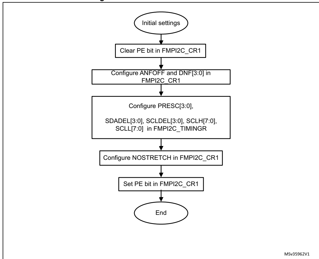
Figure 244. FMPI2C initialization flow
