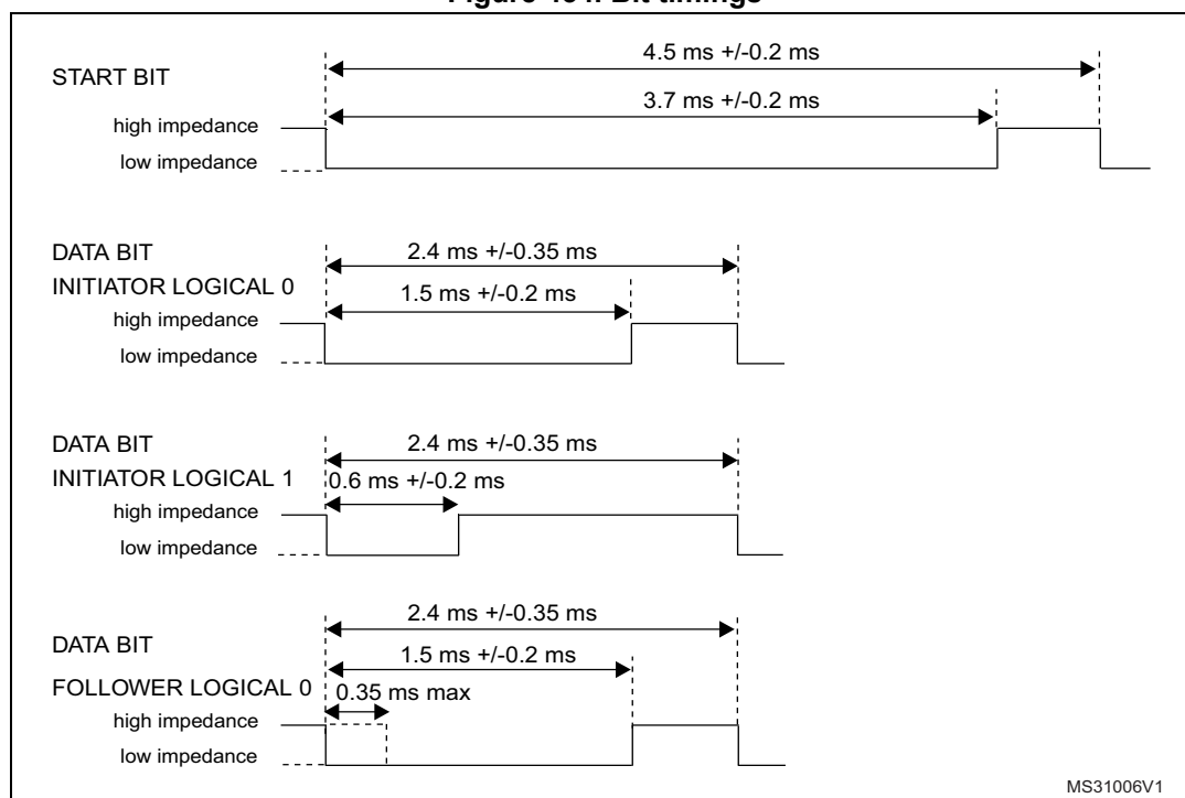
Figure 434. Bit timings
