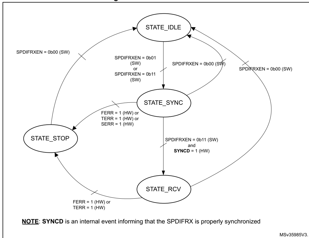
Figure 347. SPDIFRX states
