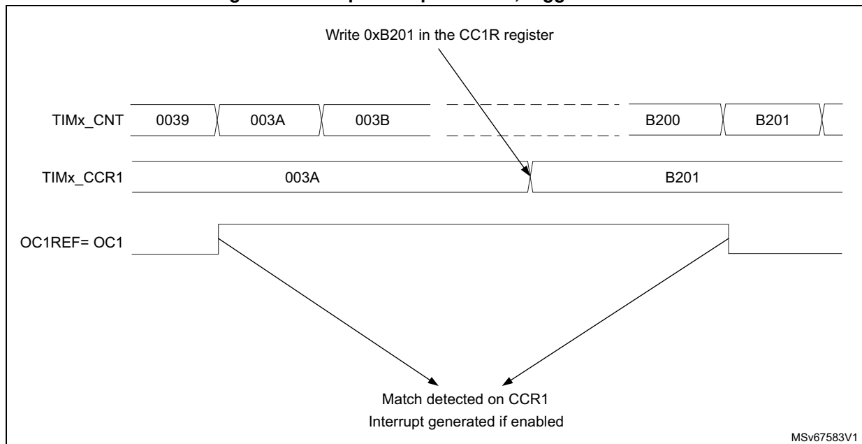
Figure 221. Output compare mode, toggle on OC1.
