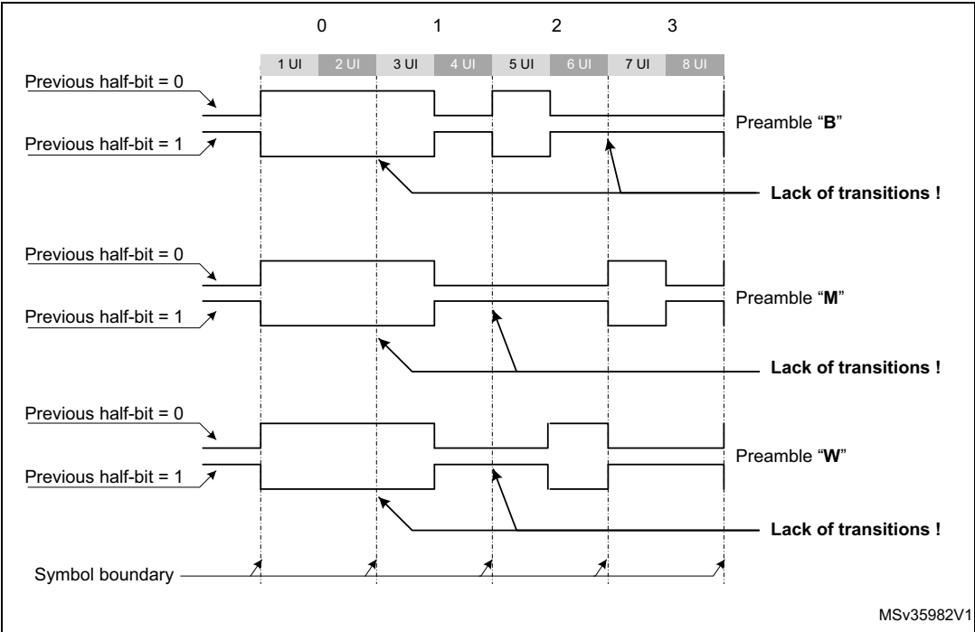
Figure 340. S/PDIF preambles
