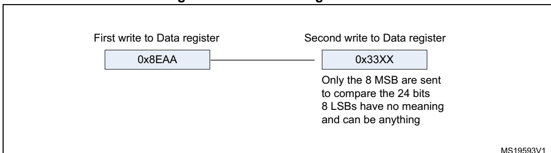
Figure 320. Transmitting 0x8EAA33
