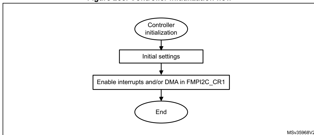
Figure 255. Controller initialization flow
