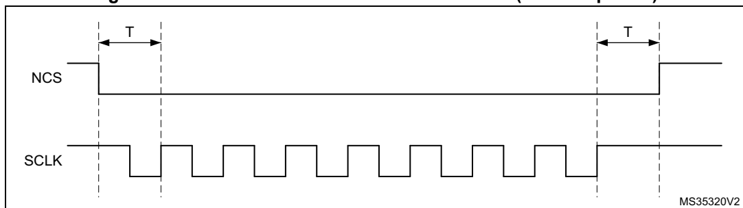
Figure 66. NCS when CKMODE = 1 in SDR mode (T = CLK period)
