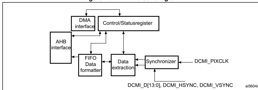
Figure 101. DCMI block diagram
