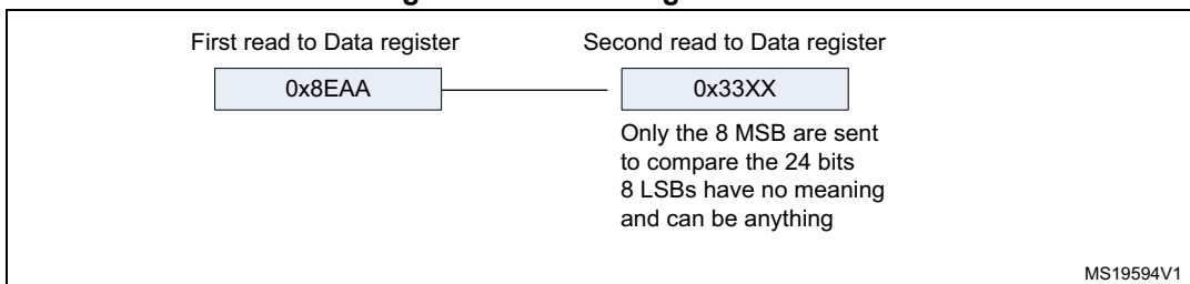
Figure 321. Receiving 0x8EAA33
