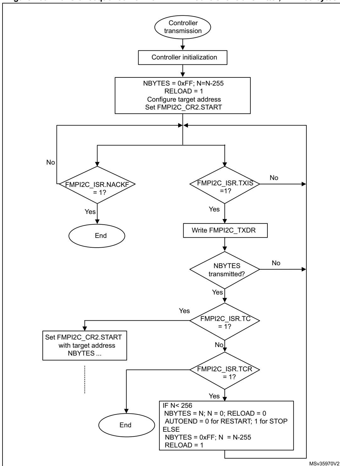
Figure 259. Transfer sequence flow for FMPI2C controller transmitter, N &gt; 255 bytes
