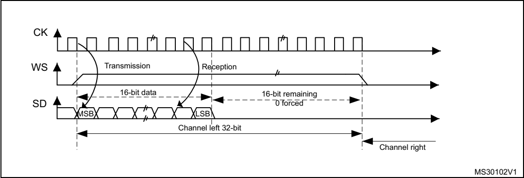
Figure 326. MSB justified 16-bit extended to 32-bit packet frame with CPOL = 0
