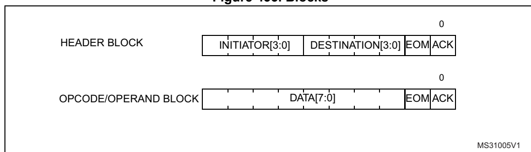
Figure 433. Blocks
