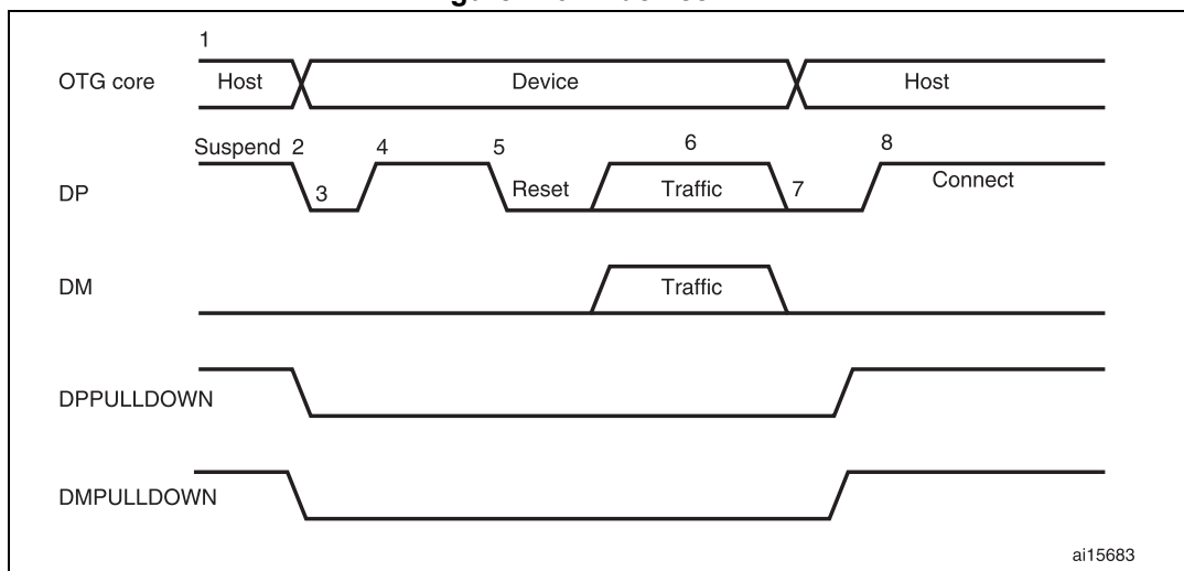
Figure 429. A-device HNP
