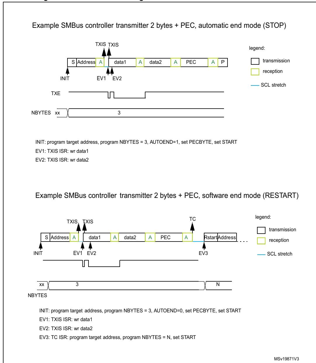
Figure 269. Bus transfer diagrams for SMBus controller transmitter
