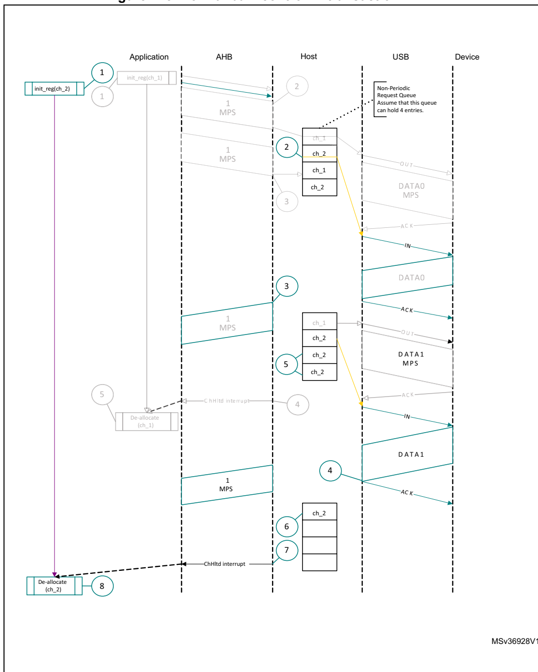
Figure 418. Normal bulk/control IN transaction - DMA
