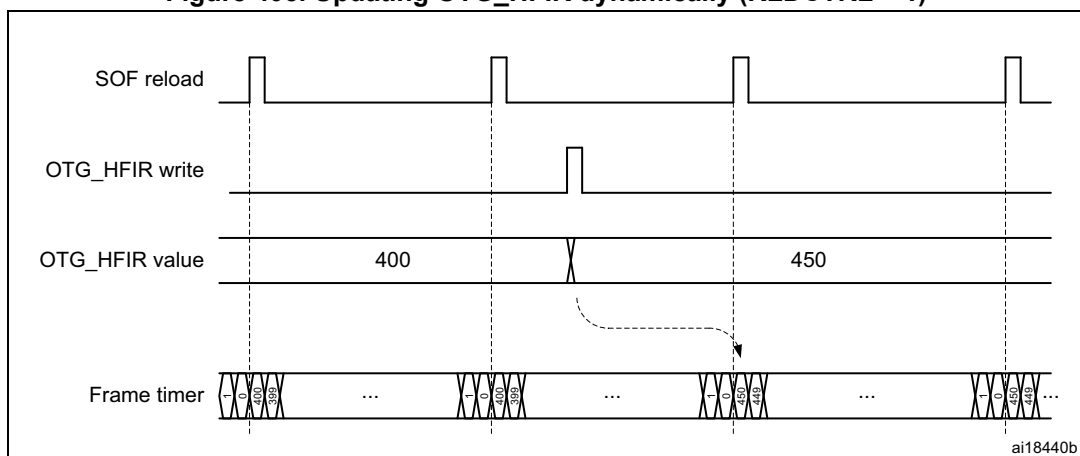
Figure 405. Updating OTG_HFIR dynamically (RLDCTRL = 1)
