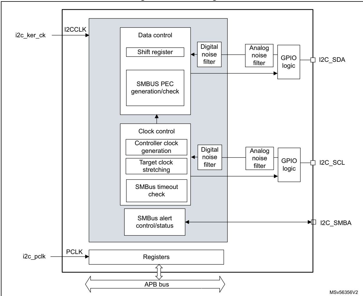
Figure 241. Block diagram
