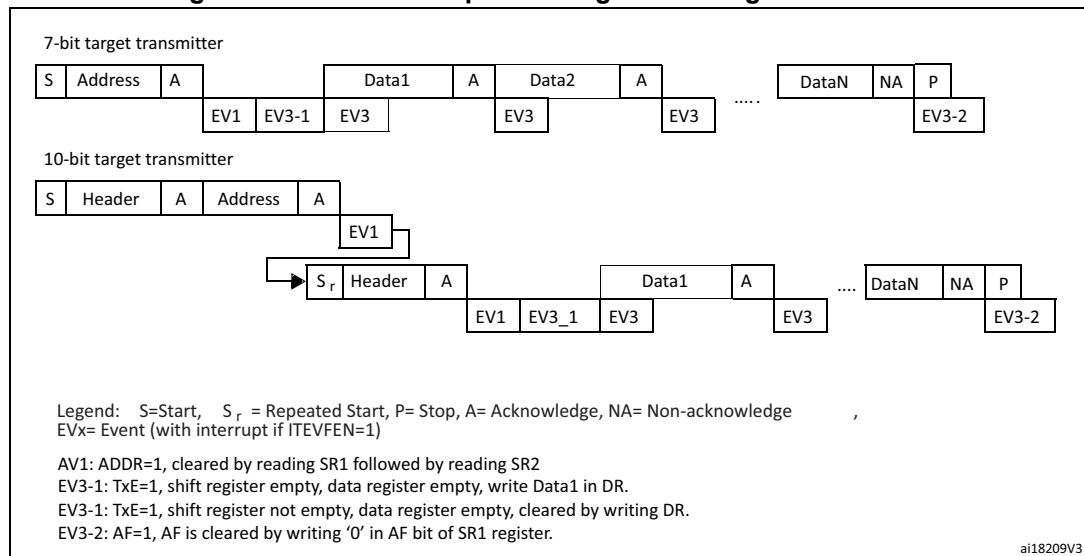
Figure 273. Transfer sequence diagram for target transmitter
