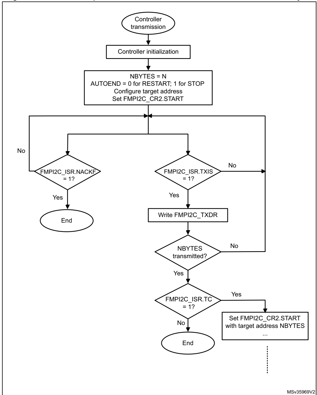
Figure 258. Transfer sequence flow for FMPI2C controller transmitter, N \leq 255 bytes
