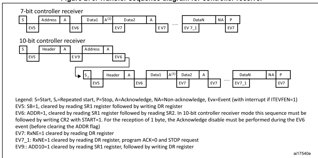
Figure 276. Transfer sequence diagram for controller receiver
