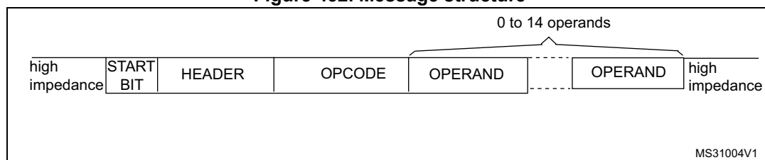
Figure 432. Message structure
