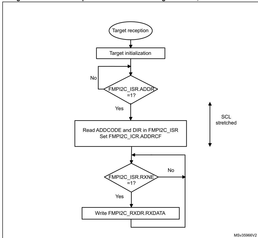
Figure 251. Transfer sequence flow for FMPI2C target receiver, NOSTRETCH = 0
