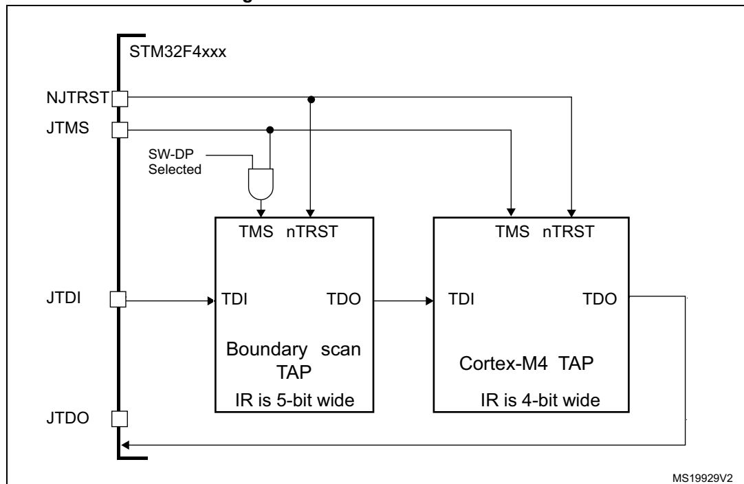
Figure 443. JTAG TAP connections
