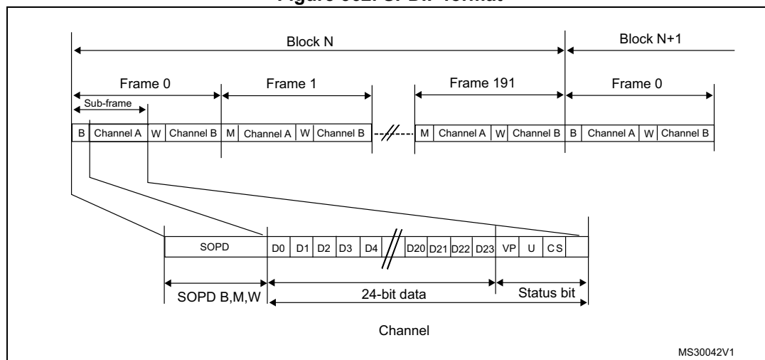
Figure 362. SPDIF format
