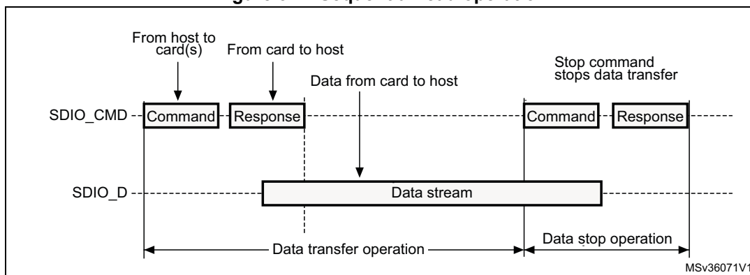
Figure 372. Sequential read operation
