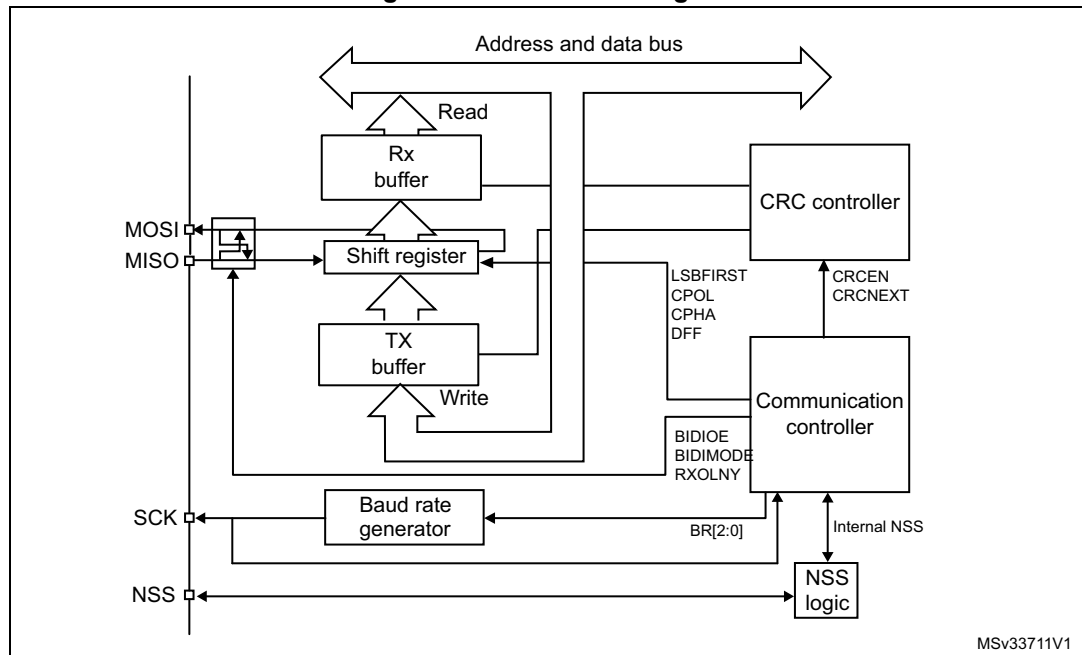
Figure 303. SPI block diagram
