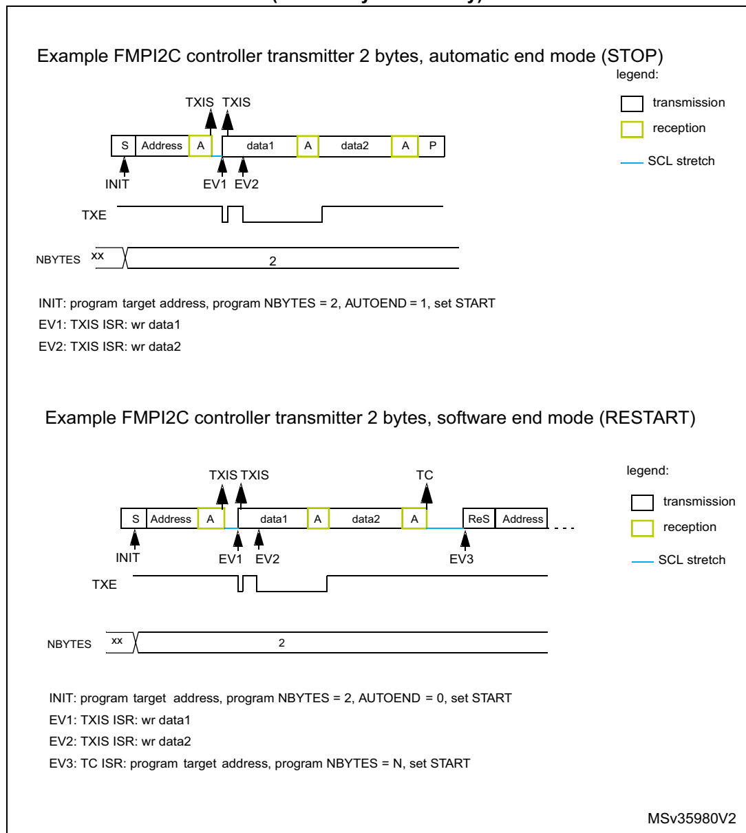
Figure 260. Transfer bus diagrams for FMPI2C controller transmitter (mandatory events only)
