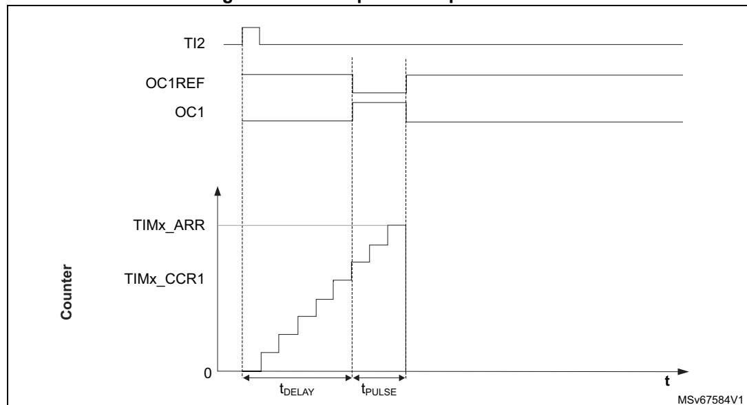
Figure 150. Example of one pulse mode
