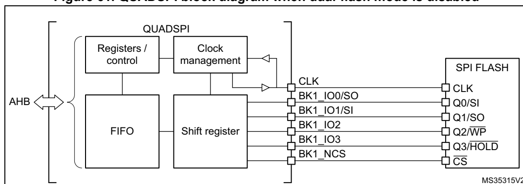
Figure 61. QUADSPI block diagram when dual-flash mode is disabled
