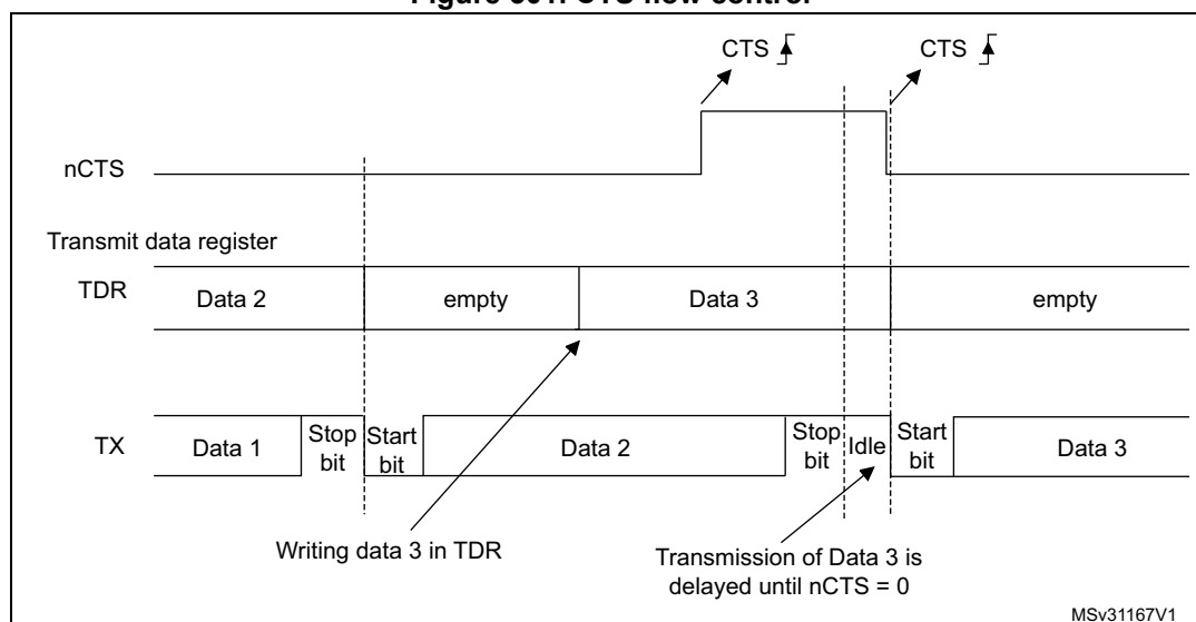
Figure 301. CTS flow control
