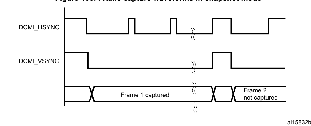
Figure 105. Frame capture waveforms in snapshot mode
