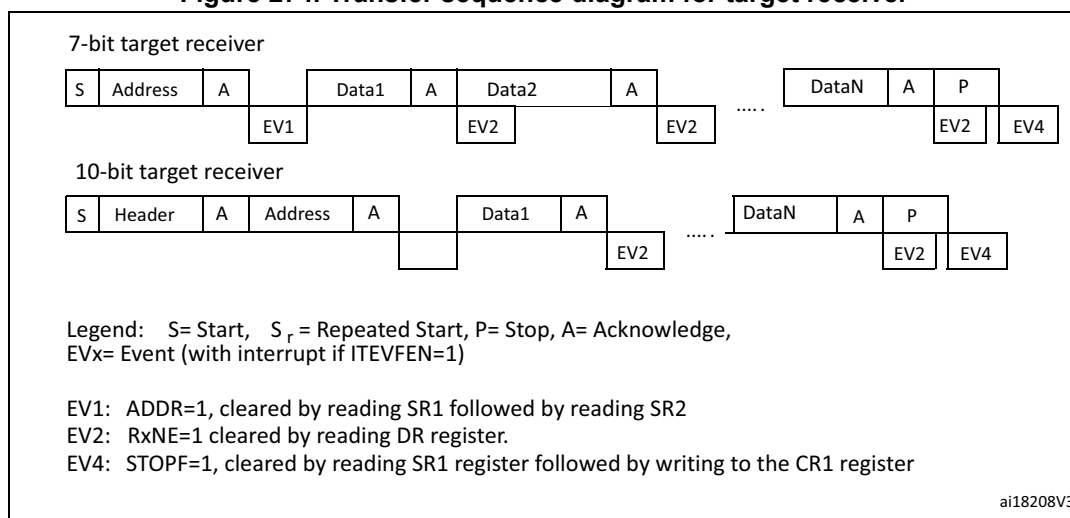
Figure 274. Transfer sequence diagram for target receiver
