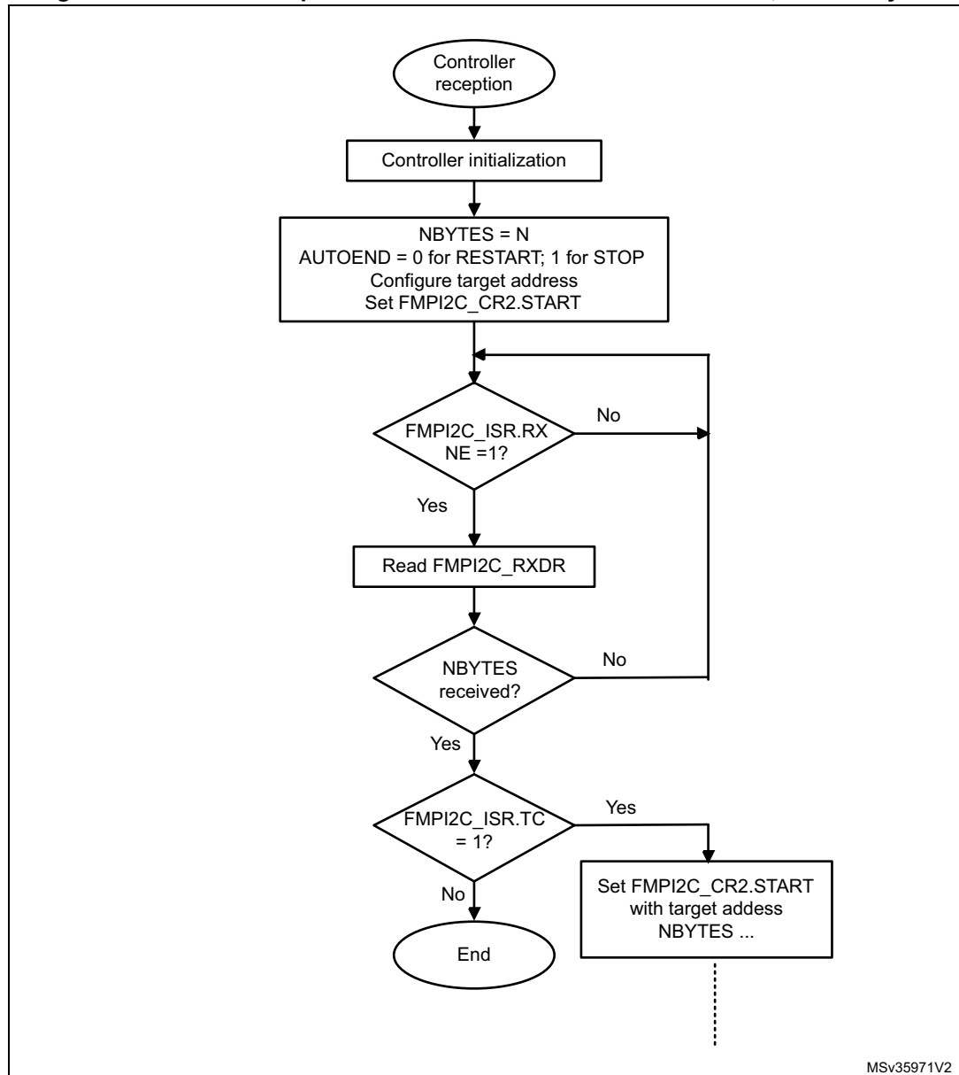
Figure 261. Transfer sequence flow for FMPI2C controller receiver, N \leq 255 bytes
