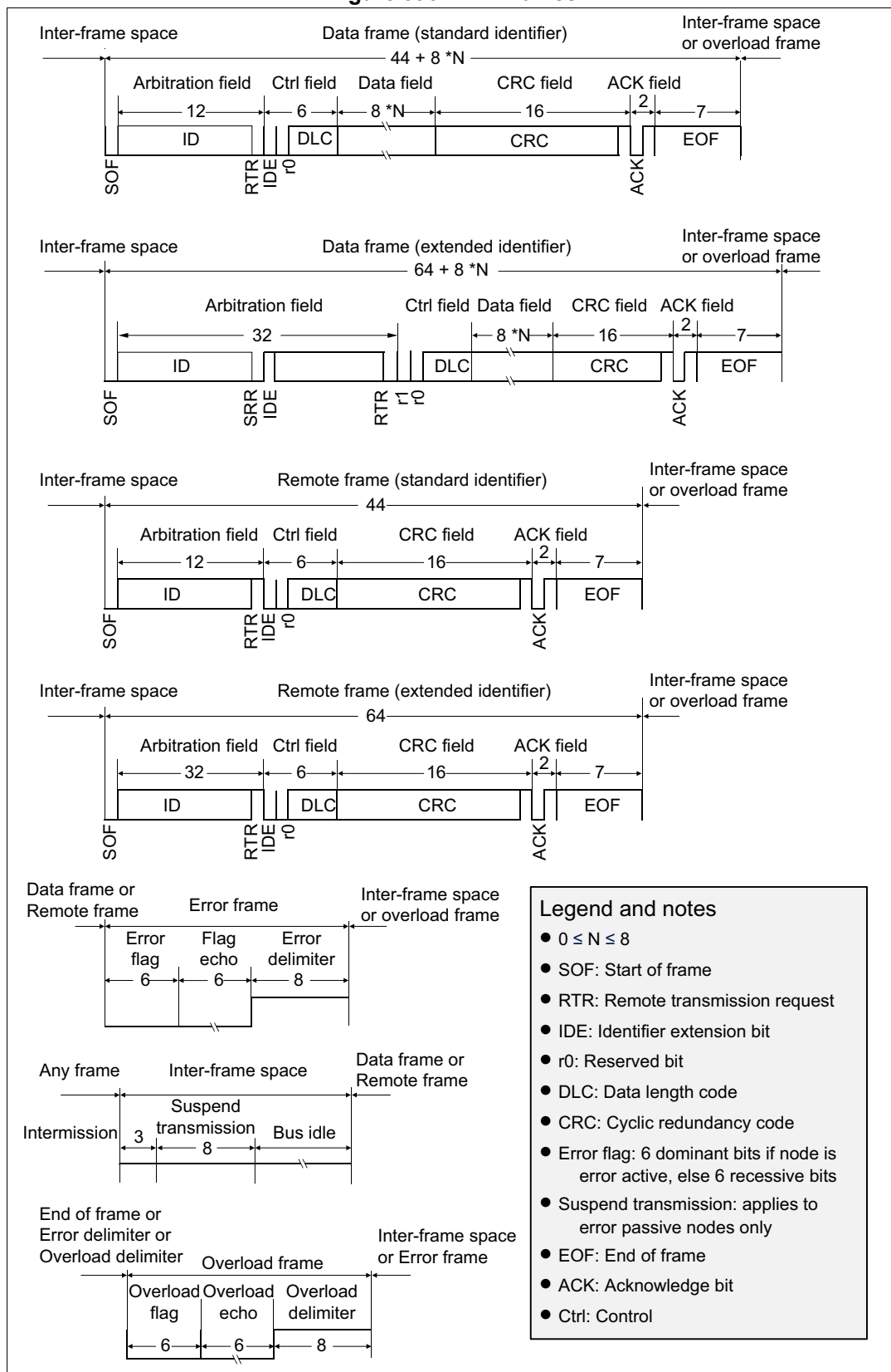
Figure 396. CAN frames
