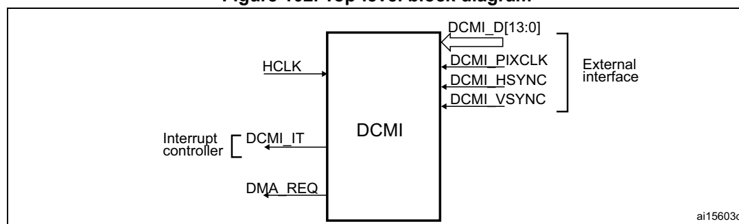
Figure 102. Top-level block diagram
