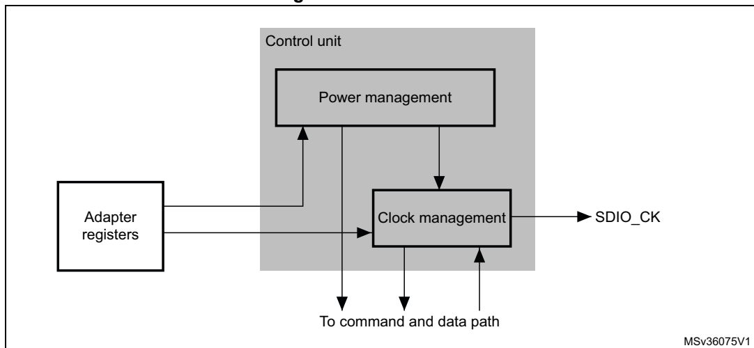
Figure 376. Control unit
