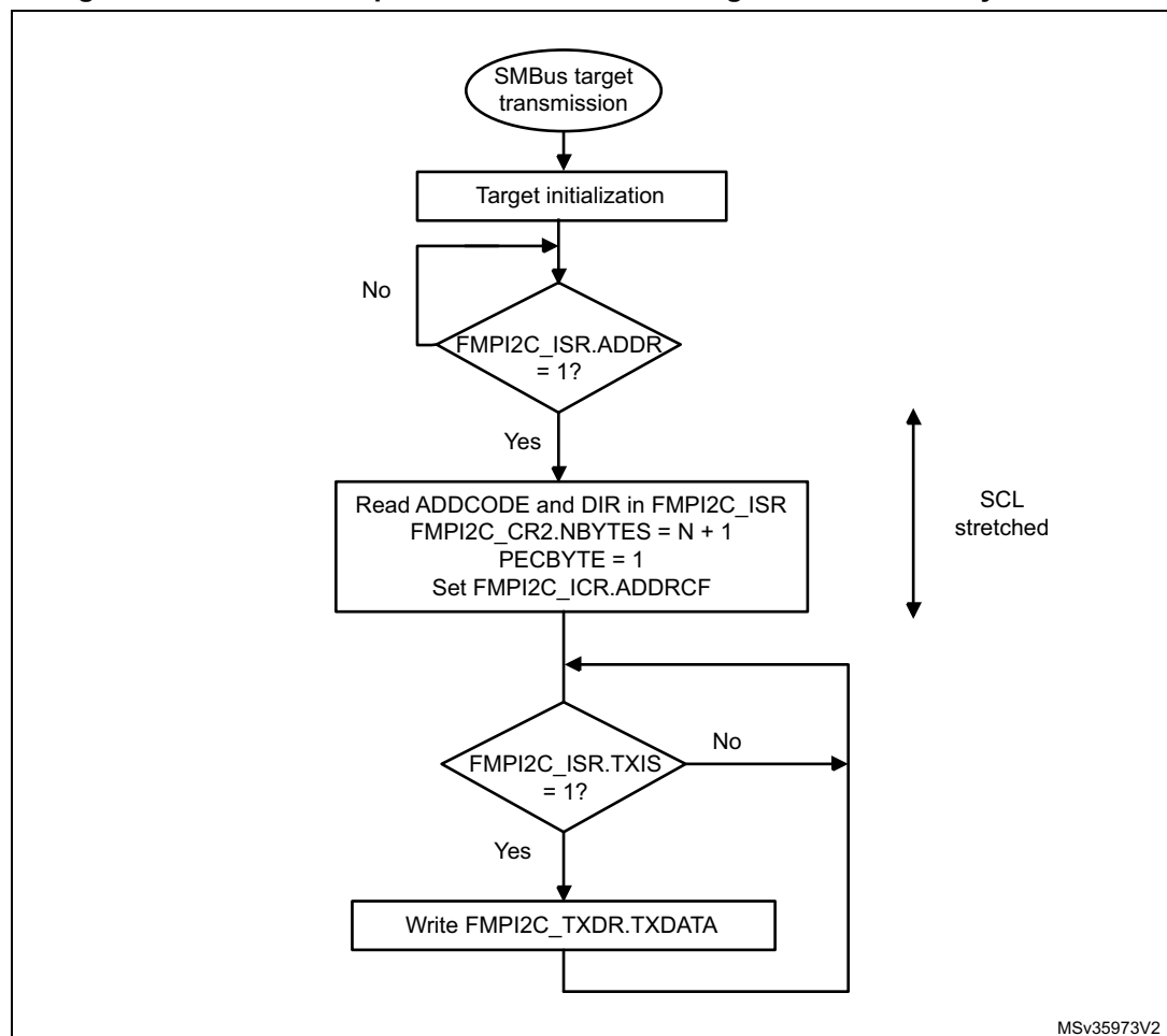
Figure 265. Transfer sequence flow for SMBus target transmitter N bytes + PEC
