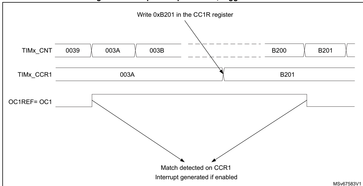
Figure 141. Output compare mode, toggle on OC1.
