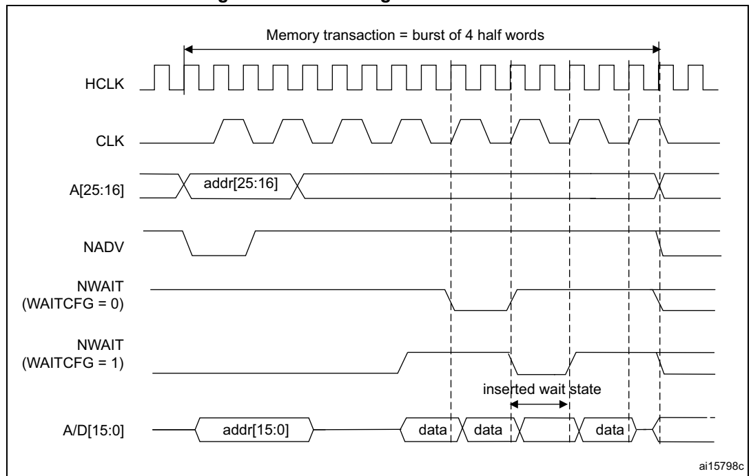
Figure 49. Wait configuration waveforms
