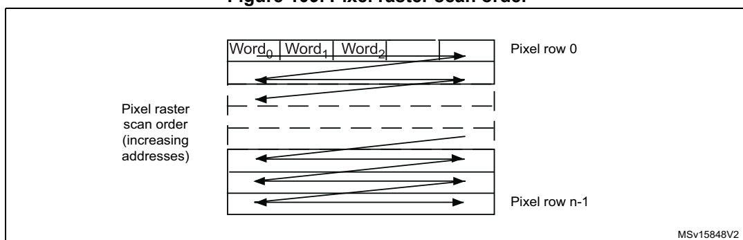
Figure 109. Pixel raster scan order
