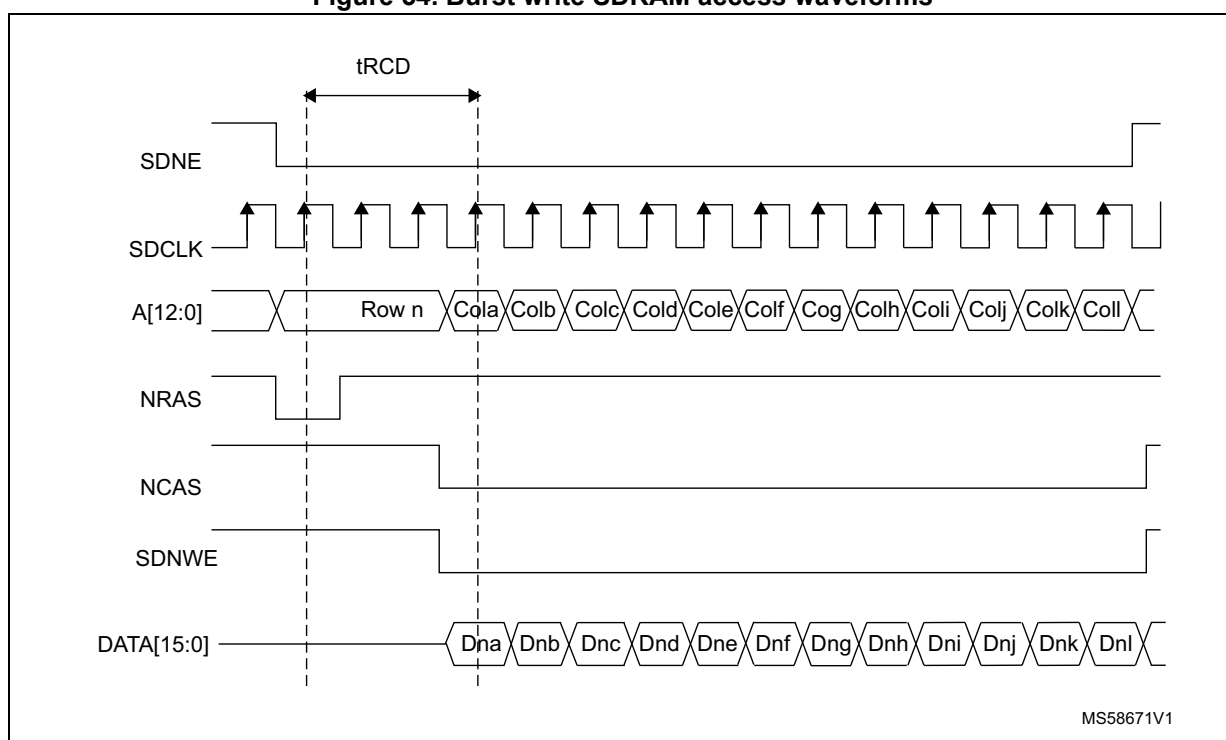
Figure 54. Burst write SDRAM access waveforms
