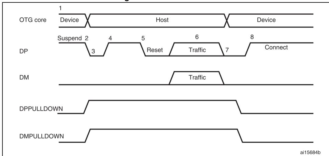
Figure 430. B-device HNP
