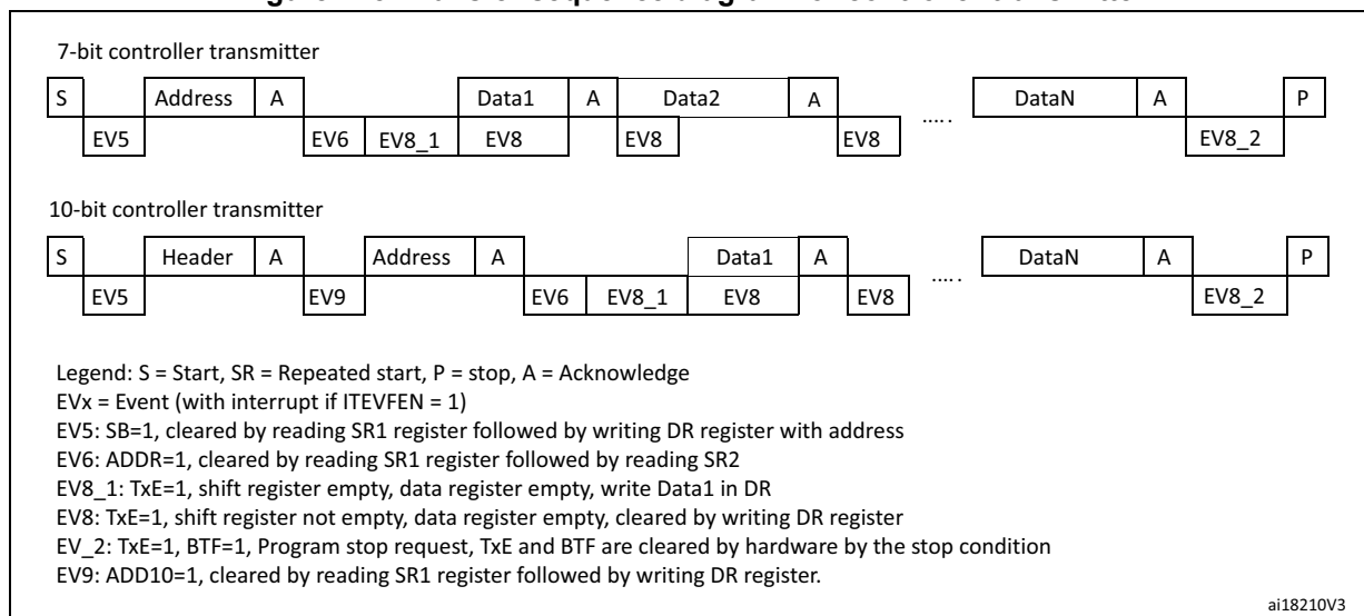
Figure 275. Transfer sequence diagram for controller transmitter
