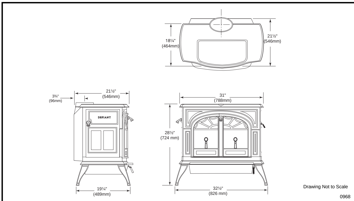
Fig. 1 Defiant dimensions.
