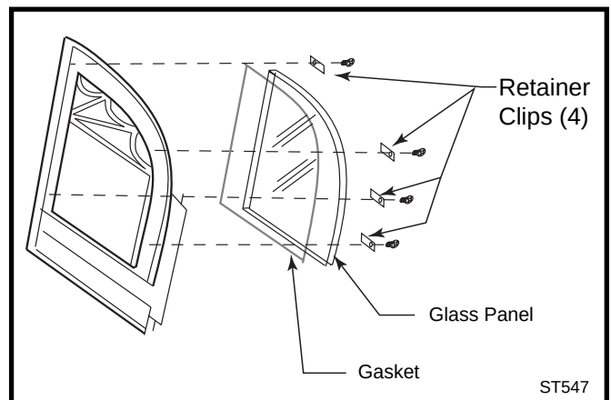
Fig. 32 An exploded view of the glass assembly on the left door.
