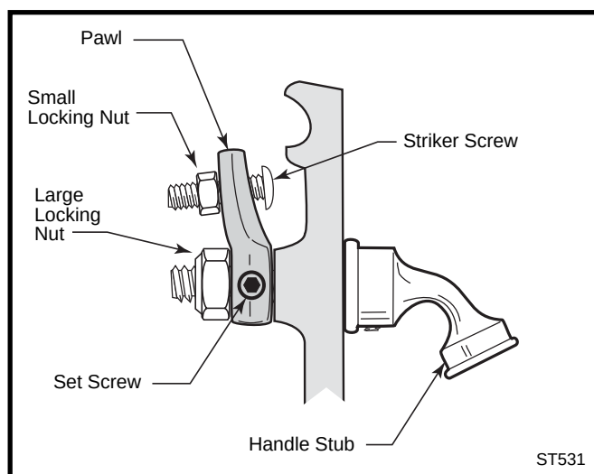
Fig. 35 Turn the door latch striker screw in or out to tighten or loosen the screw.
