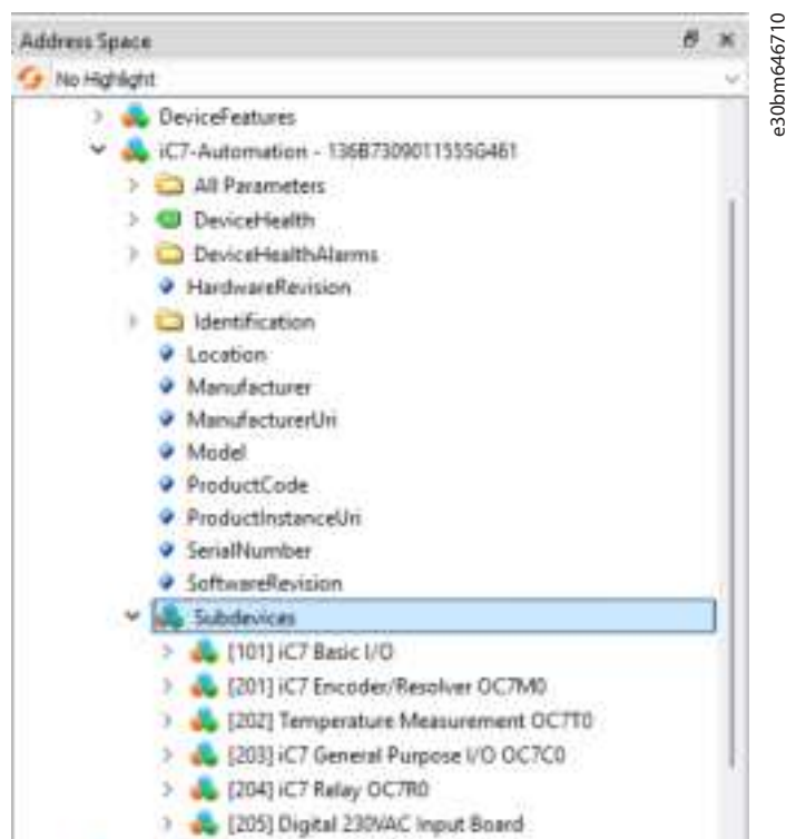
Figure 27: Subdevices View
