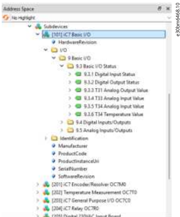
Figure 28: Example Functional Extension Options in Subdevices
