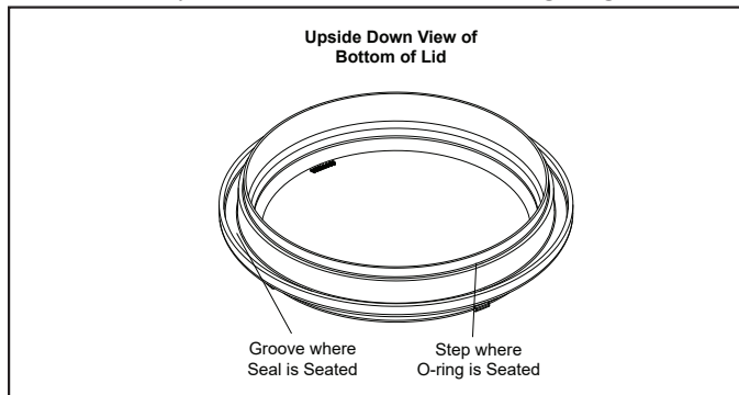
Figure 16. Placement of Blue Pressure Test O-ring
