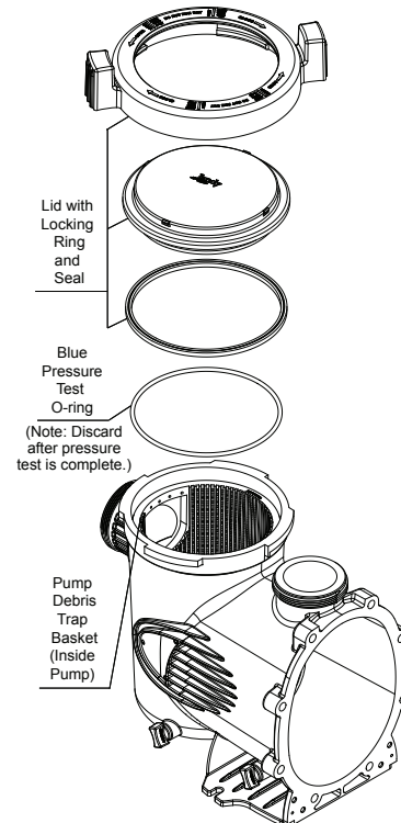
Figure 15. Exploded View with Blue Pressure Test O-ring (VSSHP Pump Models Only)
