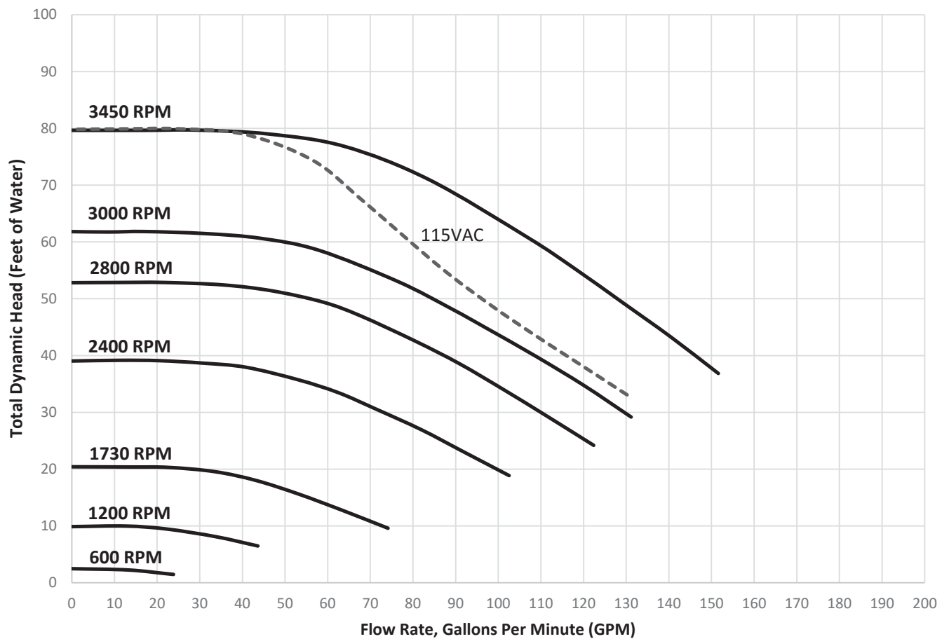
VSSH220DV2A(S) Performance Curves
