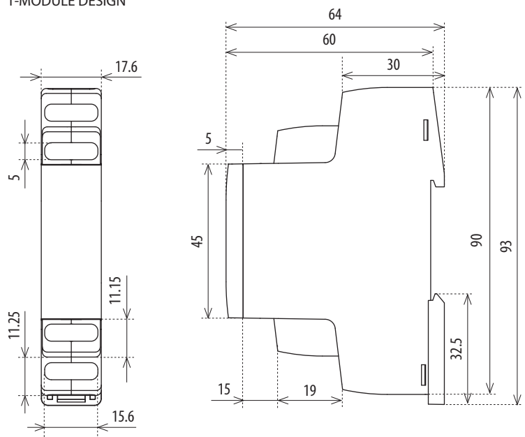
1-MODULE DESIGN
