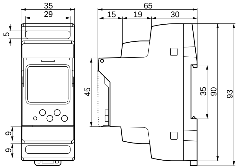
2-MODULE DESIGN
