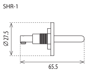
Level sensor
