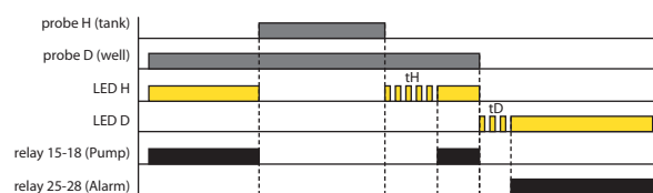
WELL - TANK, ON DELAY (Function 7)
