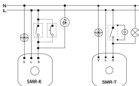
Typical wiring of SMR-K - timer for fan
