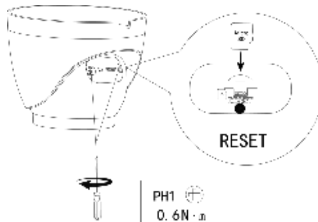
Figure 3-6 Install SD card
