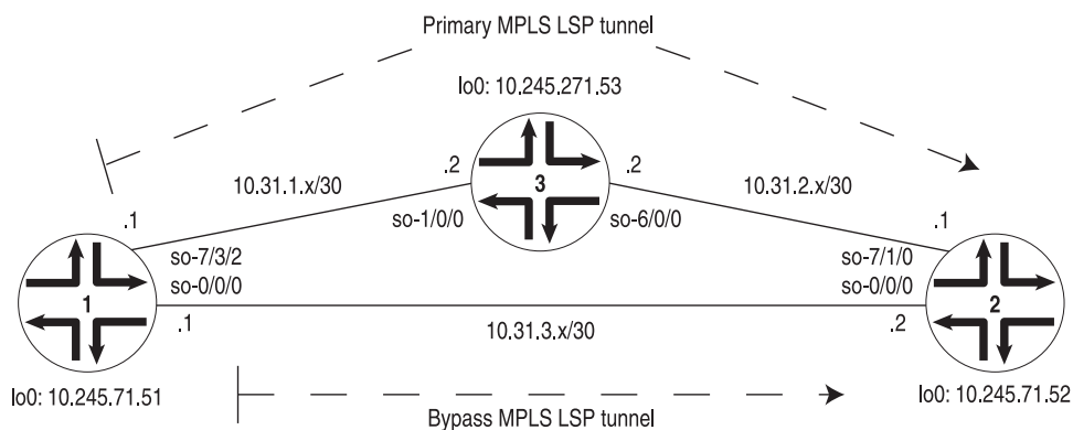
Figure 2: MPLS LSP Link Protection Topology Diagram
