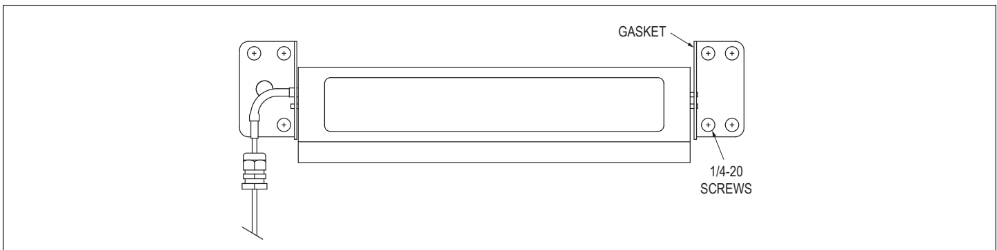
FIGURE 6 – FRONT VIEW
