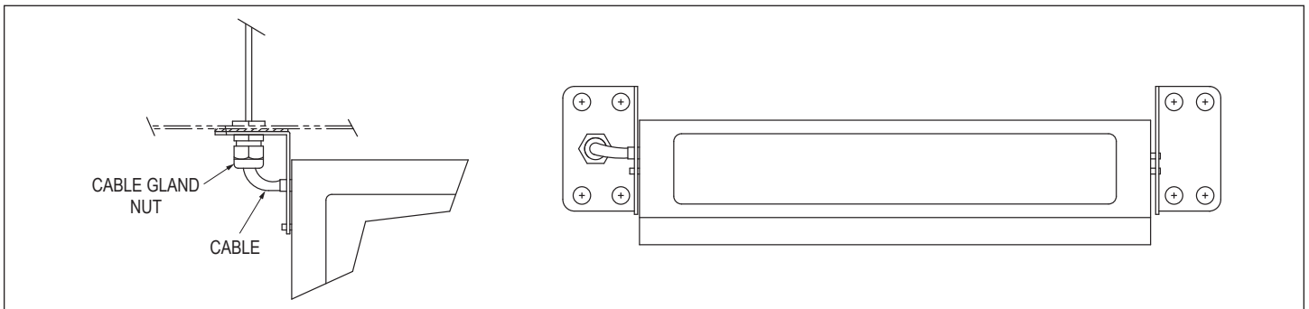
FIGURE 9 – TOP AND FRONT VIEWS
