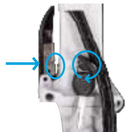
Locking Pin protruding through frame
