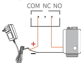
Connect the electric lock
