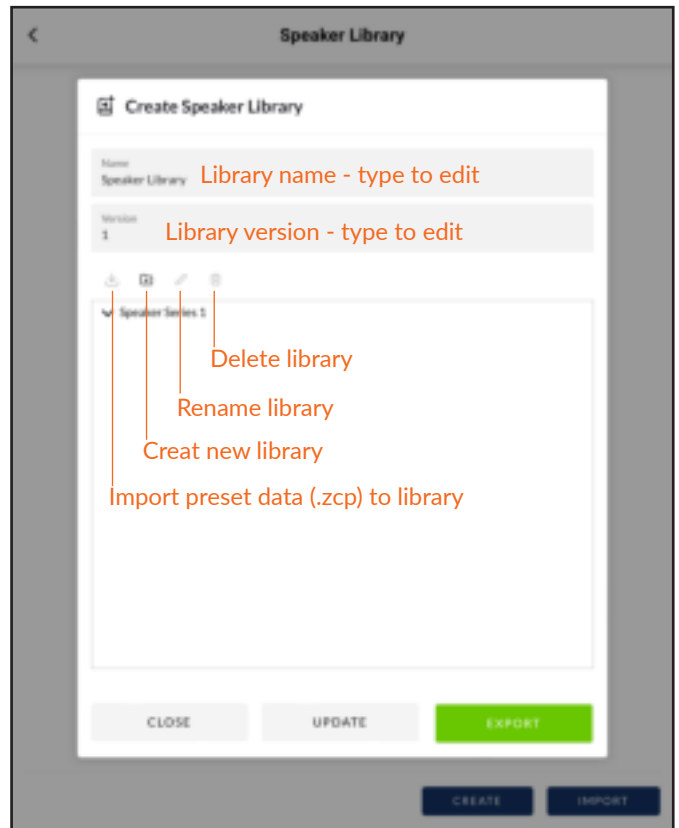
Diagram 5N Speaker Library Creation and Management
