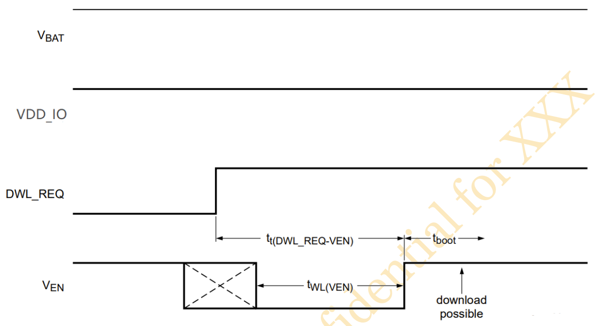
Figure 6 Download mode sequence
