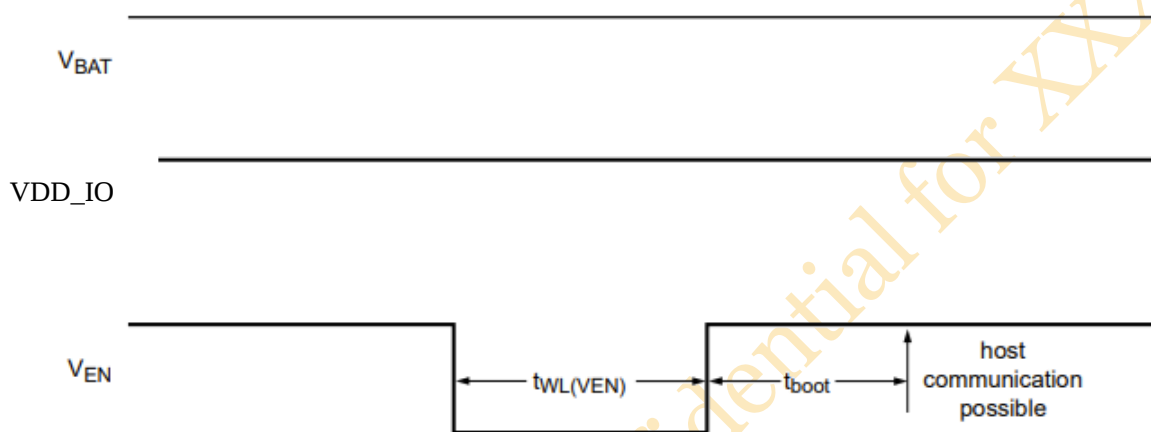
Figure 5 Reset via V_{EN} pin
