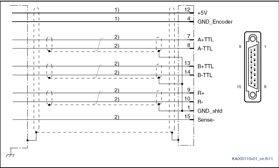
Fig. 7-7: Connection Diagram EC with TTL Encoder System
