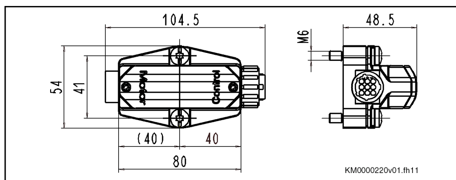
Fig. 8-8: Dimensions
