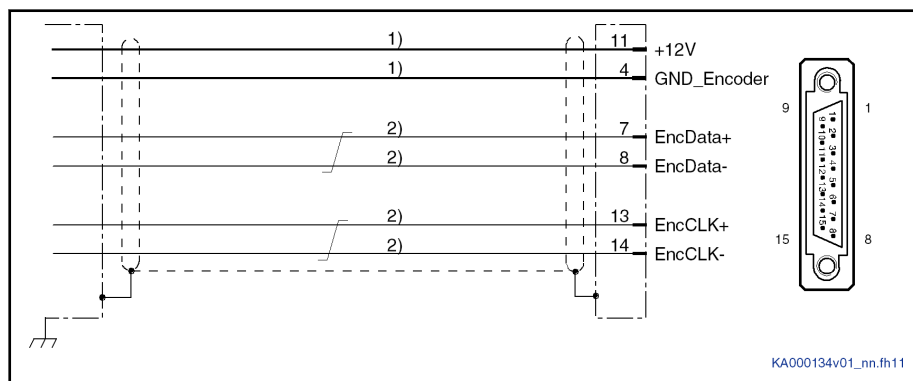
Fig. 7-10: Connection Diagram SSI Encoder System
