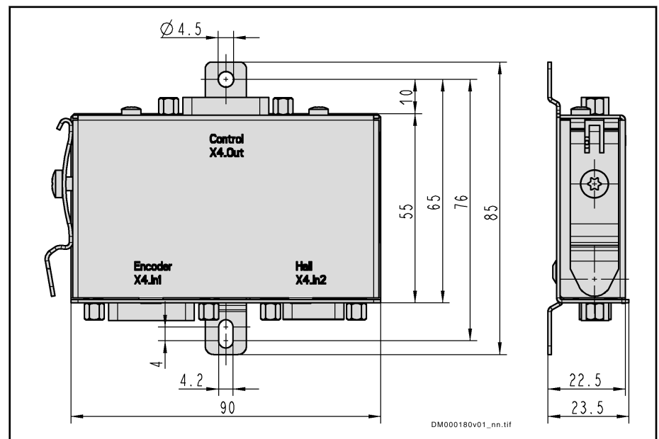
Fig. 8-24: Dimensions
