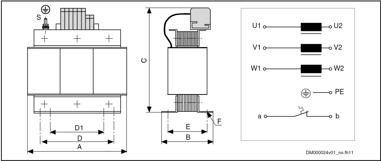
Fig.8-43: Dimensions Type 1
