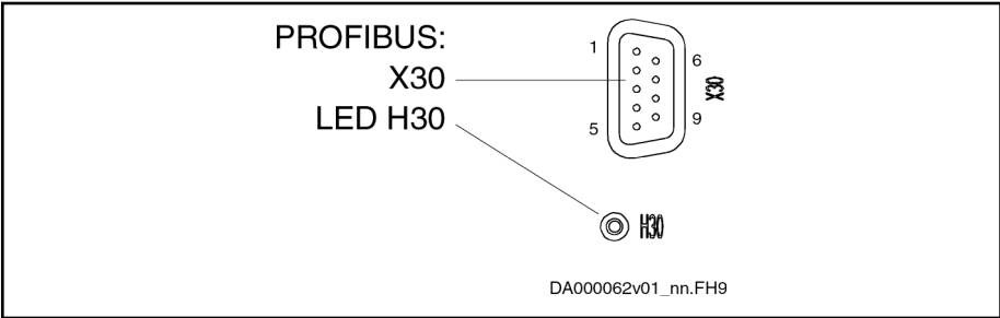
Fig.6-14: PROFIBUS Interface
