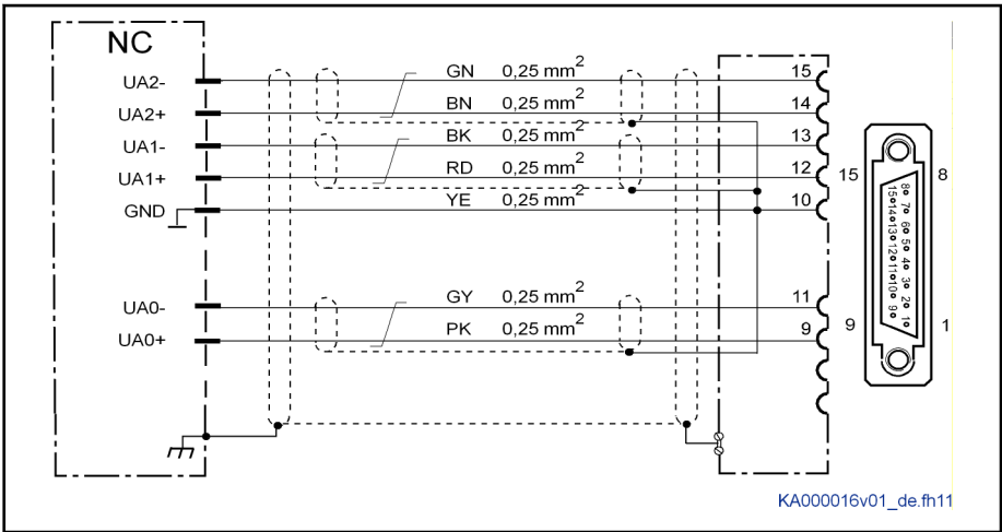
Fig.7-19: Connection of Incremental Actual Position Value Output
