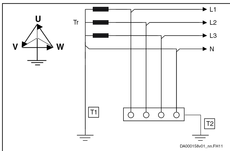
Fig. 4-20: TT Mains System
