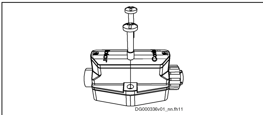
Fig. 8-6: Battery Box
