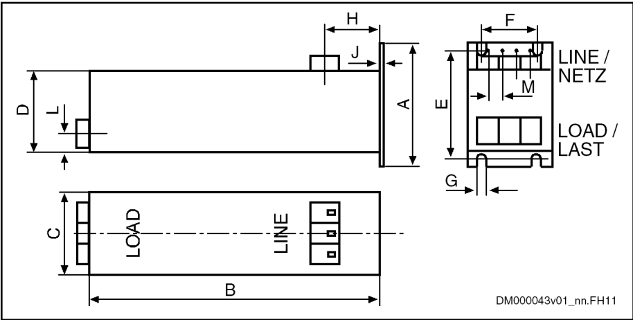
Type NFE02.1-230-008 (with 3 terminal connectors) Fig. 8-39: Single-Phase Filter NFE02.1 for Drives
