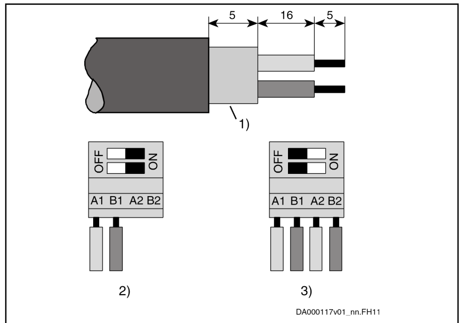
Fig. 6-15: Preparing a Cable for Connecting a Bus Connector
