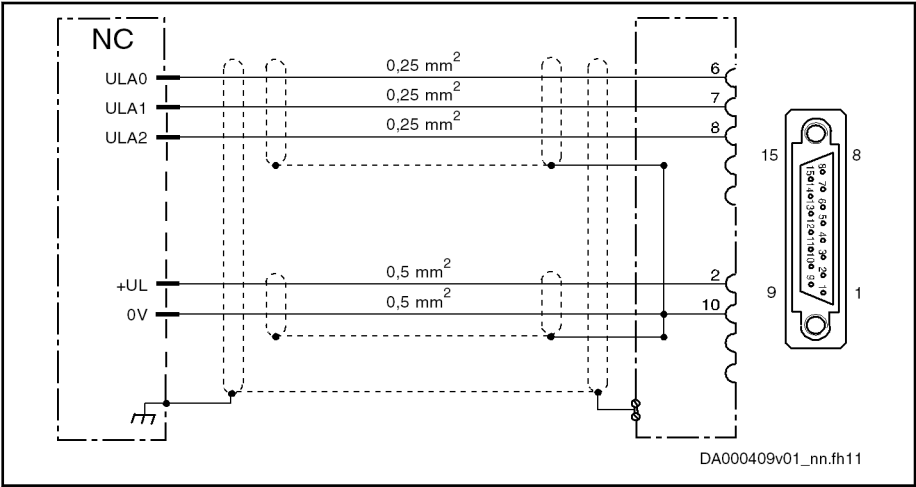
Fig. 7-22: Connection
