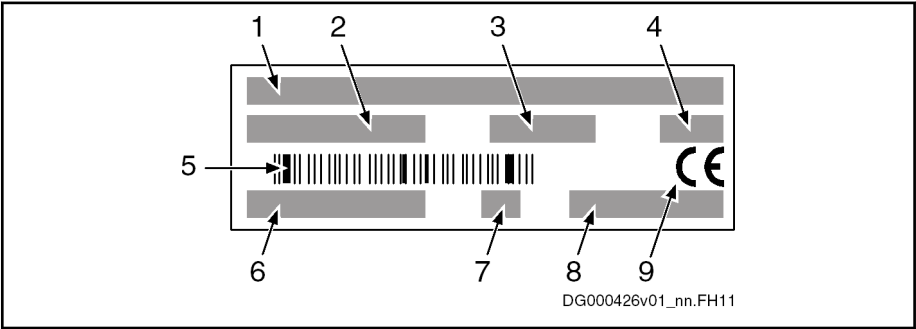
1 Device type 2 Part number 3 Production week; 11W36, for example, means year 2011, week 36 4 Factory identifier 5 Bar code 6 Serial number 7 Hardware index 8 Country of manufacture 9 Identification Fig.5-2: Type Plate (Device)
