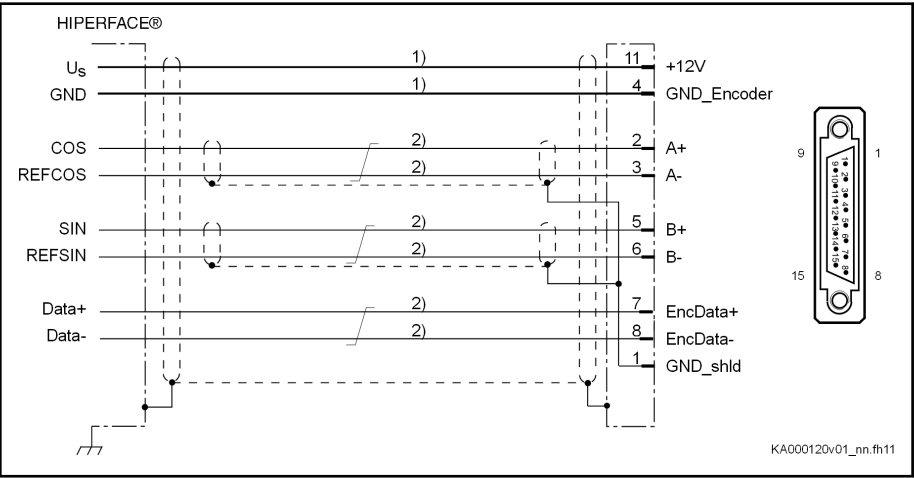
Fig. 7-3: Connection Diagram HIPERFACE® Encoder System
