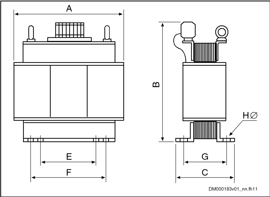
Fig.8-34: Dimensional Drawing
