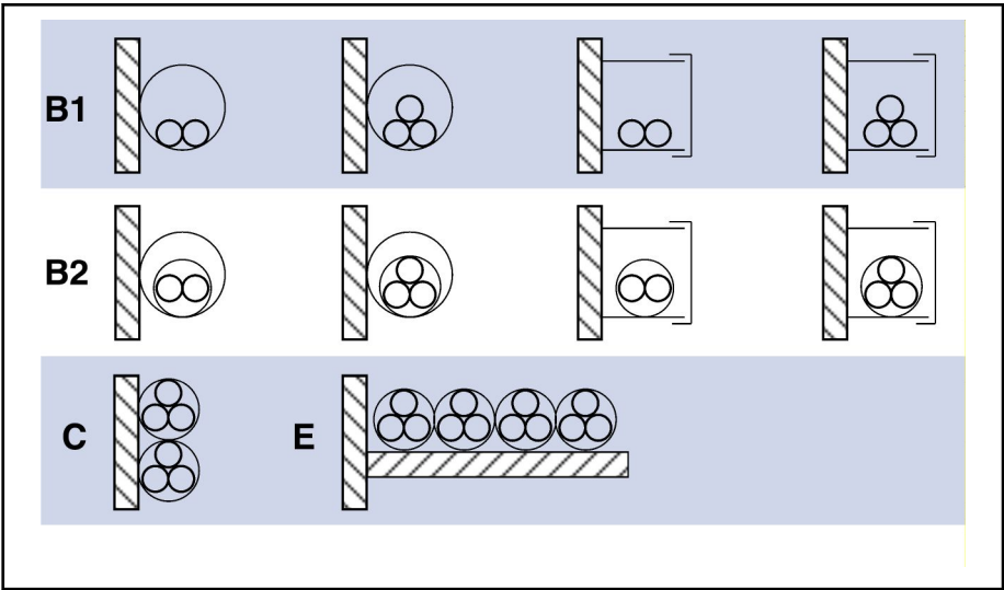
B1 Conductor in installation pipes and in installation channels to be opened B2 Cables or lines in installation pipes and in installation channels to be opened C Cables or lines on walls E Cables or lines on open cable trays. Fig. 11-1: Installation methods (compare IEC 60364-5-52; VDE0298-7; EN 60204-1)
