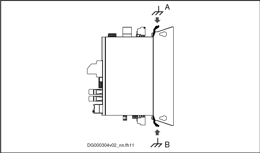
Fig.6-11: Shield Connection
