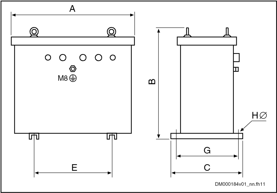
Fig.8-36: Dimensional Drawing
