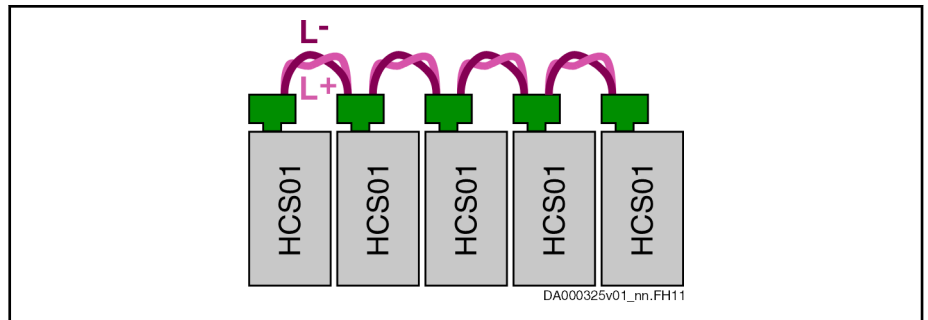
Fig.4-34: Looping Through via DC Bus Connector
