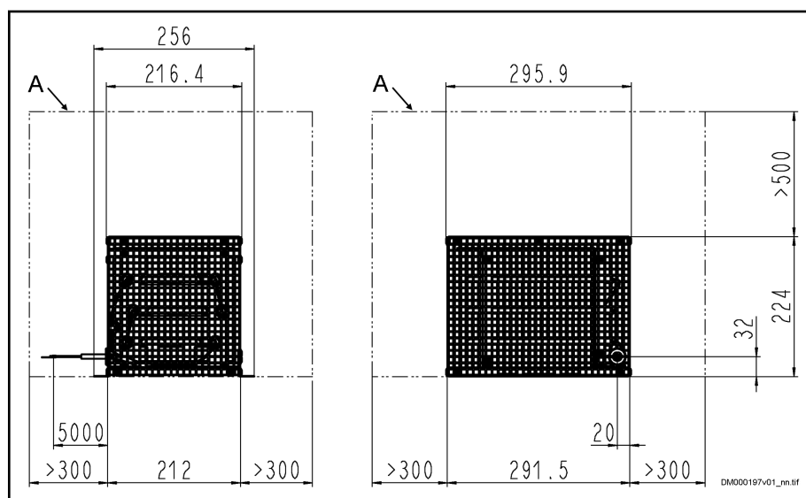
Fig. 8-47: Dimensions (with Upright Mounting on the Floor)
