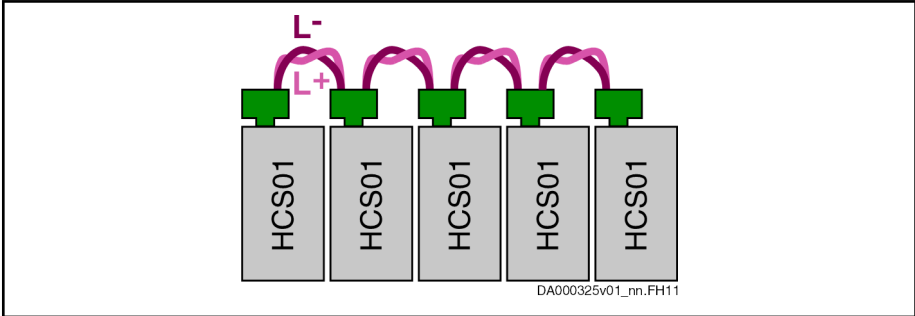
Fig.8-5: Connecting the DC Buses via DC Bus Connectors
