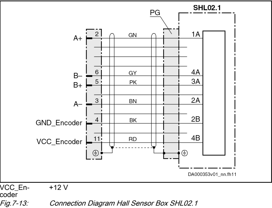
Connection Diagram
