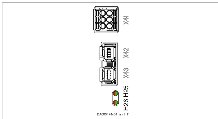
H26, H25 Bicolor LEDs Fig. 7-27: Safe Motion, Display Elements
