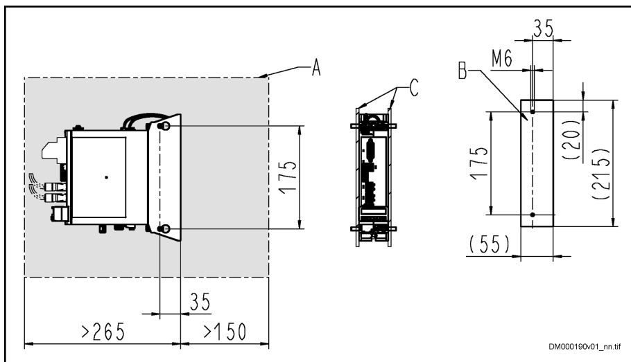
Fig. 4-5: Dimensional Drawing HCS01.1E-W0003/5/6/8/9/13 (Left-Hand or Right-Hand Mounting)
