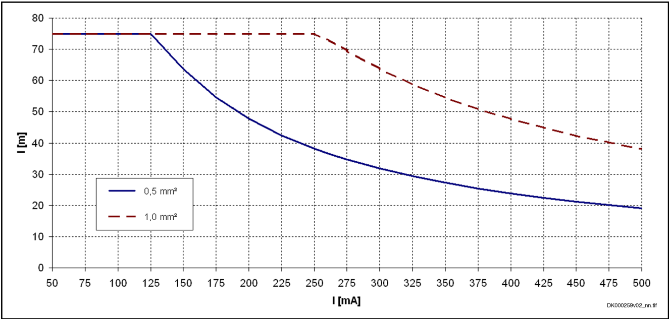
I [mA] Encoder current consumption l [m] Cable Length 0.5 mm²; 1.0 mm² Line Cross Sections Fig. 7-15: Maximum Allowed Encoder Cable Lengths for 12 V Encoder Systems Depending on Line Cross Section at a Supply Voltage of 10 V
