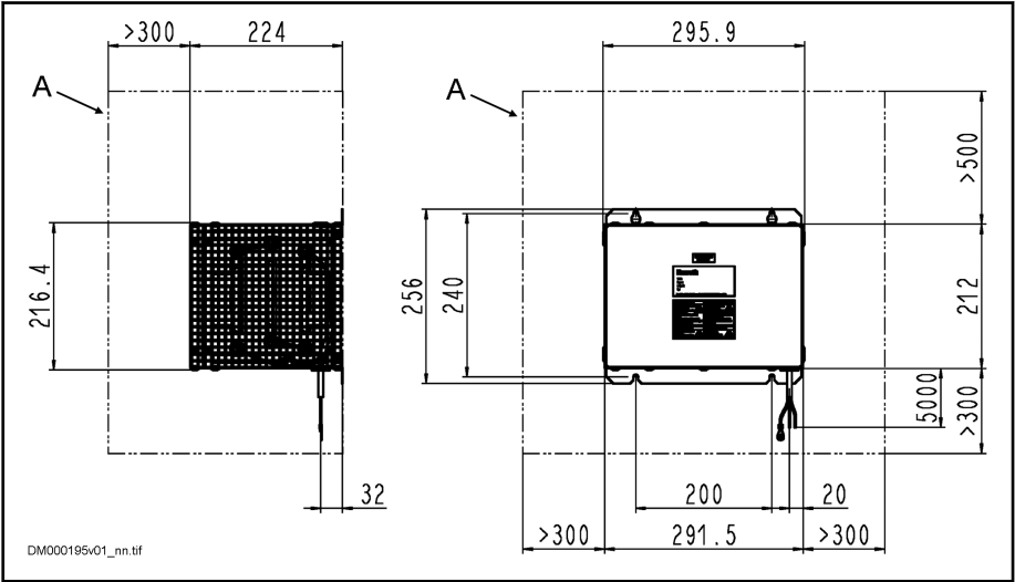
A Minimum mounting clearance Fig. 8-46: Dimensions (with Suspended Mounting on the Wall)
