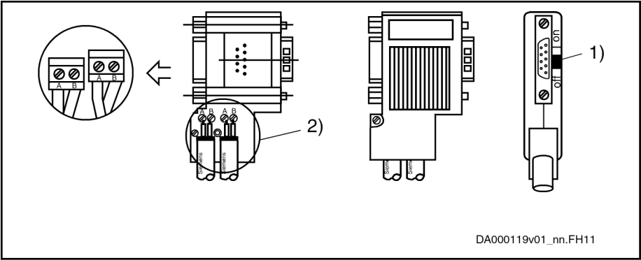
1) Terminating resistor is off 2) Cable shield must have direct contact to metal Fig.6-17: Bus Connection for all Other Slaves, Bus Connector With 9-pin D-Sub Female Connector, INS0541
