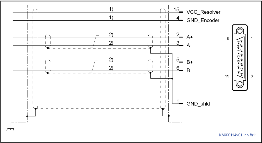
Connection Diagram
