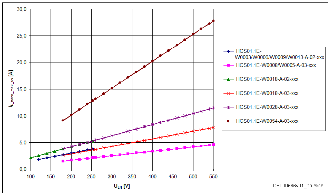
I_{L\_trans\_max\_on} Maximum inrush current U_{LN} Mains Voltage Fig.7-39: Maximum Inrush Current vs. Mains Voltage
