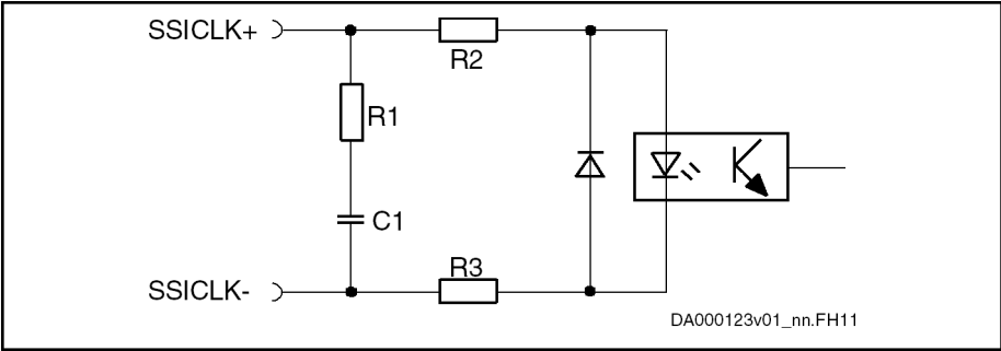
Fig.7-24: Differential Input Circuit (Block Diagram)
