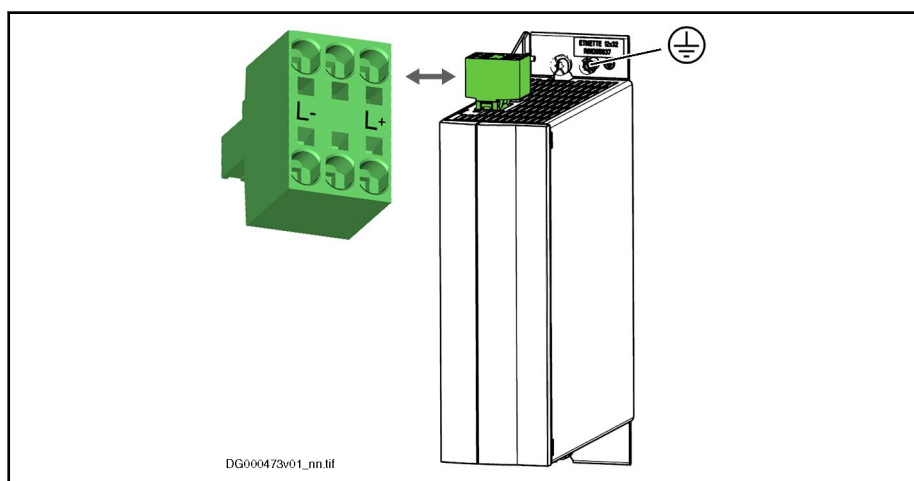
Fig. 8-51: Connection Points (DC Bus (L+ L-), Equipment Grounding Conductor)
