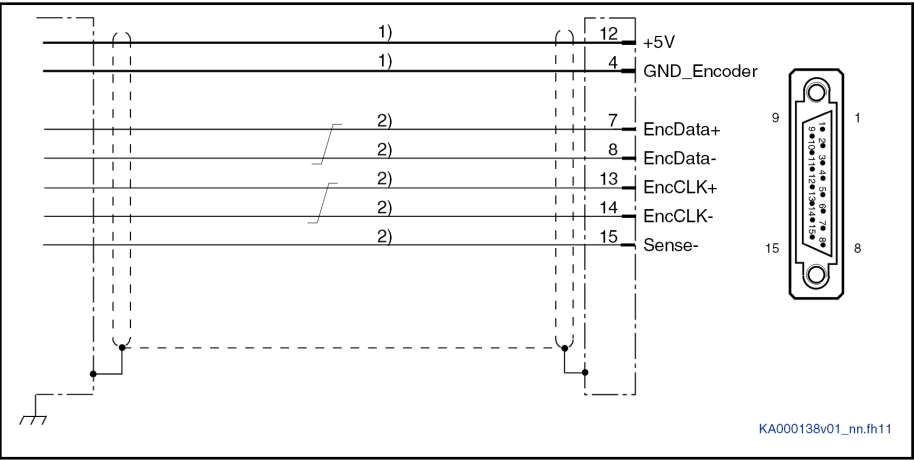
Fig. 7-9: Connection Diagram EC with SSI Encoder System
