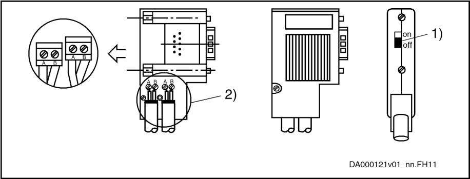
1) Terminating resistor is off 2) Cable shield must have direct contact to metal Fig.6-19: Bus Connection for all Other Slaves, Without 9-pin D-Sub Female Connector, INS0540
