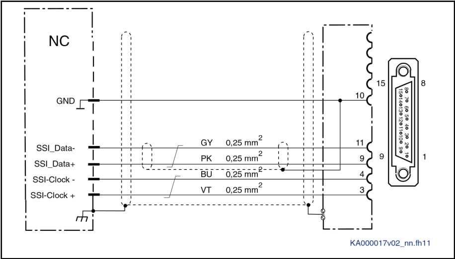
Fig. 7-23: Output of Absolute Actual Position Values According to SSI Format
