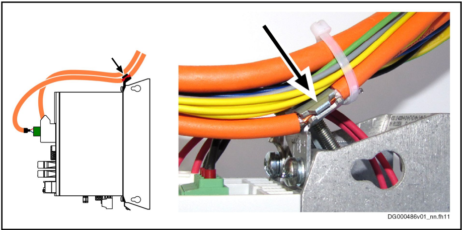
Fig. 8-16: Shield Connection of Shielded Lines at the Top of the Device
