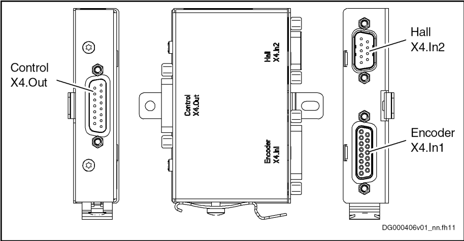
Fig.8-25: Connection Points
