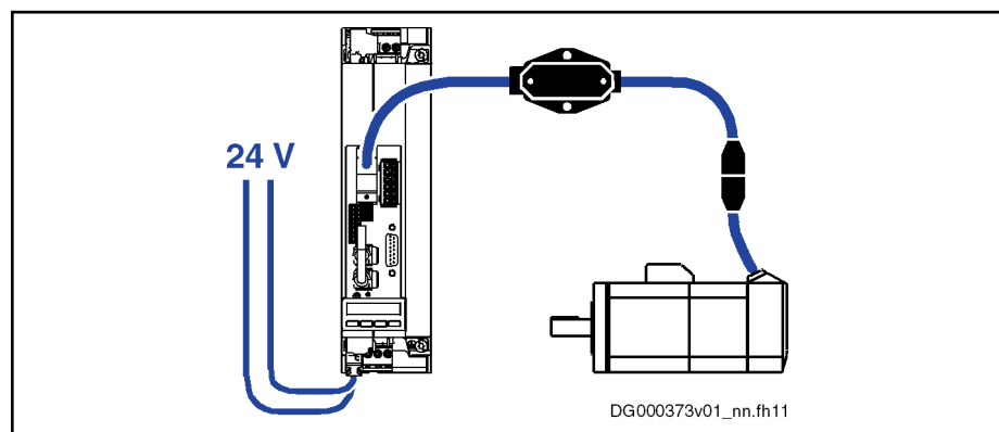
Fig. 8-13: Control Voltage Switched On and Encoder Connected
