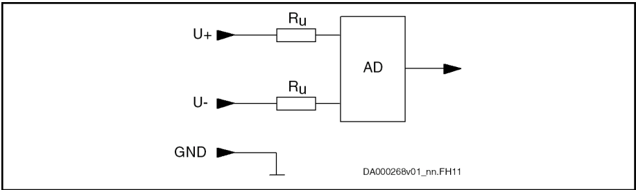
AD Analog/digital converter Fig. 7-34: Analog Voltage Input
