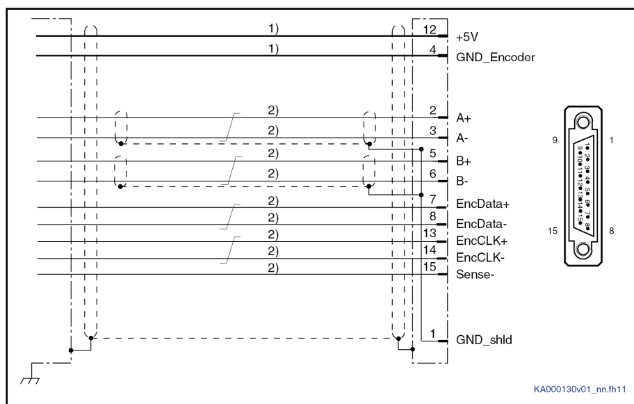
Fig. 7-4: Connection Diagram EC with EnDat 2.1 Encoder System
