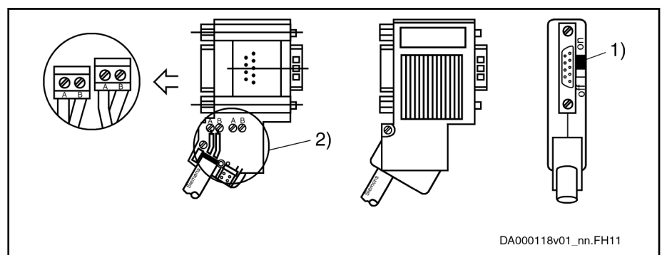
Fig. 6-16: Bus Connection for First and Last Slave, Bus Connector With 9-pin D-Sub Female Connector, INS0541
