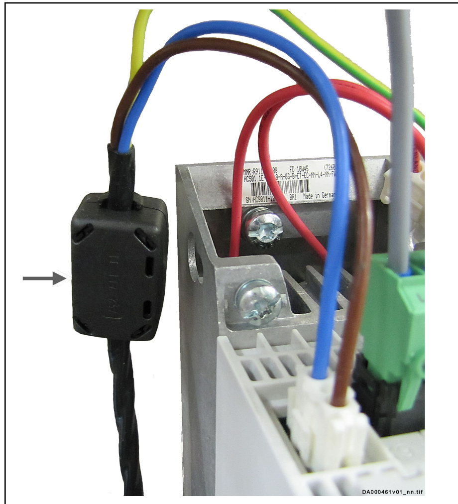
Fig.8-31: Snap-On Ferrite at Connection Line of External Braking Resistor
