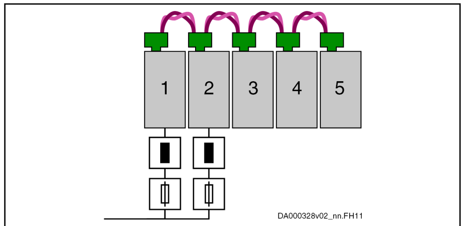
Fig.4-35: Looping Through
