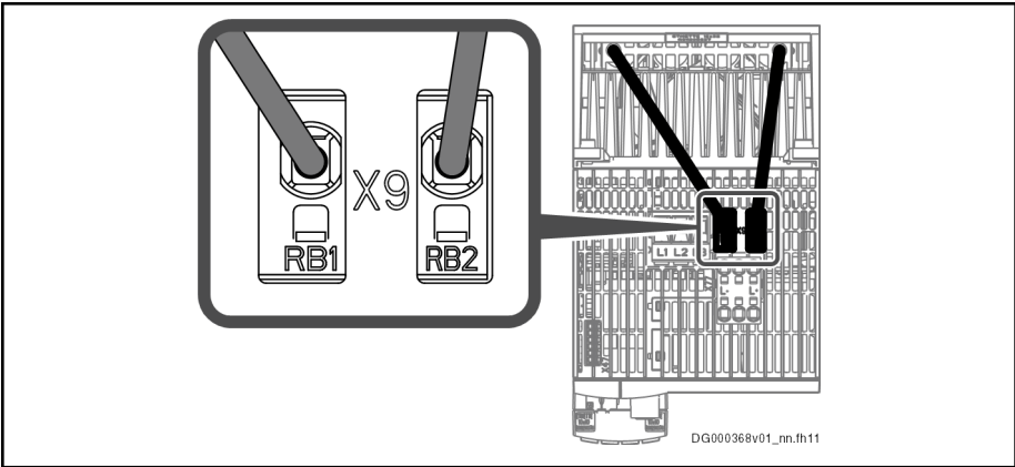
Fig.6-8: Connecting the Braking Resistor (HCS01.1E-W0054)
