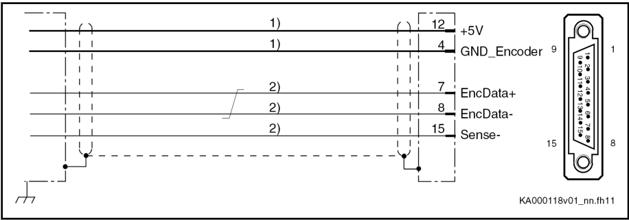
Fig. 7-1: Connection Diagram EC with Encoder System of IndraDyn S MSM Motors
