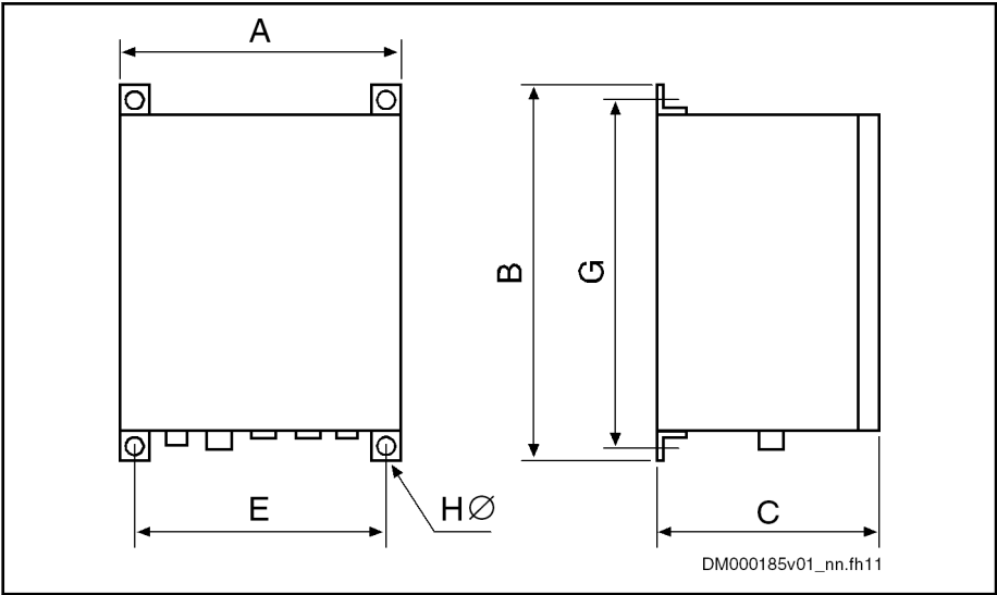
Fig.8-35: Dimensional Drawing
