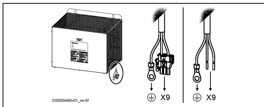
Fig. 8-48: Connection
