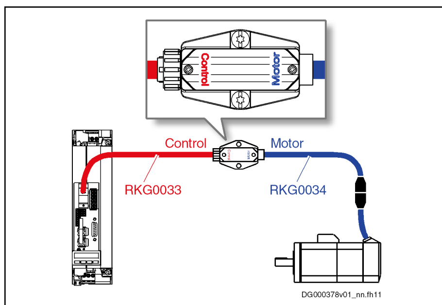
Fig. 8-10: Cabling of the Battery Box
