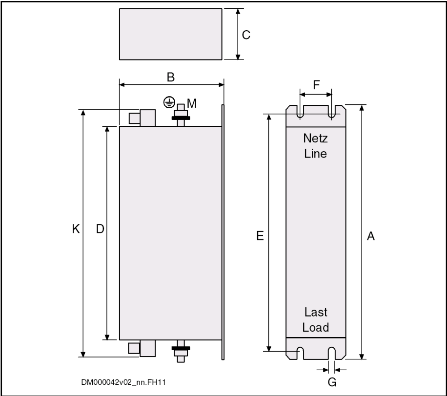
Fig.8-40: Three-Phase Current Filter NFD03.1 for Drives
