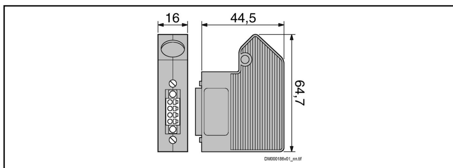
Fig. 8-20: Dimensions
