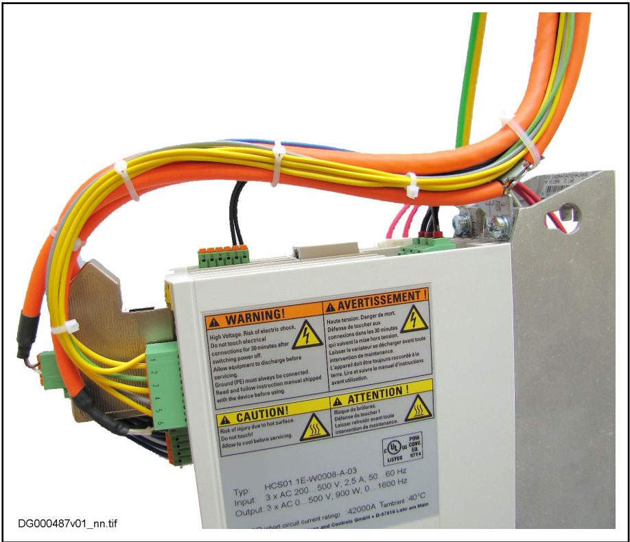
Fig. 8-17: Example of a Complete Wiring
