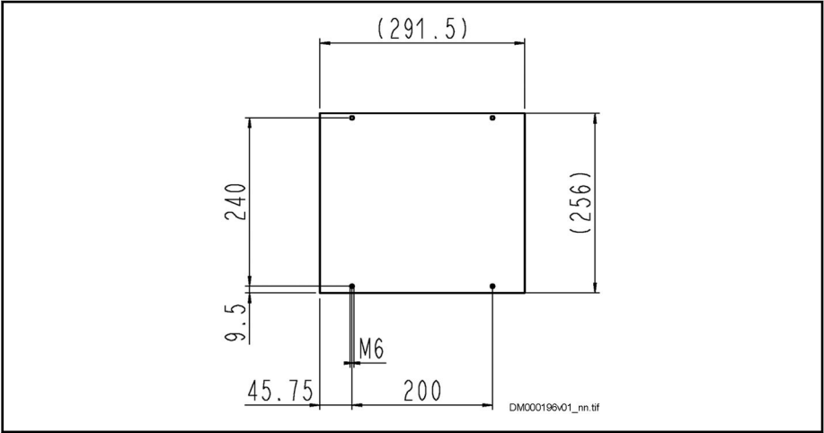
Fig. 8-45: Boring Dimensions
