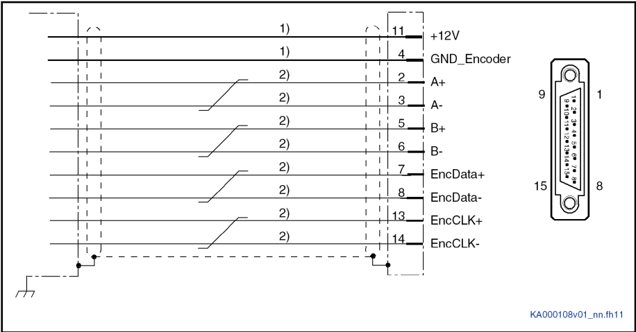
1) Line cross section \geq 0.5 \text{ mm}^2 ; observe allowed encoder cable length 2) Line cross section \geq 0.14 \text{ mm}^2 Fig. 7-2: Connection Diagram MSK/QSK Encoder Interface for S1/M1, S2/M2, S5/M5 Encoder Systems
