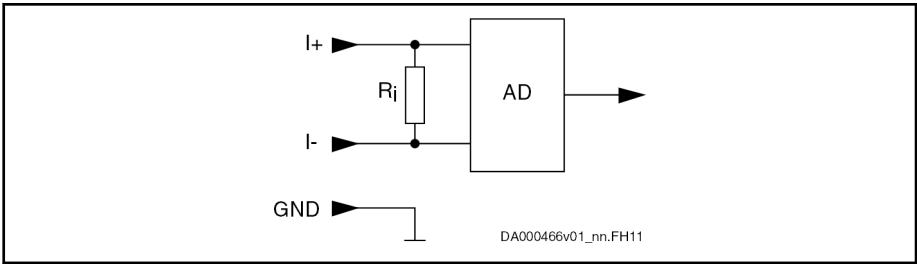
AD Analog/digital converter Fig. 7-35: Analog Current Input
