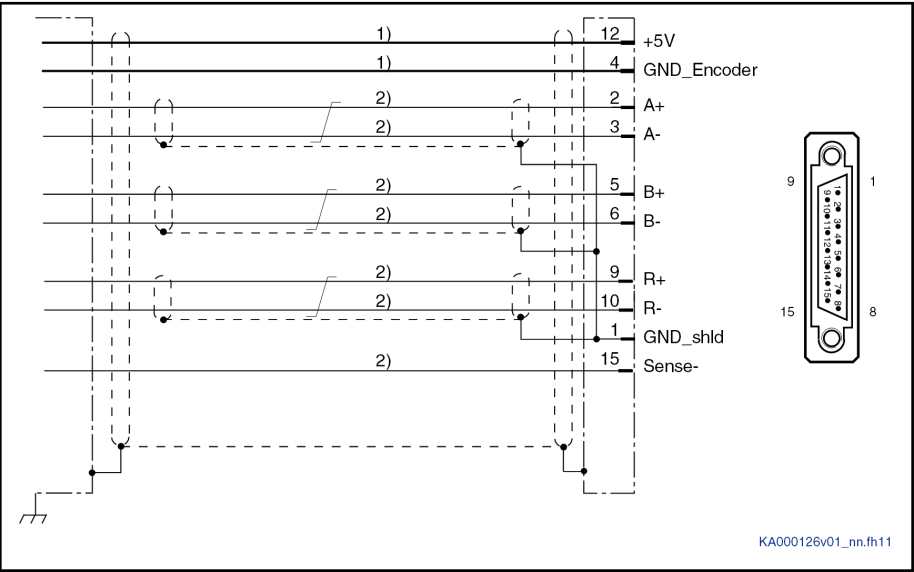
Connection Diagram
