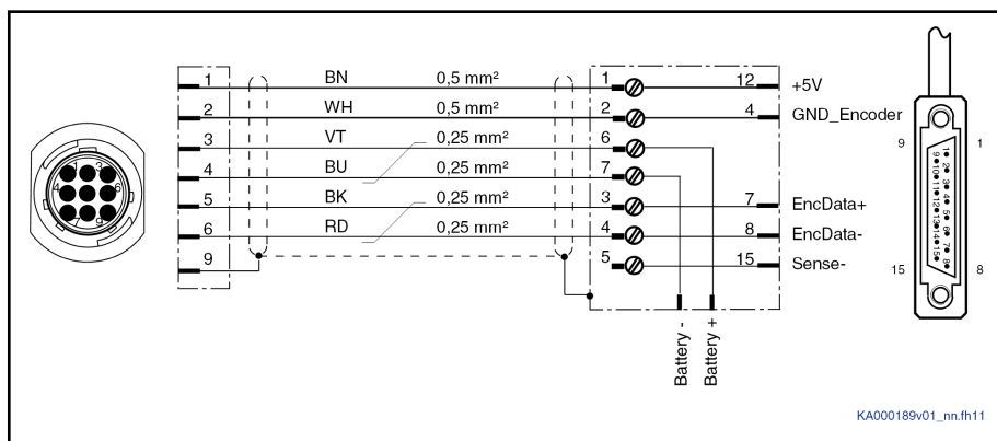
Fig. 8-21: Interconnection Diagram
