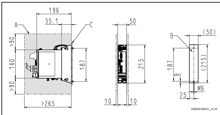
Fig. 4-4: Dimensional Drawing HCS01.1E-W0003/5/6/8/9/13 (Standard Mounting)
