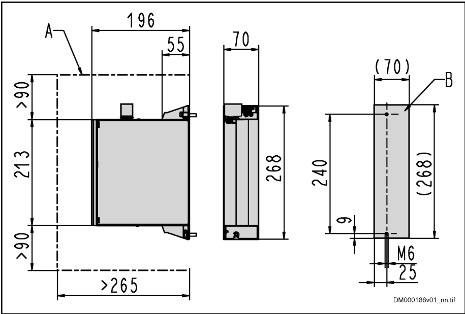
A Minimum mounting clearance B Boring Dimensions Fig.8-50: Dimensions
