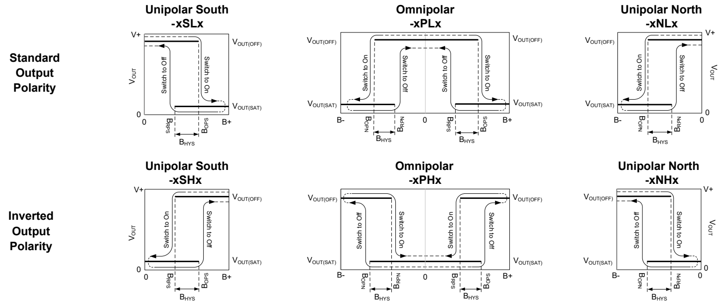
Figure 4: Hall Switch Output State vs. Magnetic Field
