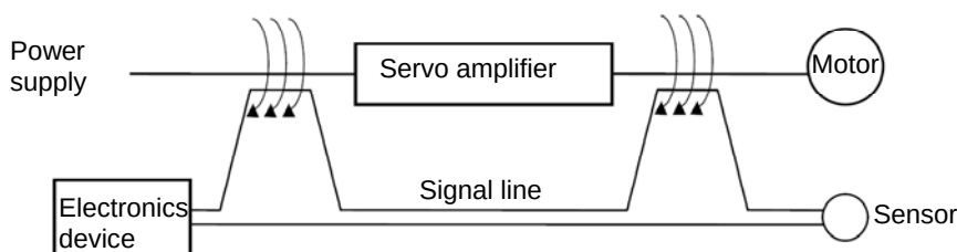
Fig. F2(2) Electromagnetically induced noise
