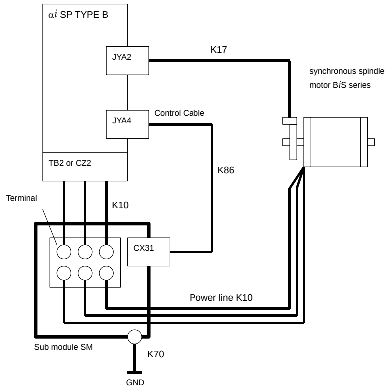
Overall connection
