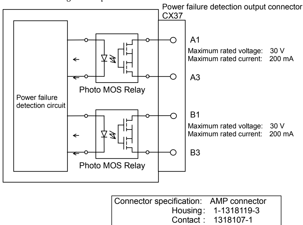
Fig. 1 Output circuit
