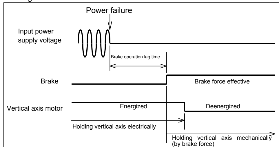
Timing chart
