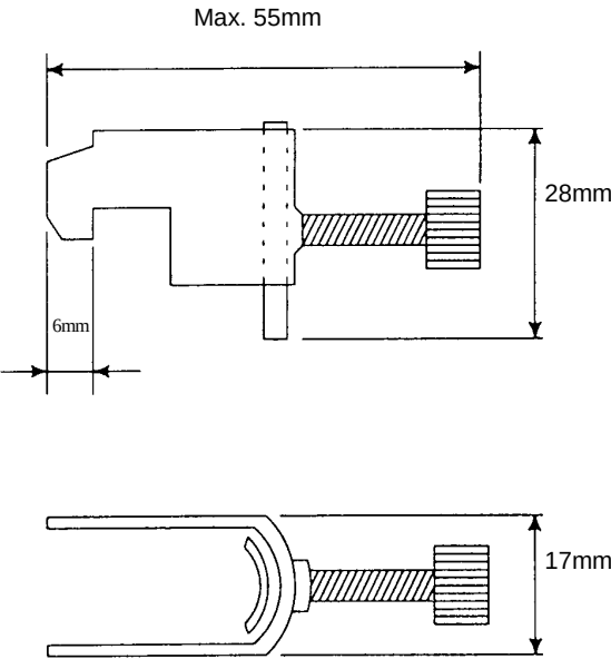
Fig.5.3.2(e) Outer drawings of metal fittings for clamp
