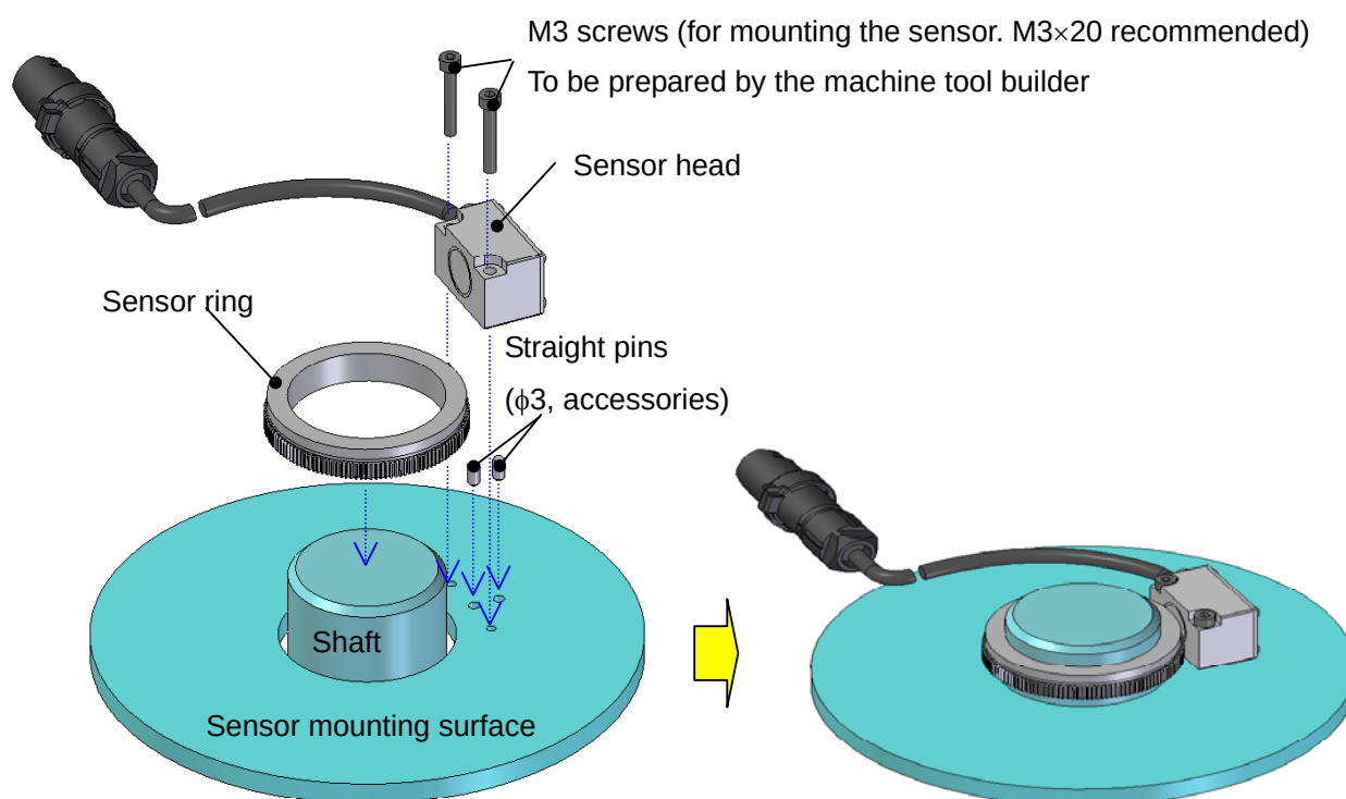
Fig. 2 After installation
