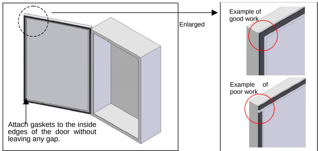
Fig. 6 Sealing doors
