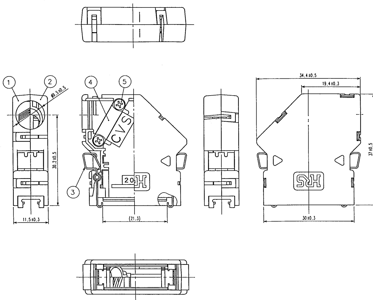
Fig.C(j) Connector housing (Side cable type)
