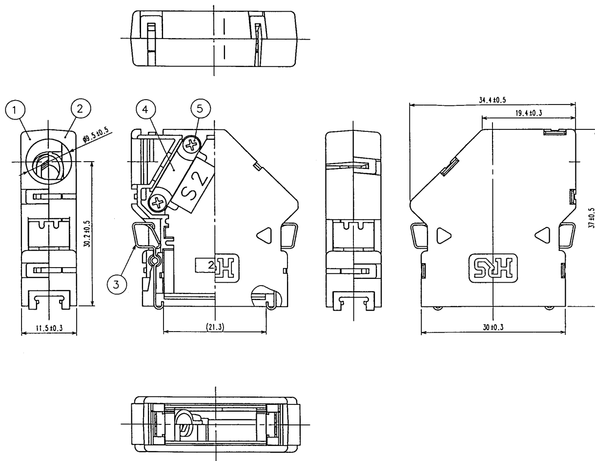
Fig.C(h) Connector housing (Side cable type)
