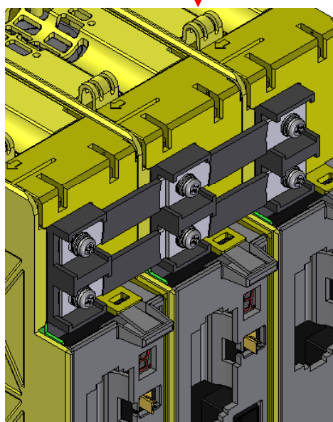
Before mounting
