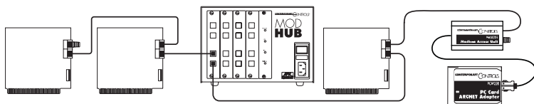
Figure 4—TB5 bus segments can be extended through active hubs.
