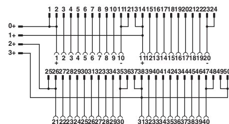
Connection scheme FLKM 50-PA-AB/OBN
