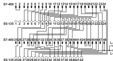
FLKM S135-465-4UA/T/S400 connection scheme
