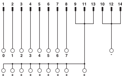
VIP-2/SC/FLK14/8P/PLC connection scheme
