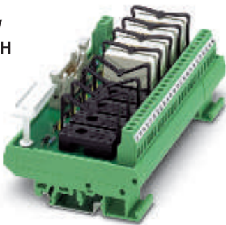
Output module with eight miniature relays, 1 PDT
