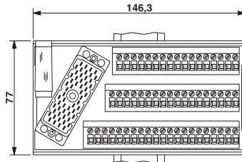
Dimensional drawing for UMK-EC56/32-XOL
