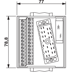
Dimensional drawing for UMK-EC56/25/EX-R
