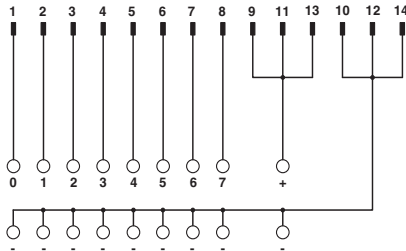
VIP-2/SC/FLK14/8M/PLC connection scheme
