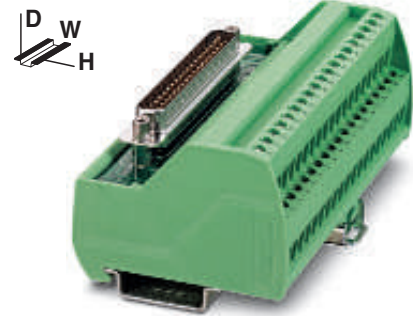
37 poles with screw connection
