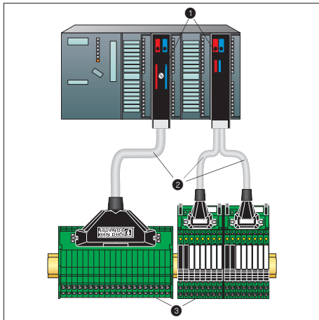
Figure 2: Example of control cabinet wiring with front adapters 1, pre-assembled system cables 2, and termination boards 3
