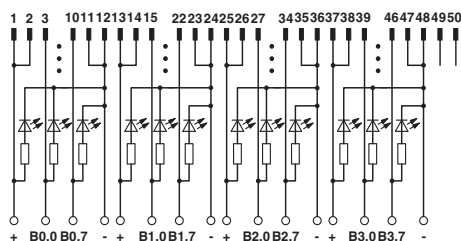
UM 45-FLK50/LA/ZFKDS/PLC connection scheme
