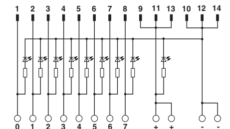
UM 45-2FLK14/ZFKDS/S7 connection scheme
