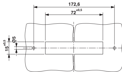
Dimensioning of the housing cutout
