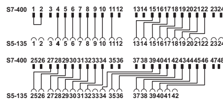
FLKM S135-431-UA/S400 connection scheme
