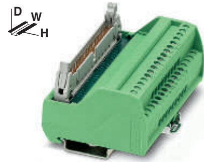
VARIOFACE controller board for 16 channels
