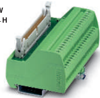
Passive interface modules for input/output of 32 channels
