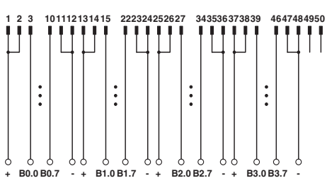
UM 45-FLK14/ZFKDS/PLC connection scheme
