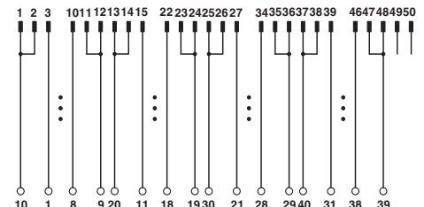
VIP-2/SC/FLK50/MODI-TSX/Q connection scheme
