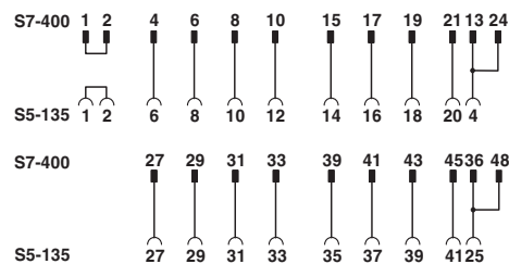
Connection scheme: FLKM S135/S400/SO123
