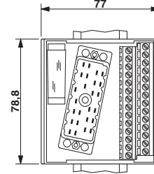
Dimensional drawing for UMK-EC56/25/EX-L
