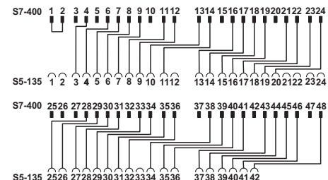
FLKM S135-465-4UA/UI/S400 connection scheme
