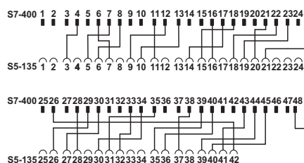
Connection scheme FLKM S135-470-4UC//S400
