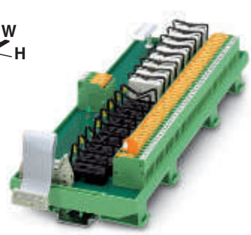
Output extension module for 16 miniature relays with knife/disconnect terminal blocks, 1 PDT
