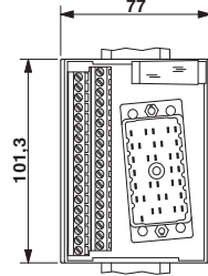
Dimensional drawing for UMK-EC90/32/EX-XUR
