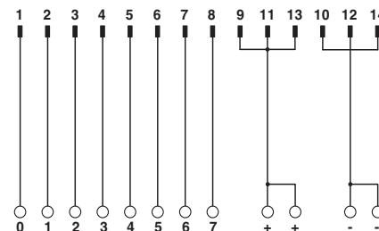
UM 45-FLK14/ZFKDS/PLC connection scheme
