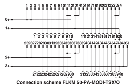
Connection scheme FLKM 50-PA-MODI-TSX/Q
