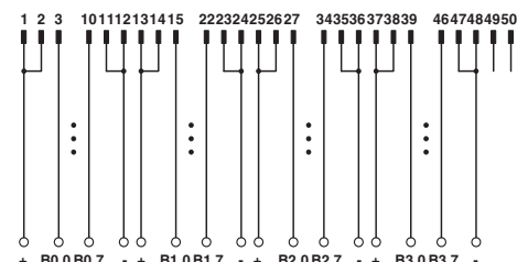
VIP-2/SC/FLK50/PLC connection scheme
