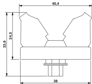
Dimensional drawing DFLK-D62 SUBH/S
