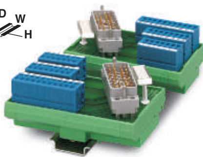
25-pos., with front connection terminal blocks
