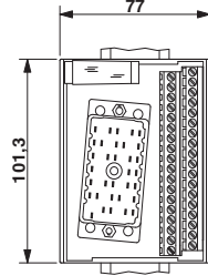
Dimensional drawing for UMK-EC90/32/EX-XUL
