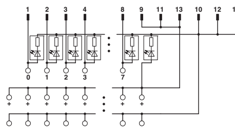
VIP-3/SC/FLK14/8IM/PLC connection scheme
