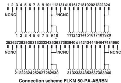
Connection scheme FLKM 50-PA-AB/IBN
