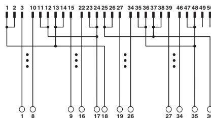
VIP-2/SC/FLK50/AB-1756 connection scheme
