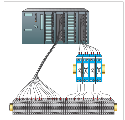
Figure 1: Example of control cabinet cabling with individual signal lines
