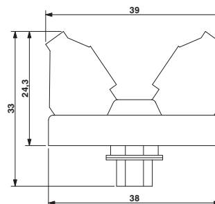
Dimensional drawing: DFLK-D...SUB:
