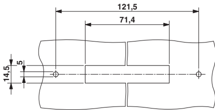
Dimensioning of the housing cutout
