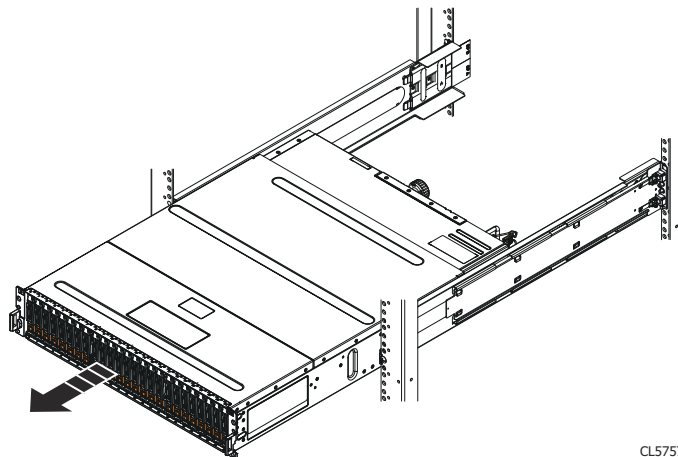
Figure 5. Sliding the enclosure out of the cabinet
