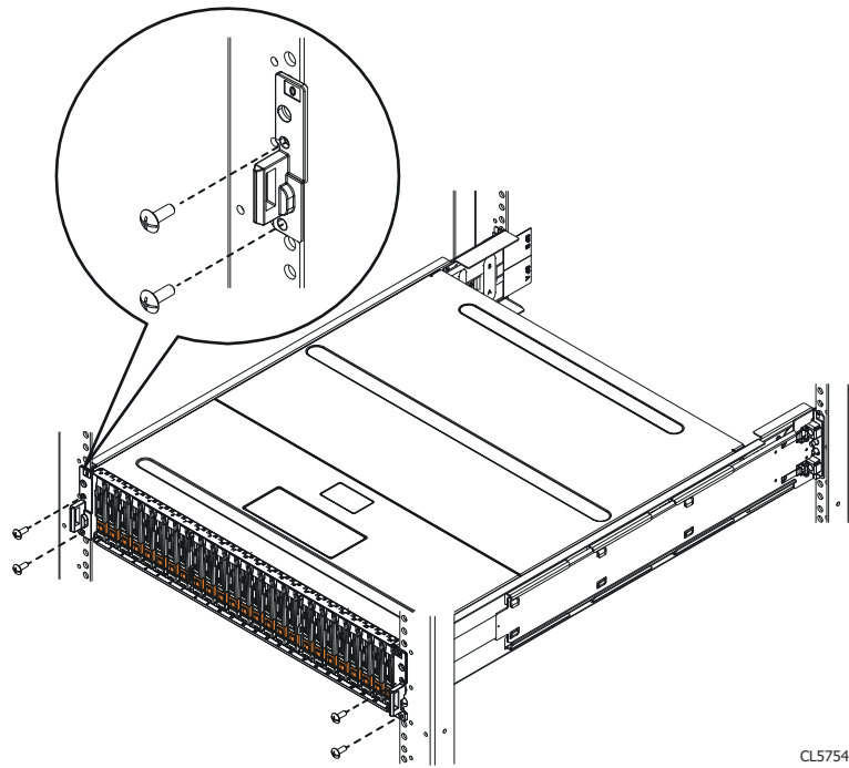
Figure 4. Removing the screws that secure the enclosure to the front of the cabinet
