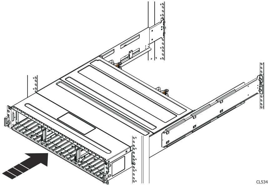
Figure 6. Sliding the enclosure onto the rails
