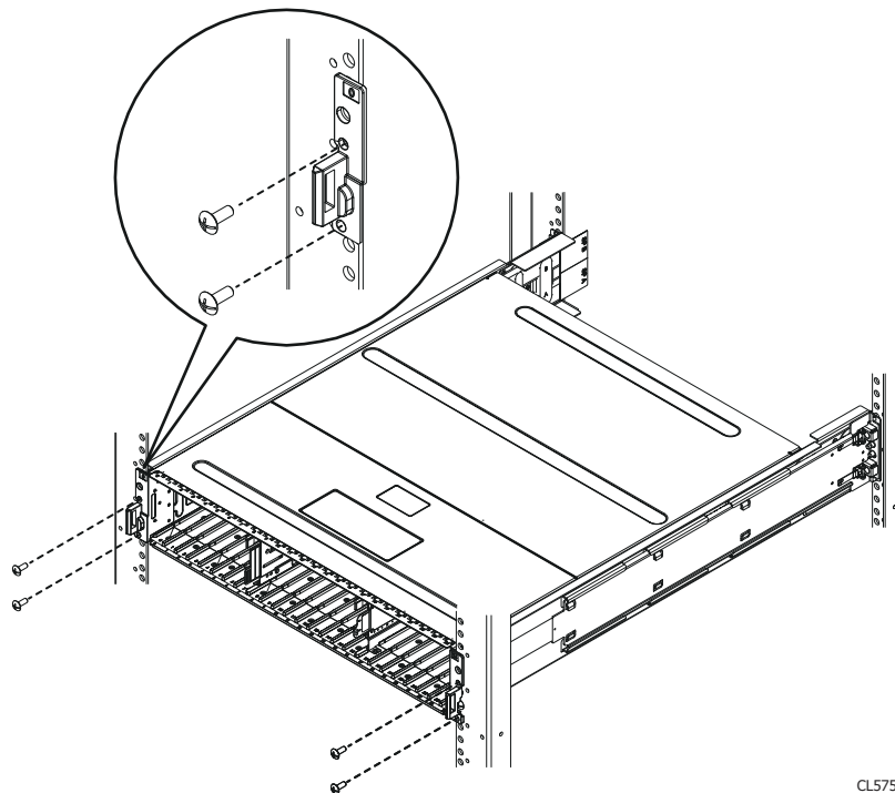
Figure 7. Securing enclosure to the front of the cabinet
