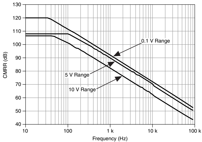
Figure 1. AI <0..31> CMRR
