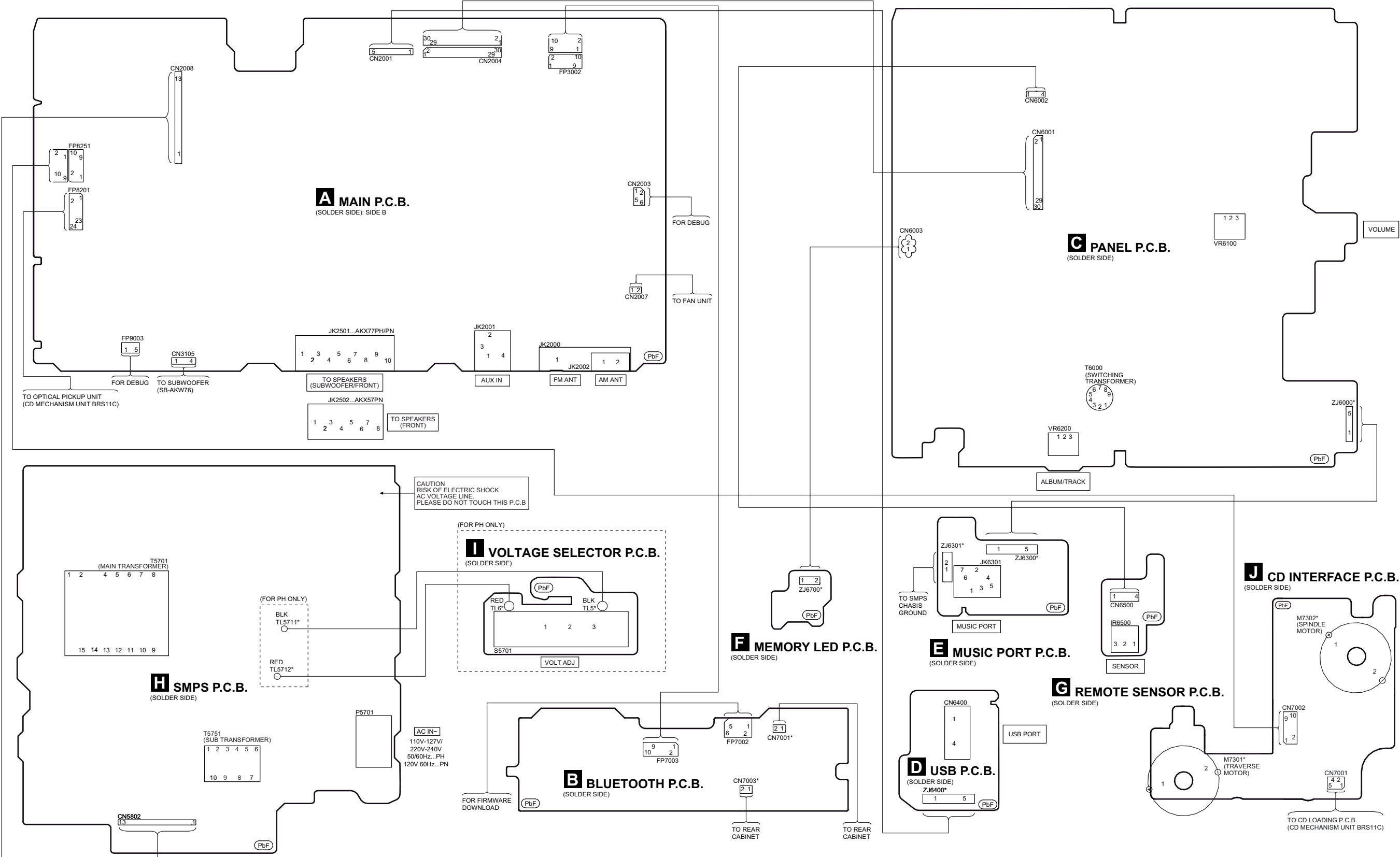
SA-AKX57PN, SA-AKX77PH/PN WIRING CONNECTION DIAGRAM
