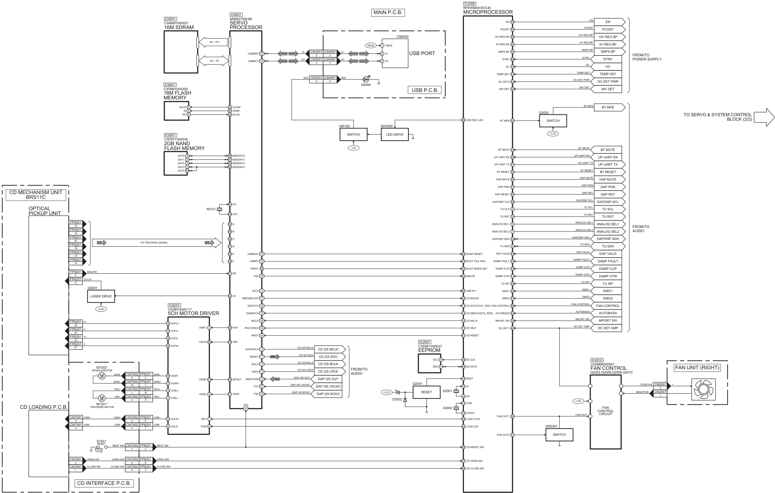
SA-AKX57PN,SA-AKX77PH/PN SERVO & SYSTEM CONTROL (1/2) BLOCK DIAGRAM
